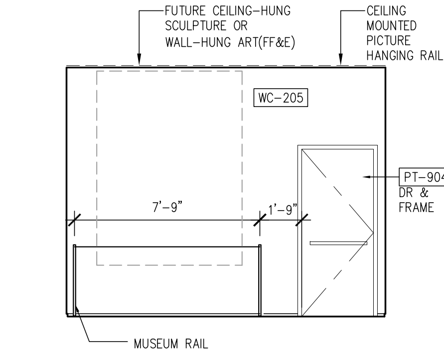
4 | PREFUNCTION AND GALLERY - S. ELEV. 1/4" = 1'-0"
