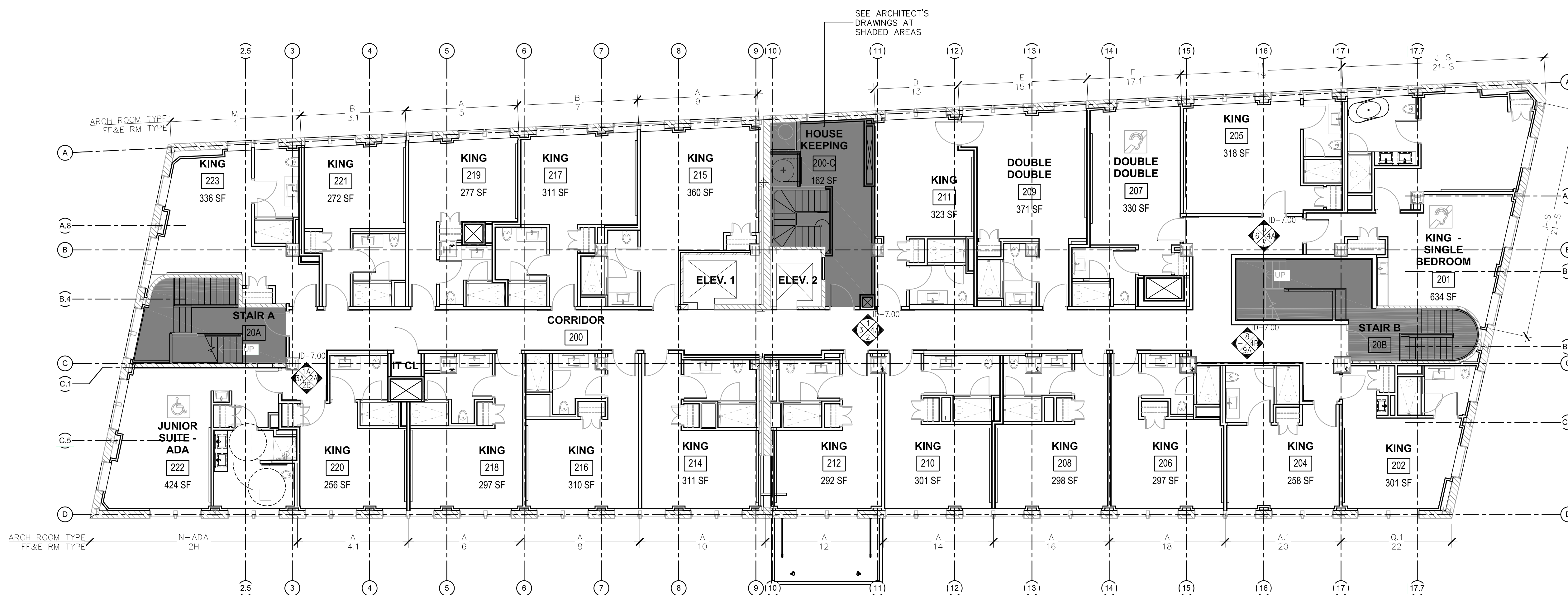
1 2ND FLOOR - PLAN 1/8" = 1'-0"
