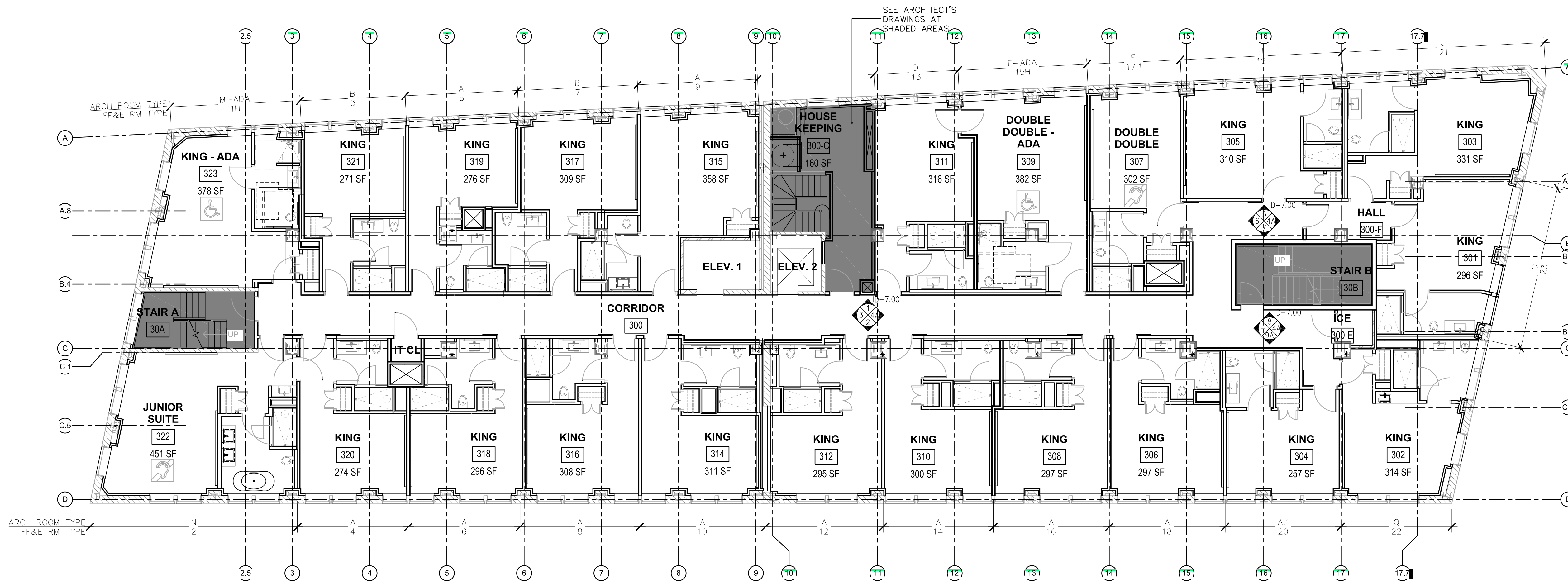
2 3RD FLOOR - PLAN 1/8" = 1'-0"
