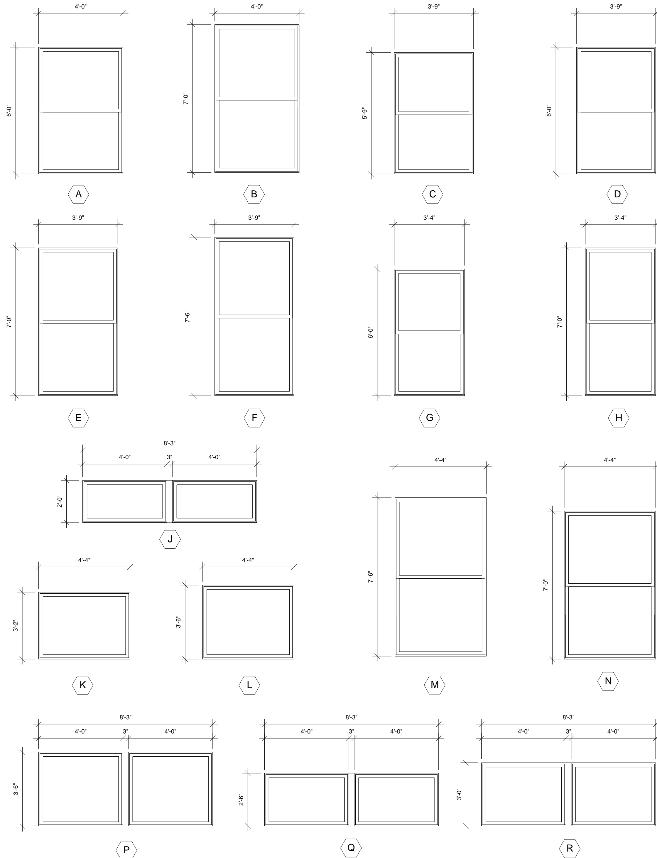
NEW WINDOW ELEVATIONS
