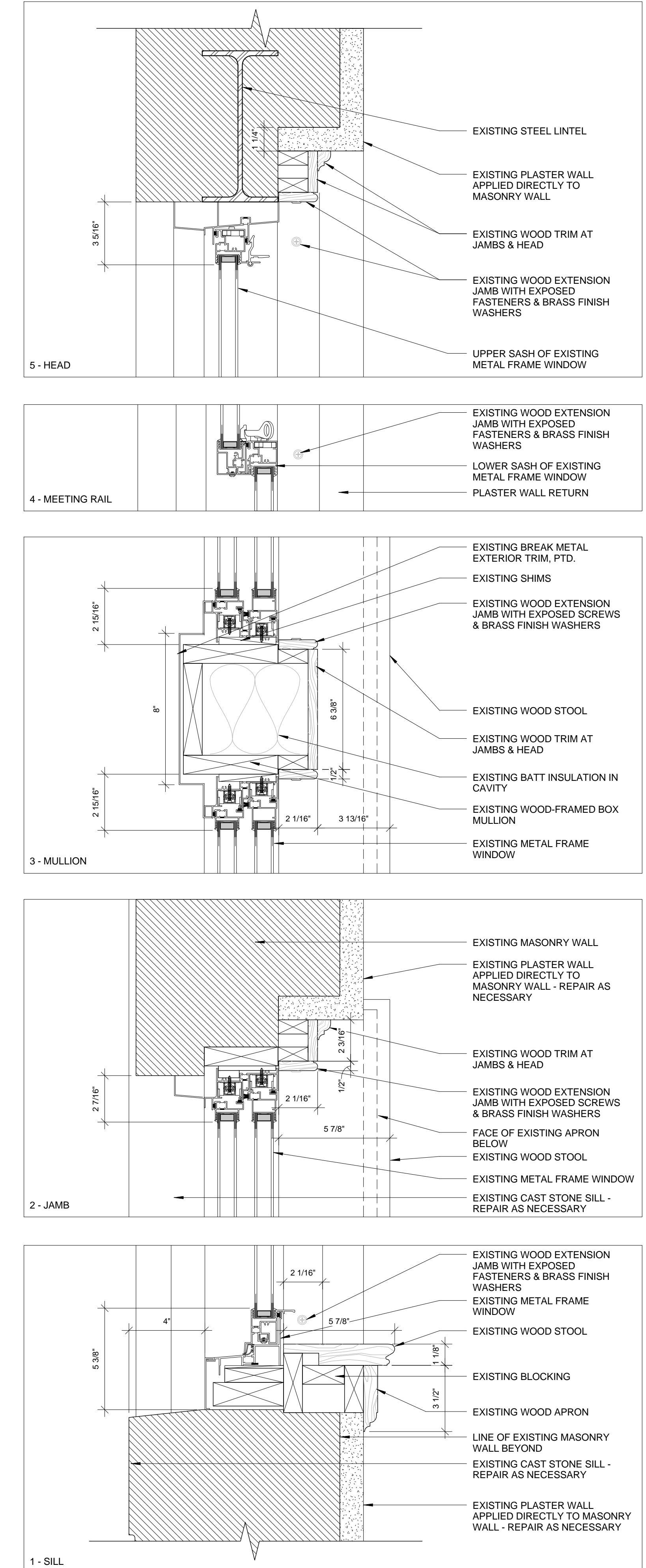
1 EXISTING WINDOW & TRIM DETAILS
