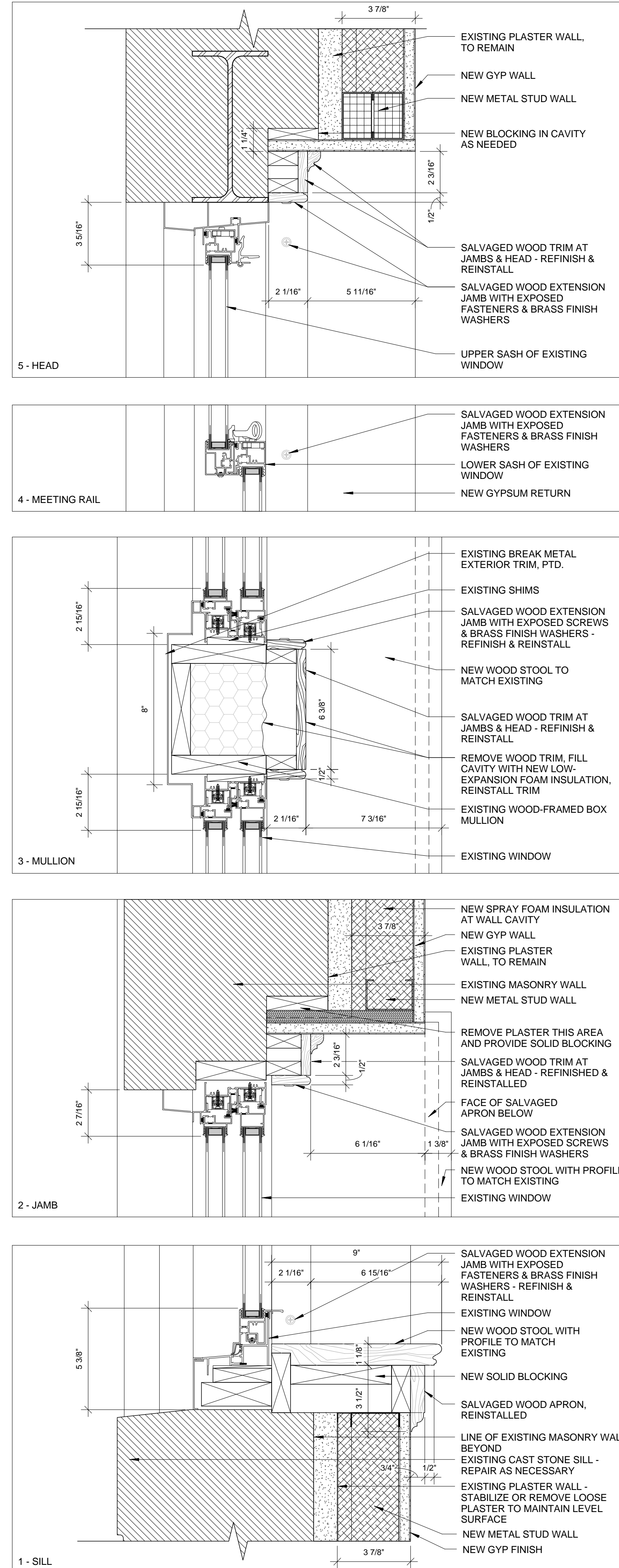
2 EXISTING WINDOW DETAILS WITH NEW FURRING WALL & TRIM
