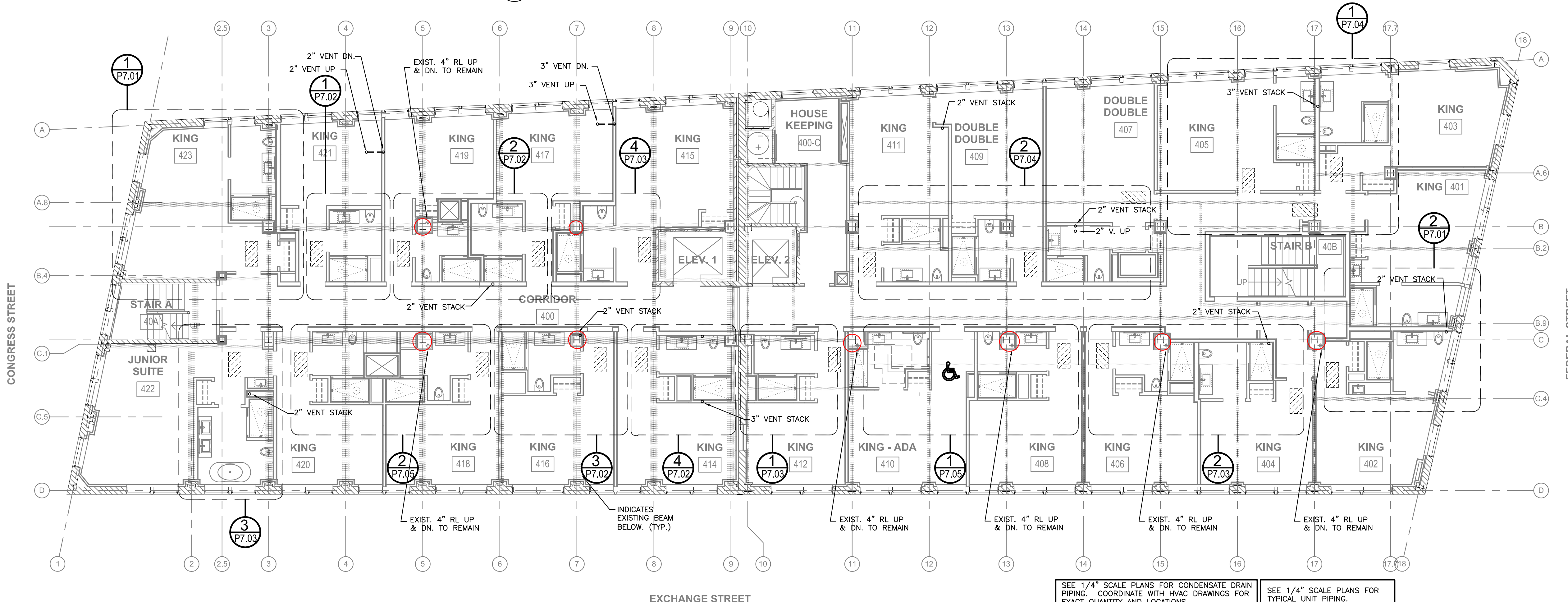
1 | FOURTH FLOOR PLAN - WATER SCALE: 1/8"=1'-0"
