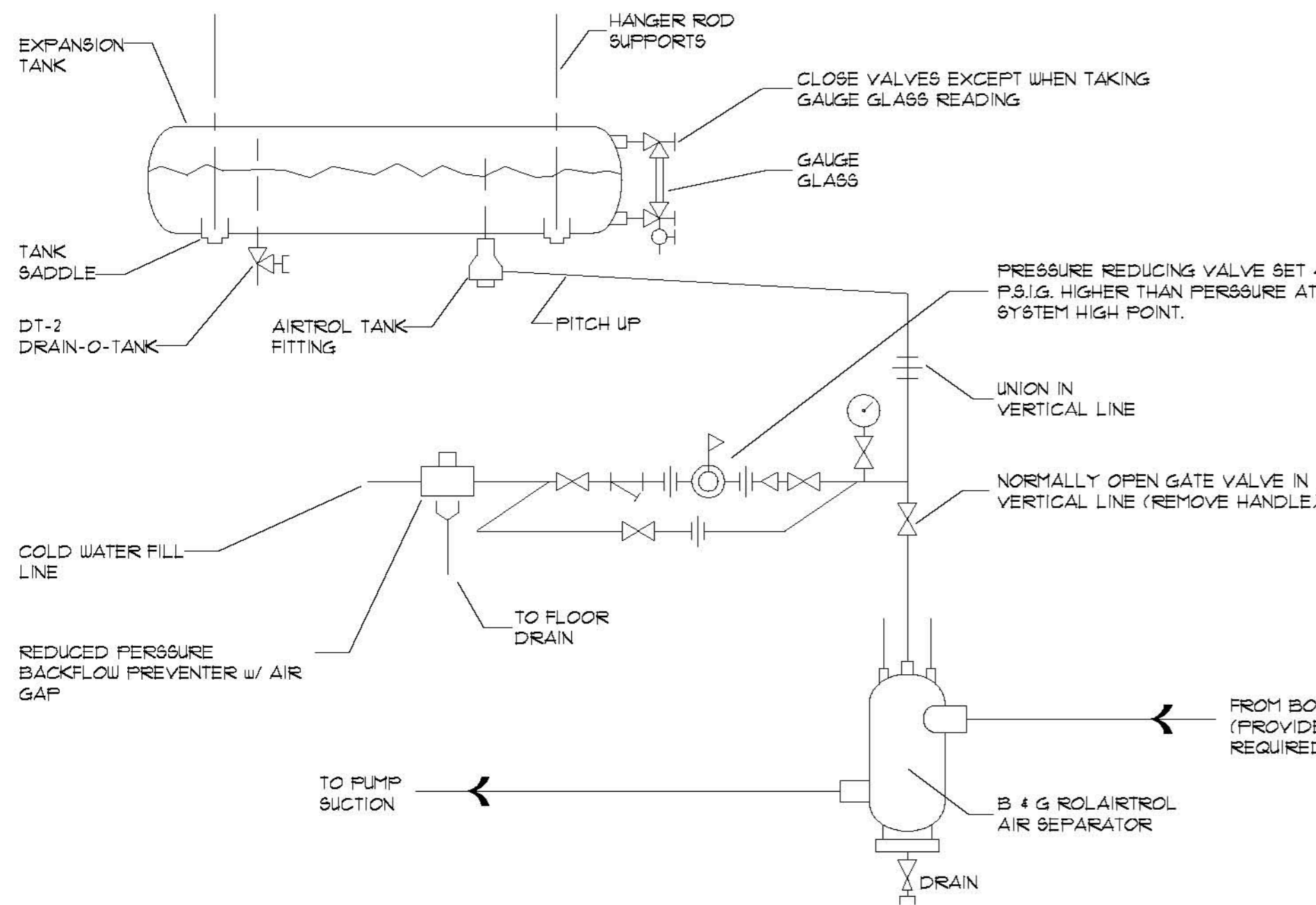
TYPICAL EXPANSION TANK CONNECTIONS DETAIL NO SCALE
