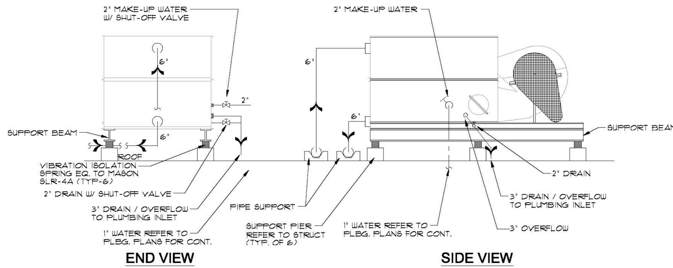
HEAT EXCHANGER DETAIL NO SCALE
