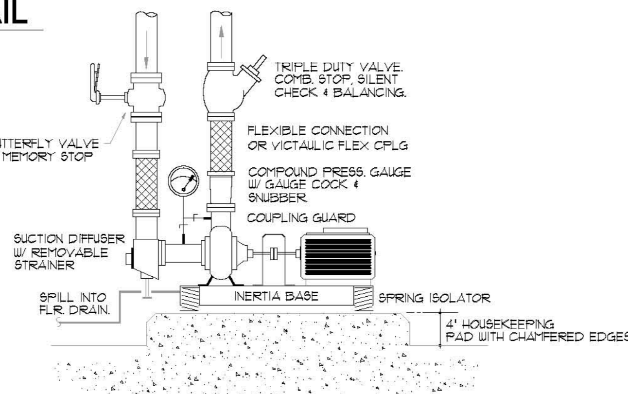
BASE MOUNTED PUMP DETAIL NO SCALE
