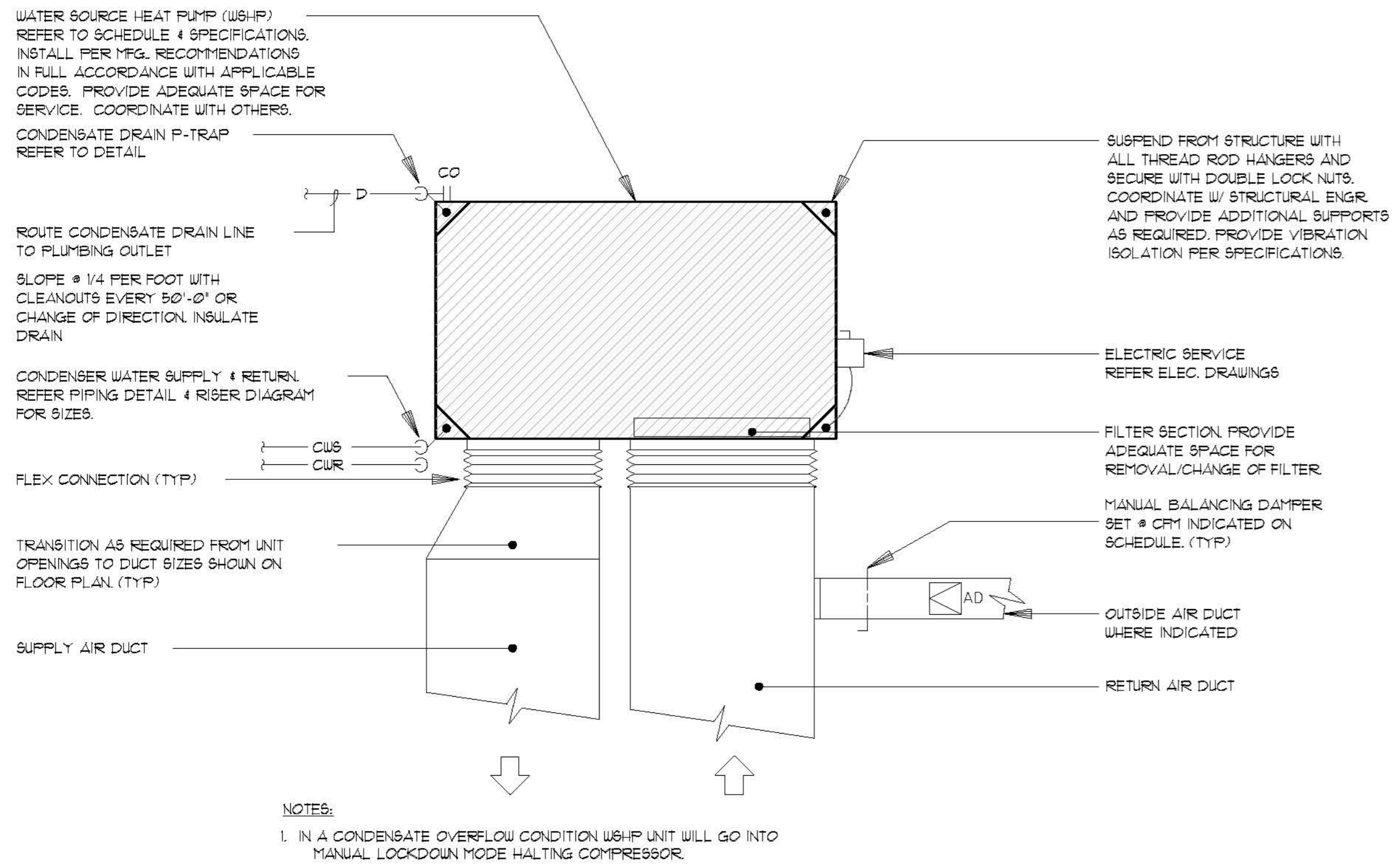
WATER SOURCE HEAT PUMP UNIT - HORIZONTAL NO SCALE
