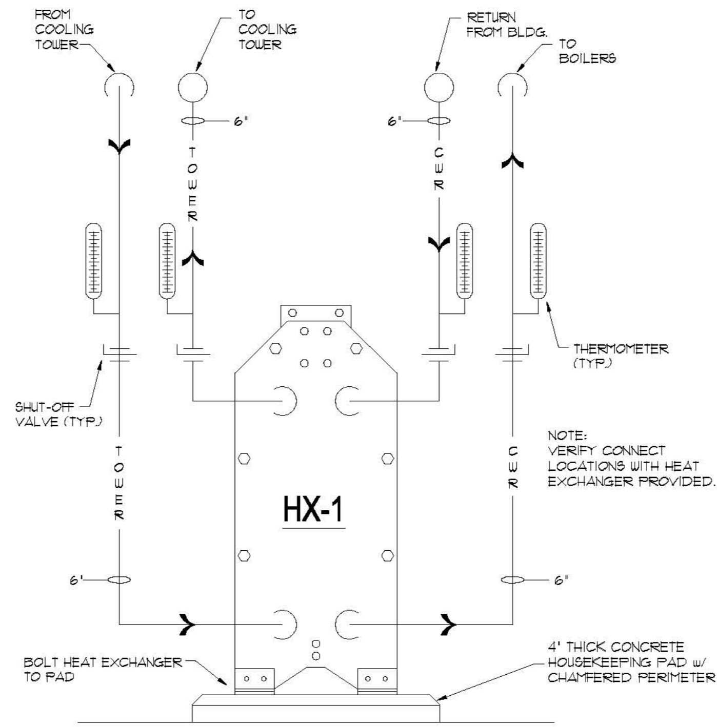
HEAT EXCHANGER DETAIL NO SCALE
