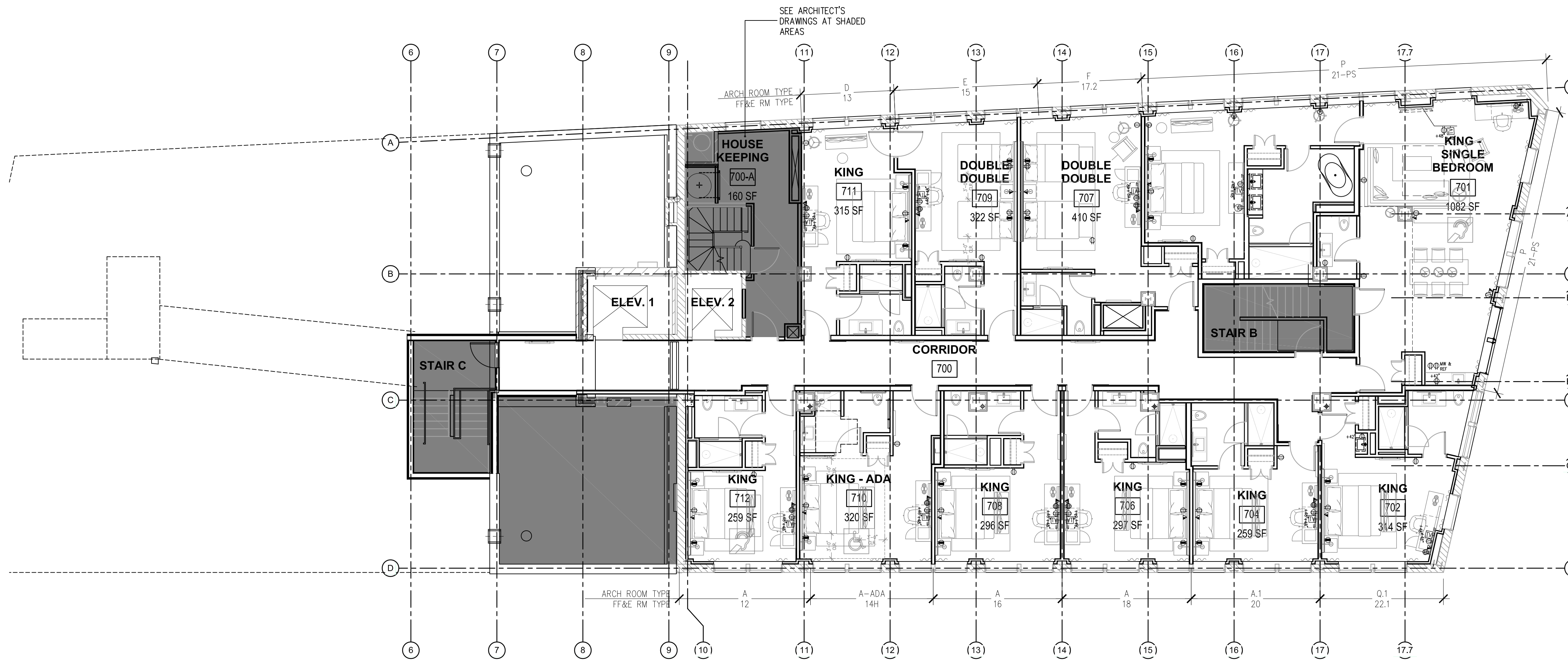
2 7TH FLOOR - FURNITURE PLAN 1/8" = 1'-0"
