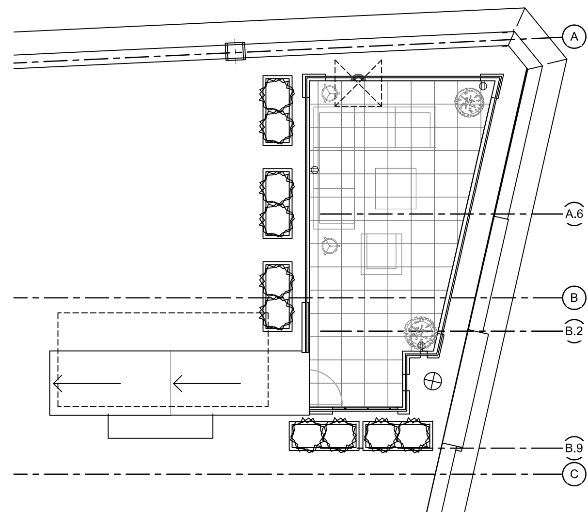
3 ROOF DECK - FURNITURE PLAN 1/8" = 1'-0"
