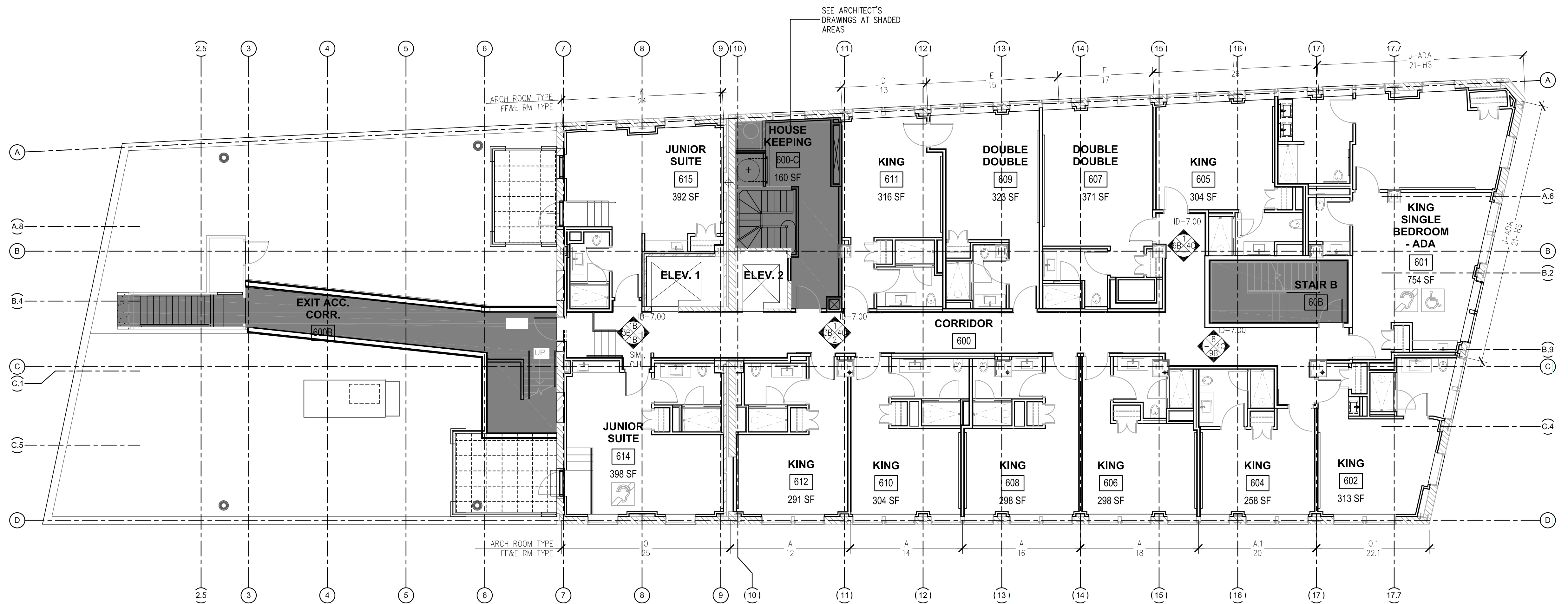
1 | 6TH FLOOR - PLAN 1/8" = 1'-0"
