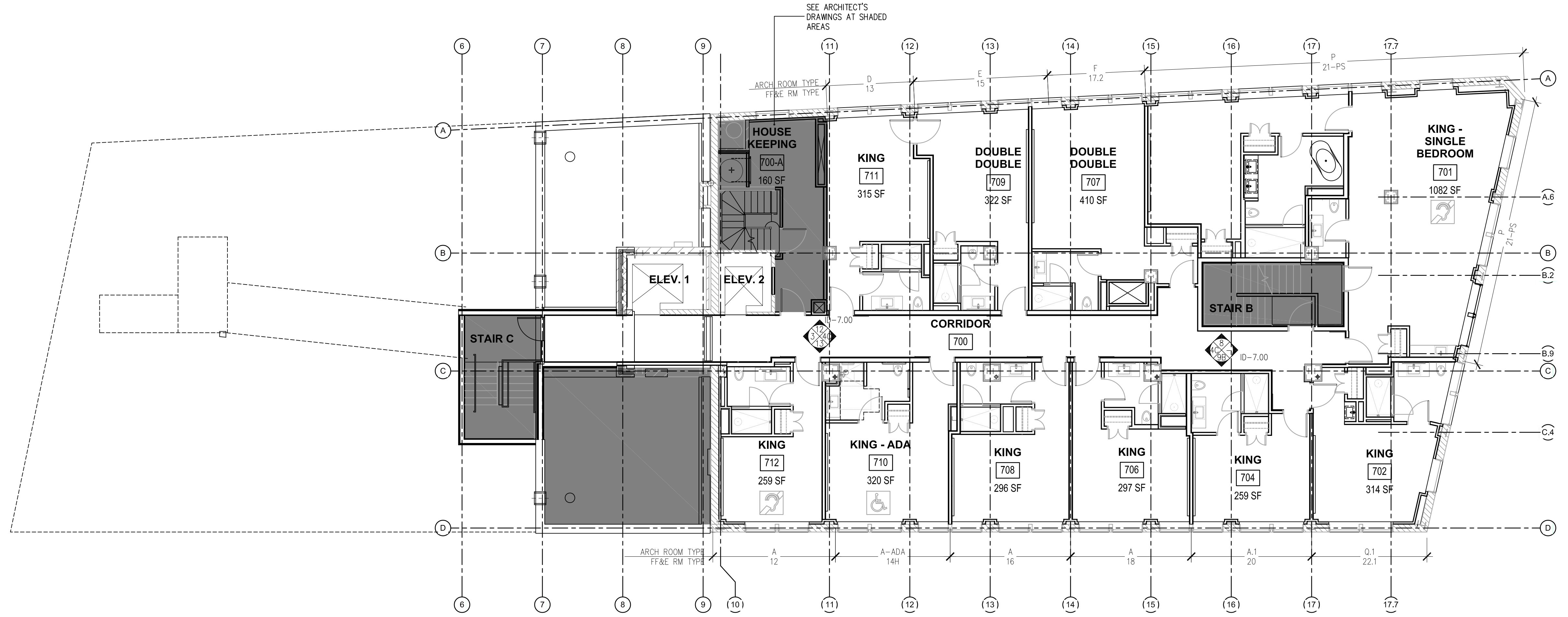
2 | 7TH FLOOR - PLAN 1/8" = 1'-0"
