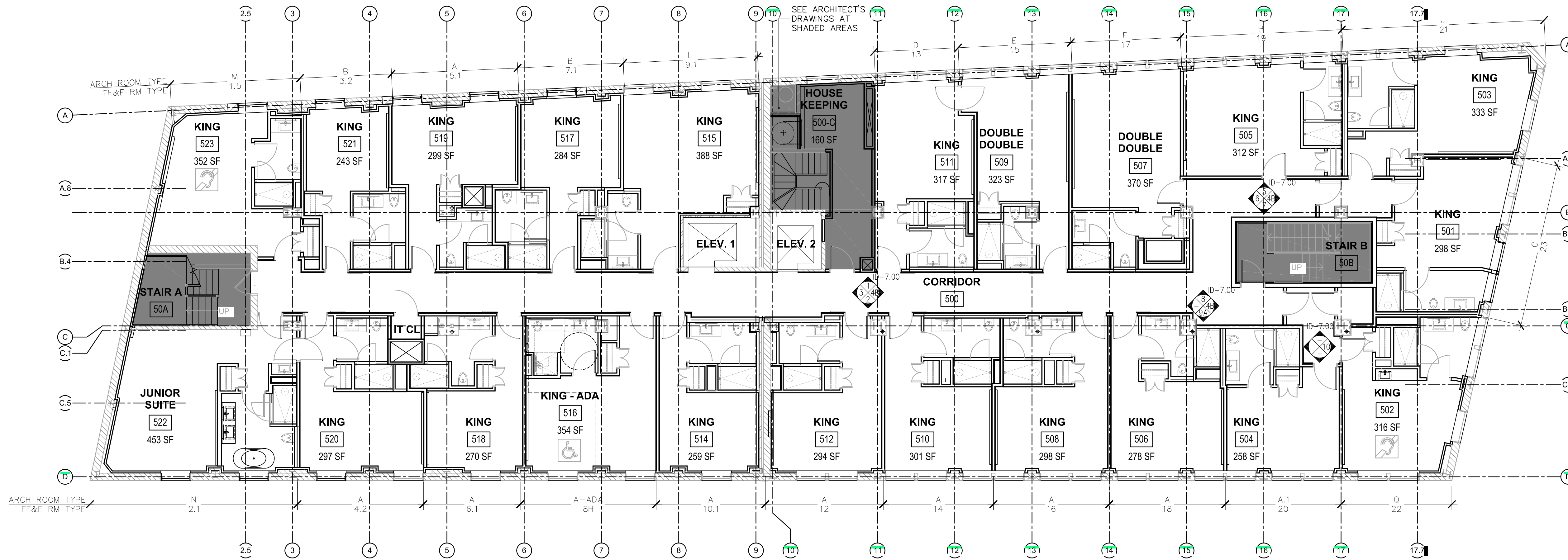
2 | 5TH FLOOR - PLAN 1/8" = 1'-0"
