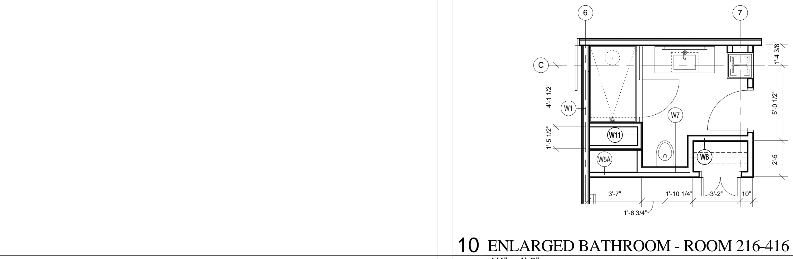
10 ENLARGED BATHROOM - ROOM 216-416 1/4" = 1'-0"
