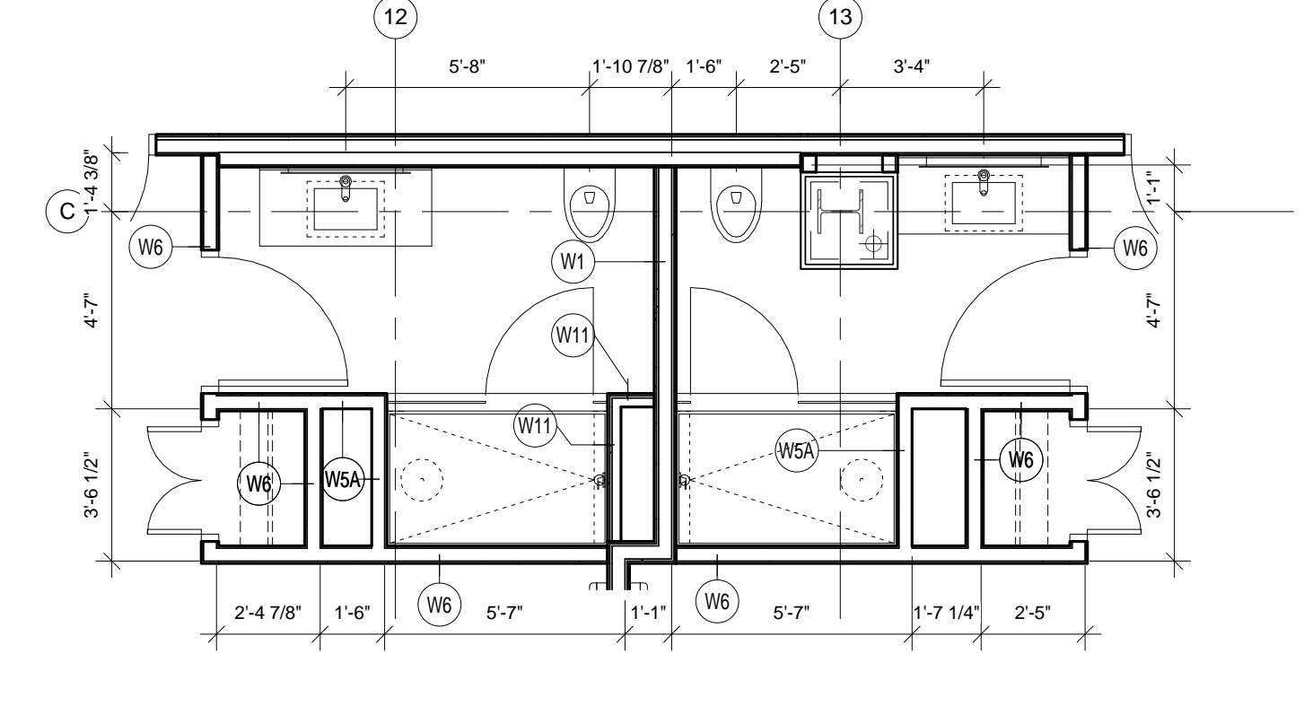
5 ENLARGED BATHROOM - ROOM 208-708 & 210, 310, 510 - 710 1/4" = 1'-0"
