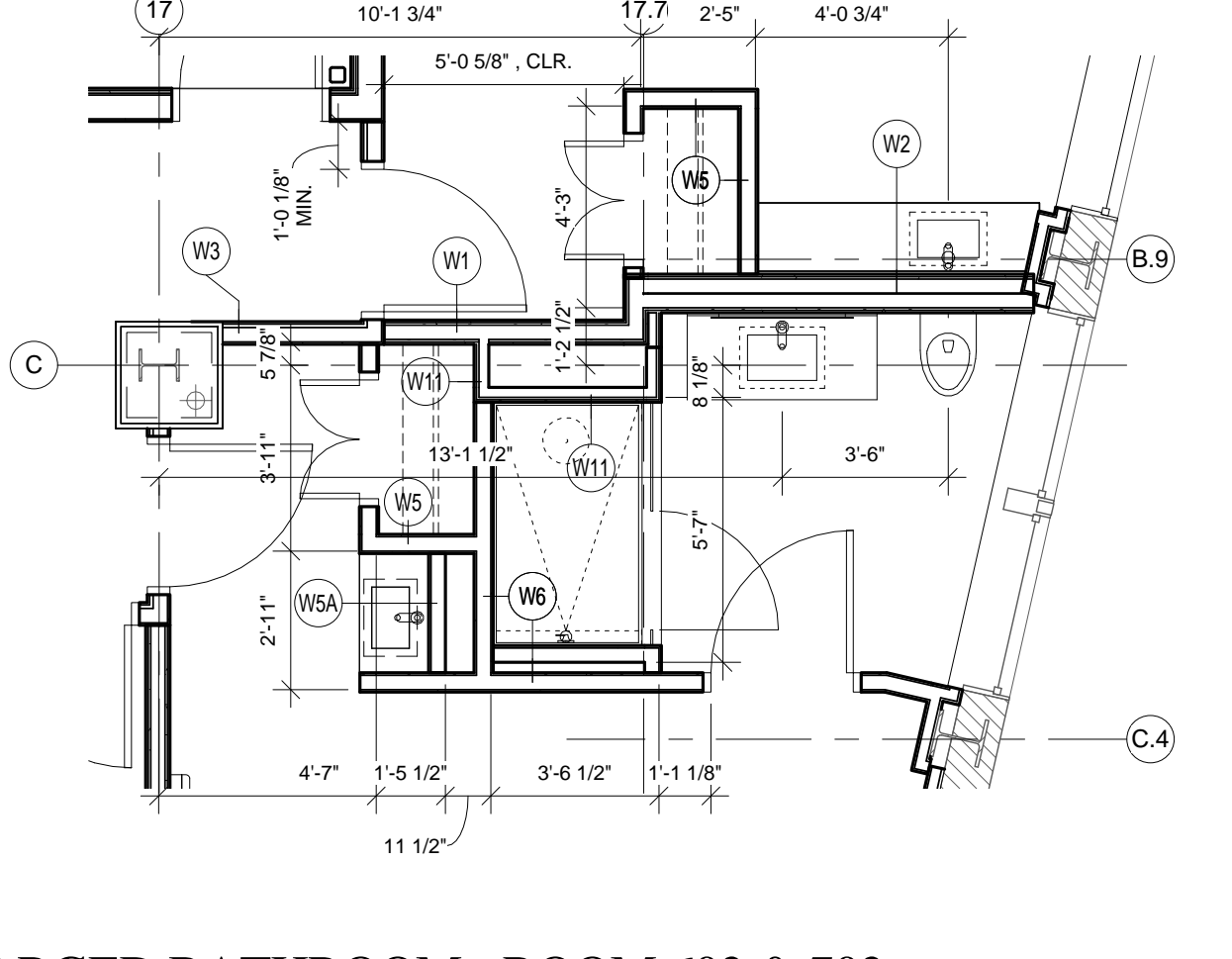
3 ENLARGED BATHROOM - ROOM 602 & 702 1/4" = 1'-0"
