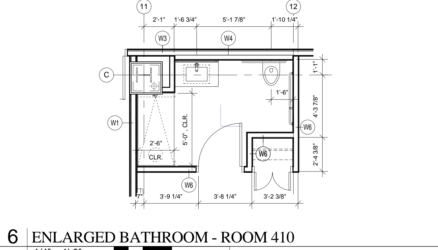
6 ENLARGED BATHROOM - ROOM 410 1/4" = 1'-0"
