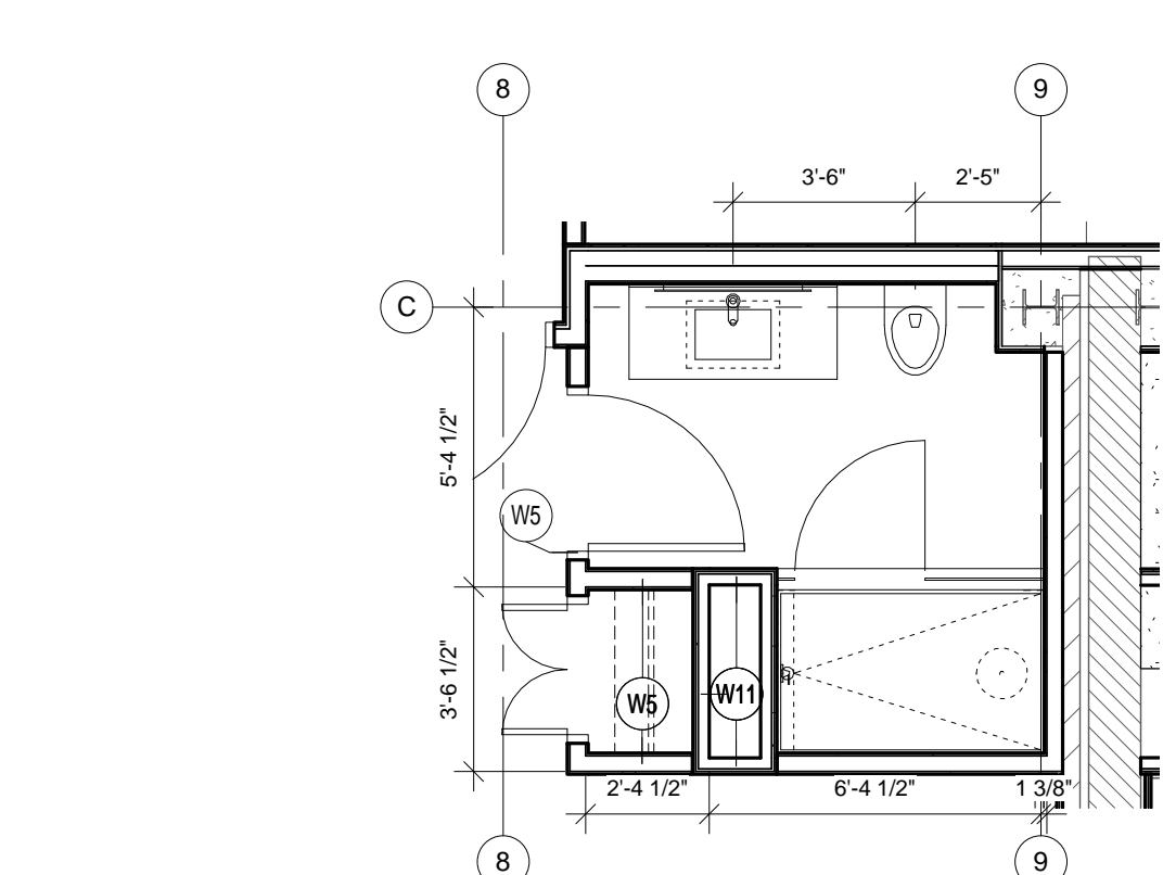
9 ENLARGED BATHROOM - ROOM 714 1/4" = 1'-0"
