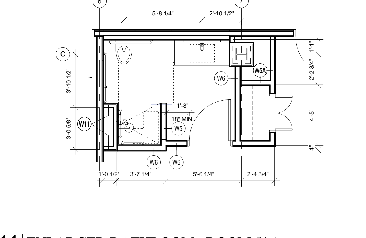
11 ENLARGED BATHROOM - ROOM 516 1/4" = 1'-0"
