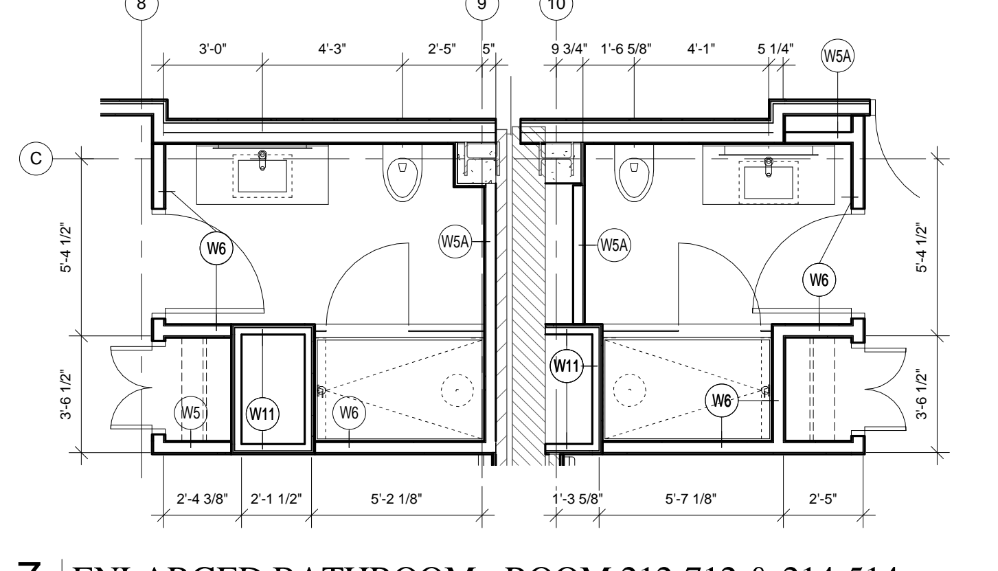
7 ENLARGED BATHROOM - ROOM 212-712 & 214-514 1/4" = 1'-0"
