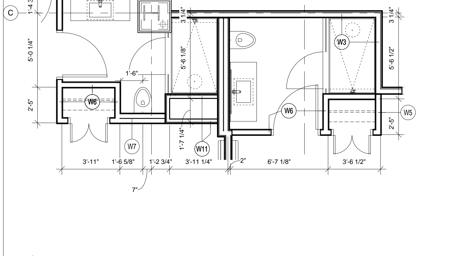
4 ENLARGED BATHROOM - ROOM 204 & 206 - 704 & 706 1/4" = 1'-0"
