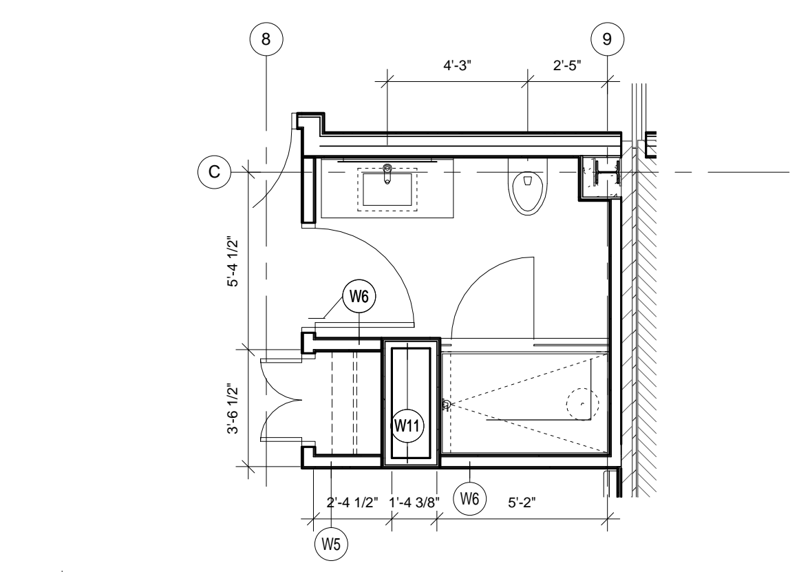
8 ENLARGED BATHROOM - ROOM 614 1/4" = 1'-0"
