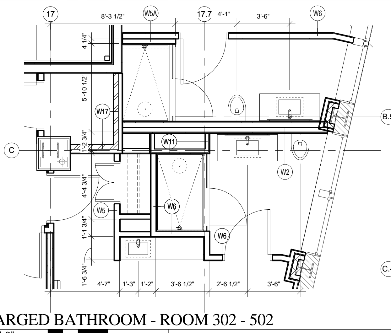
2 ENLARGED BATHROOM - ROOM 302 - 502 1/4" = 1'-0"
