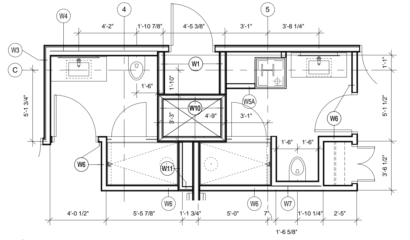
12 ENLARGED BATHROOM - ROOM 218 & 220 1/4" = 1'-0"
