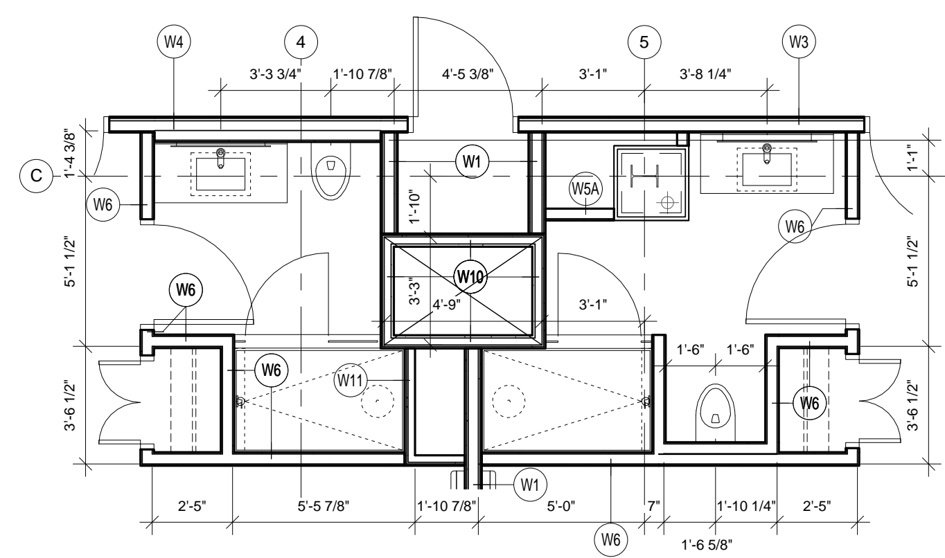
13 ENLARGED BATHROOM - ROOM 318-518 & 320-520 1/4" = 1'-0"
