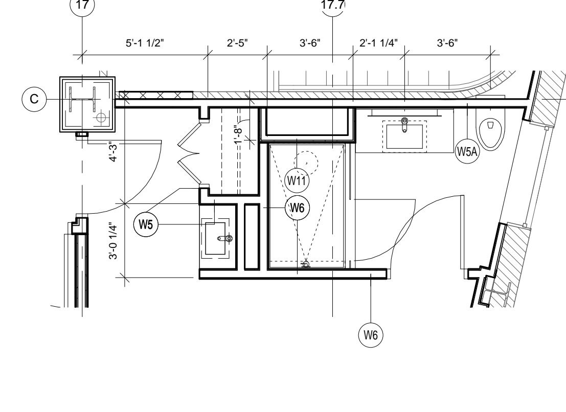
1 ENLARGED BATHROOM - ROOM 202 1/4" = 1'-0"
