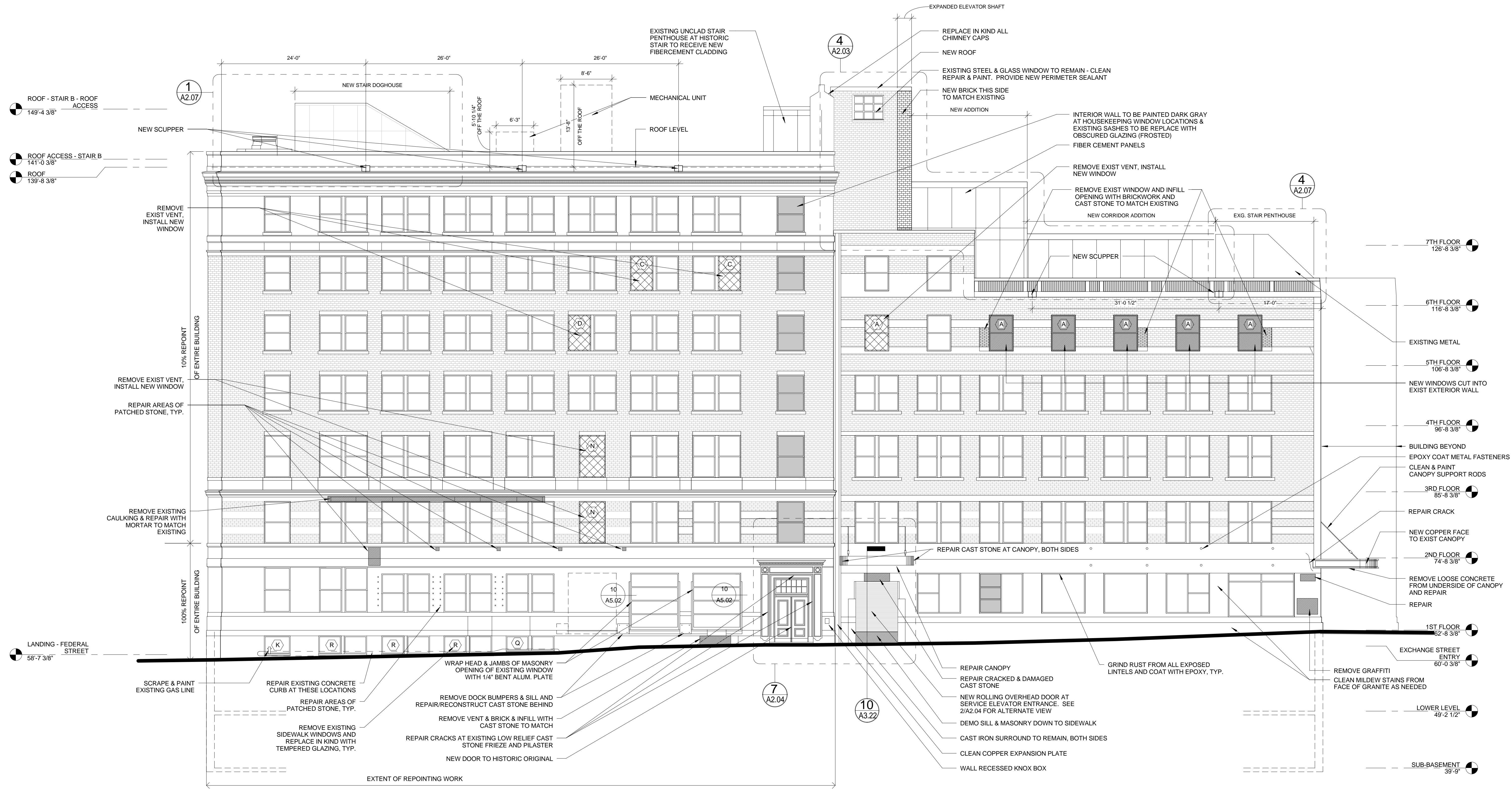
1 EAST ELEVATION - MARKET STREET ELEVATION 1/8" = 1'-0"
