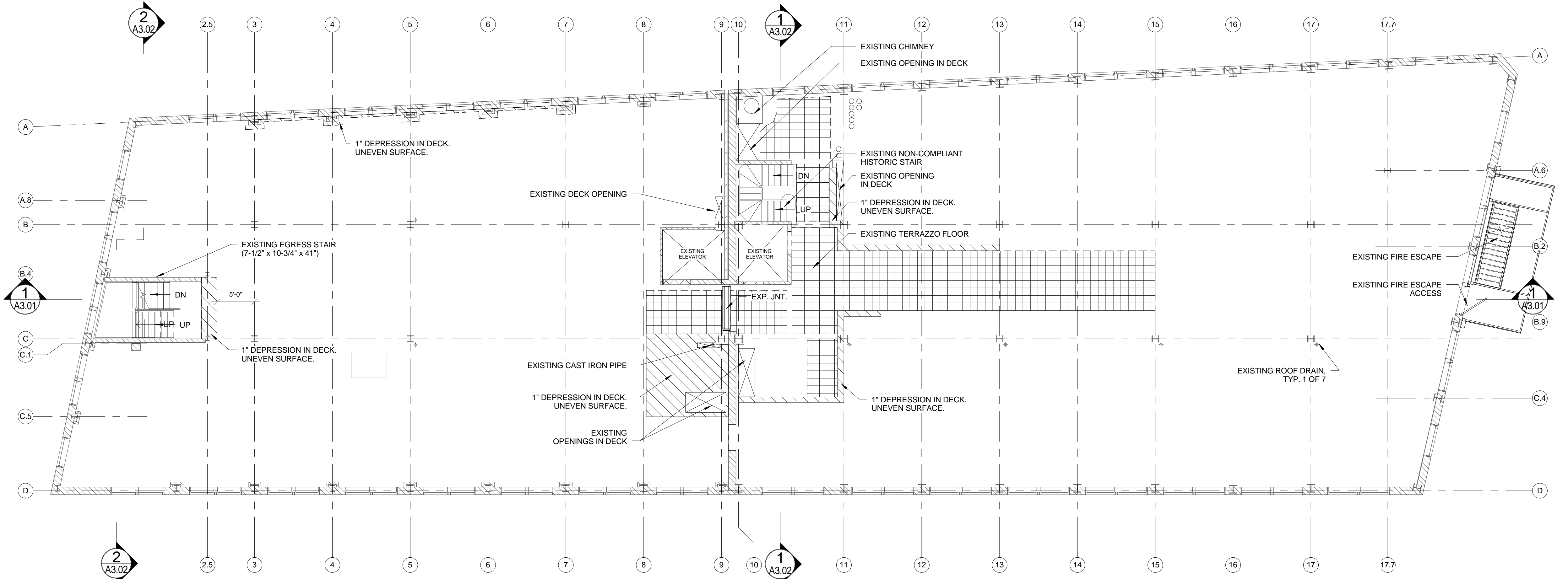
1 FOURTH FLOOR - EXISTING CONDITIONS 1/8" = 1'-0"
