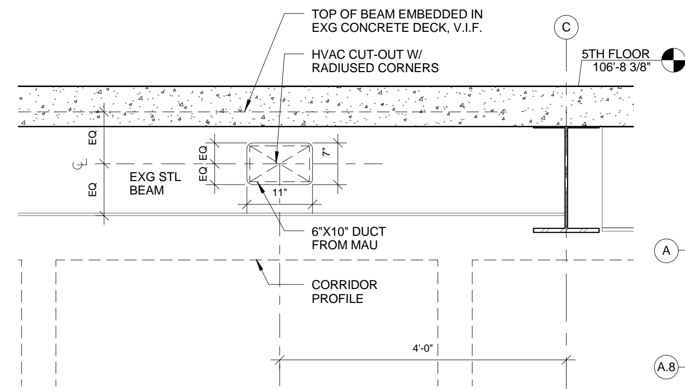
3 BEAM DEMO DTL @ 5TH FL. DECK (4TH FL. HALL) 3/4" = 1'-0"
