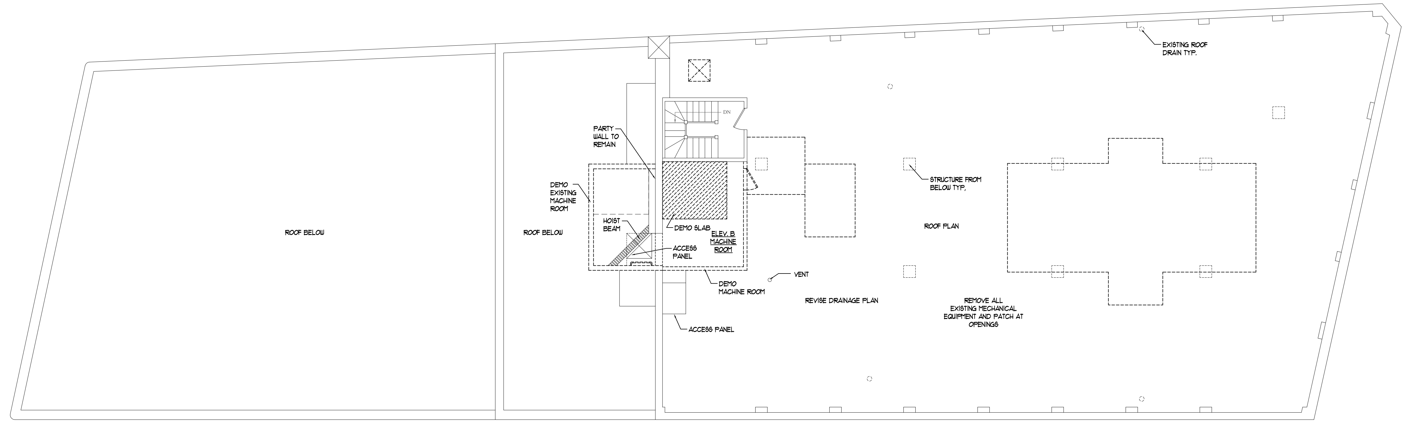
8 | MACHINE ROOM B/ROOF DEMO PLAN SCALE: 1/8"=1'-0"
