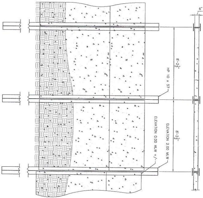
SCOUR PROTECTION - ELEVATION VIEW 1/2" = 1'
