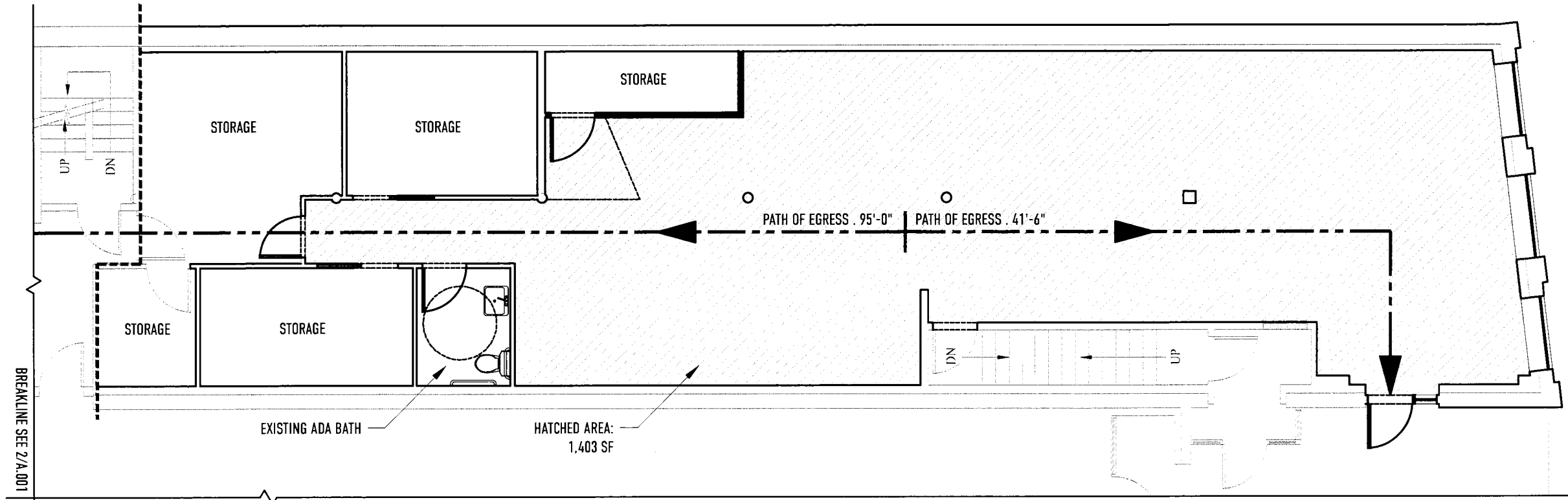
1 PARTIAL LIFE SAFETY PLAN 1/8"=1'-0"
