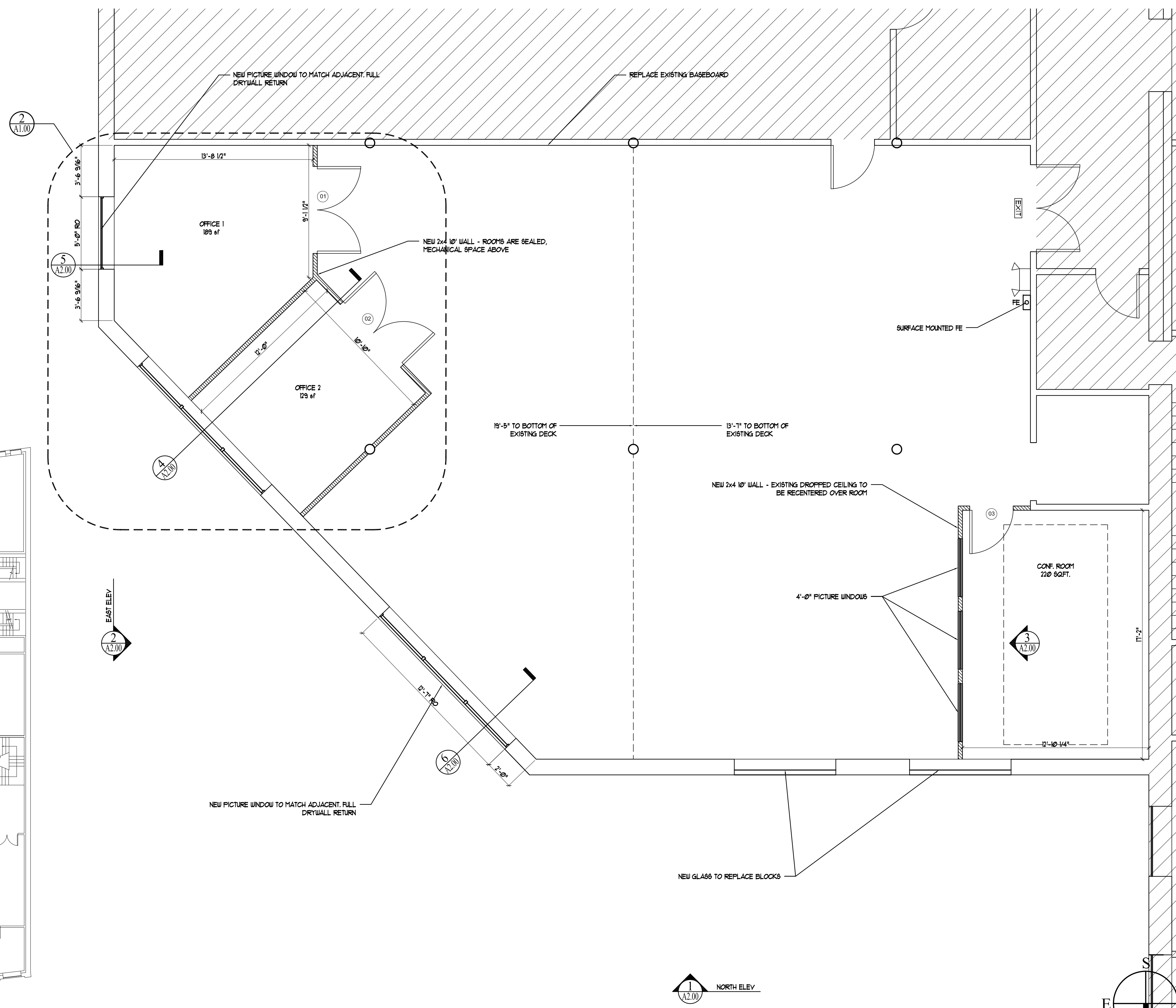
1 | FLOOR PLAN SCALE: 1/4"=1'-0"
