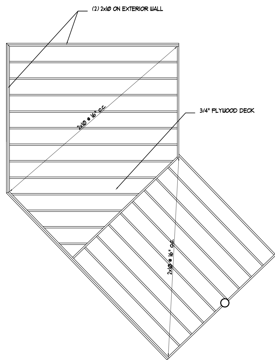
2 | FRAMING PLAN SCALE: 1/4"=1'-0"
