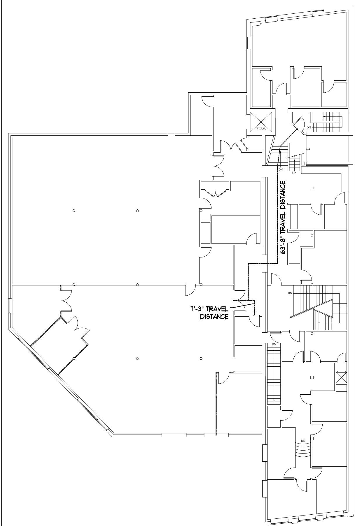
4 | SECOND FLOOR EGRESS PLAN SCALE: 1/16"=1'-0"
