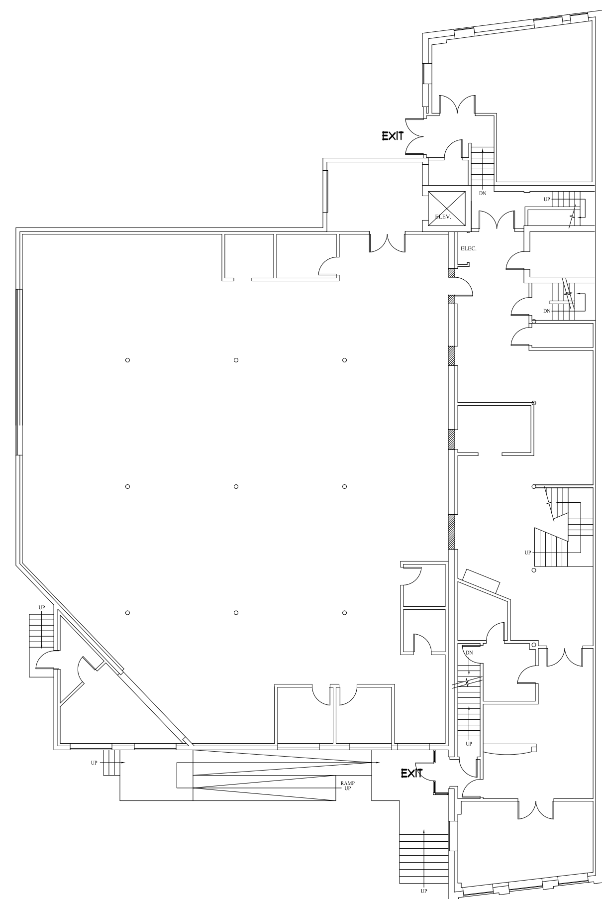
3 | FIRST FLOOR EGRESS PLAN SCALE: 1/16"=1'-0"
