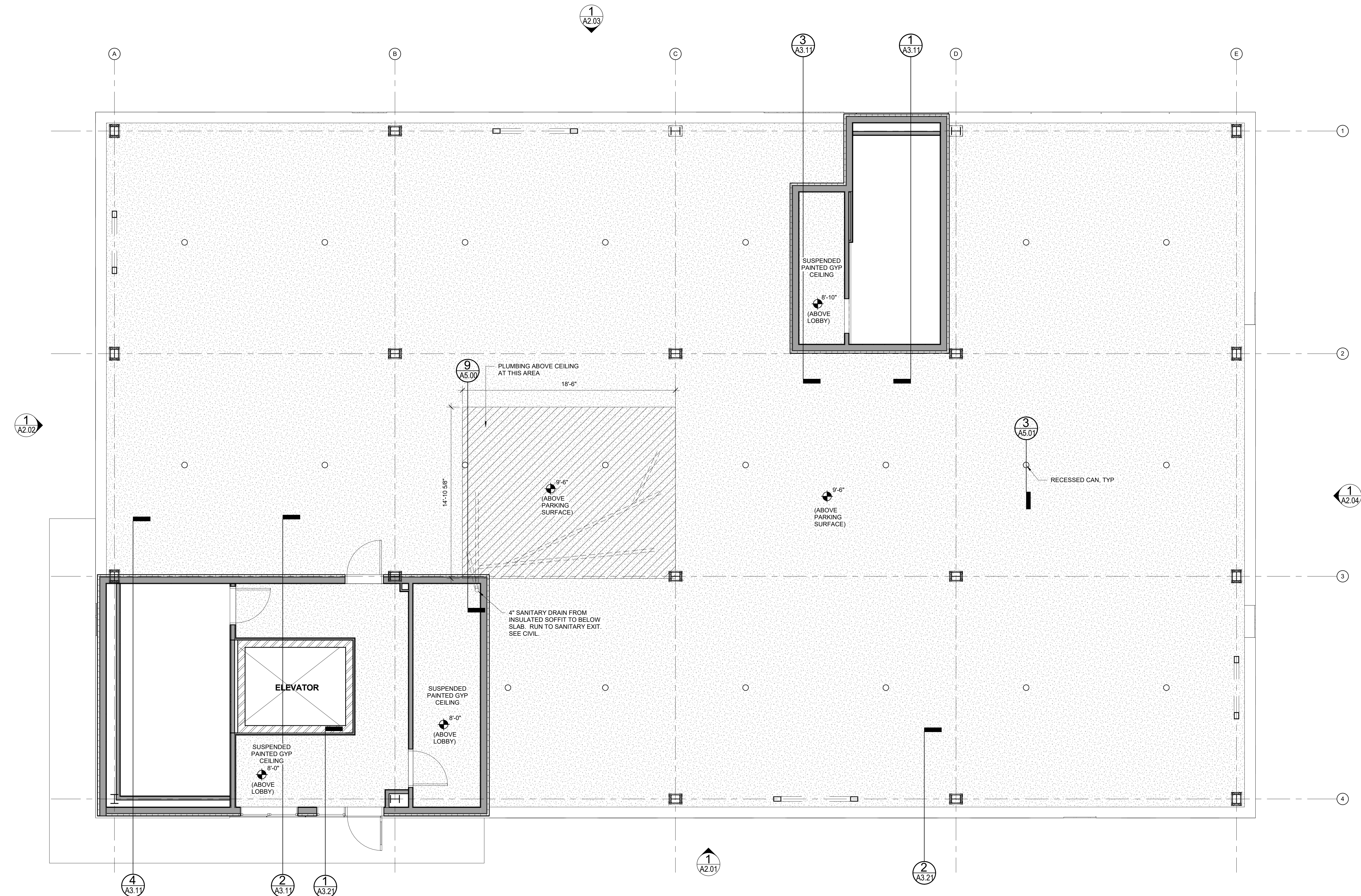
1 LOBBY 1/4" = 1'-0"
