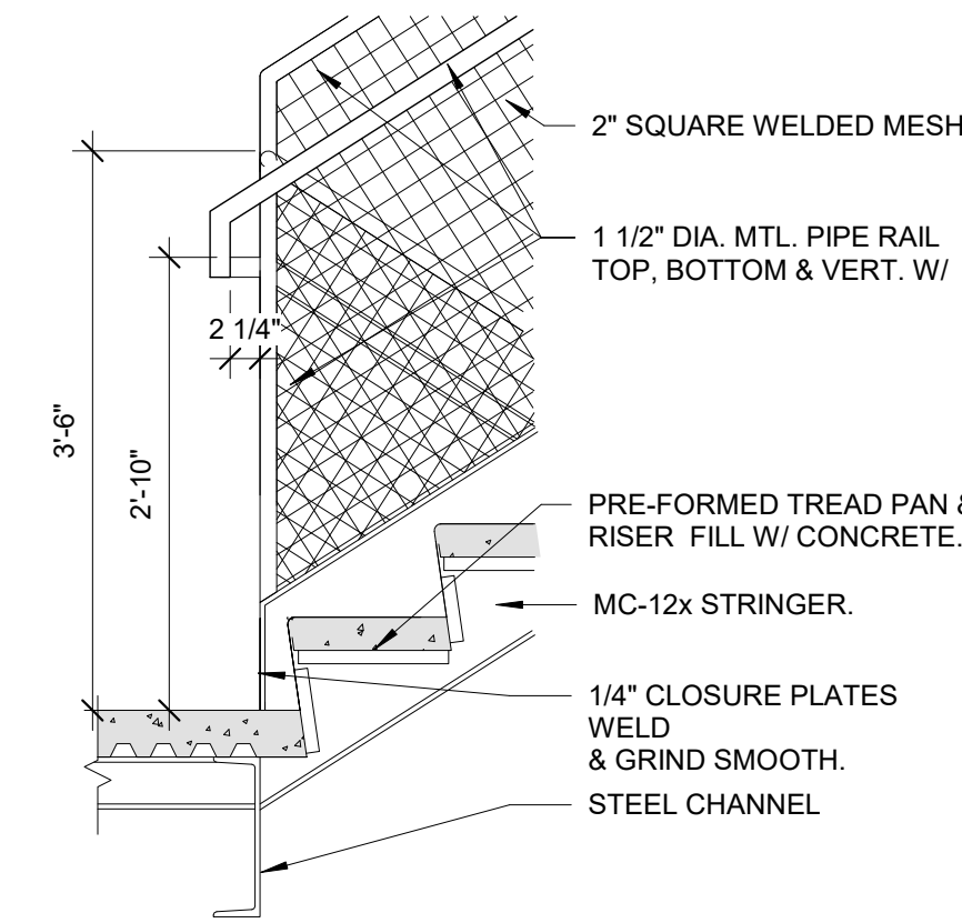
8 STAIR DETAIL - B/O RUN TO LANDING 3/4" = 1'-0"
