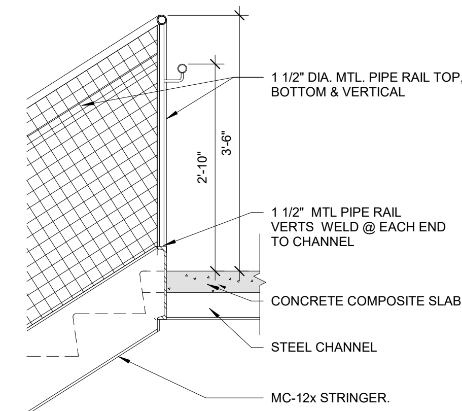
7 STAIR DETAIL - T/O RUN TO DECK 3/4" = 1'-0"
