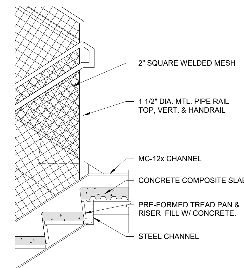
6 STAIR DETAIL - T/O RUN TO LANDING 3/4" = 1'-0"
