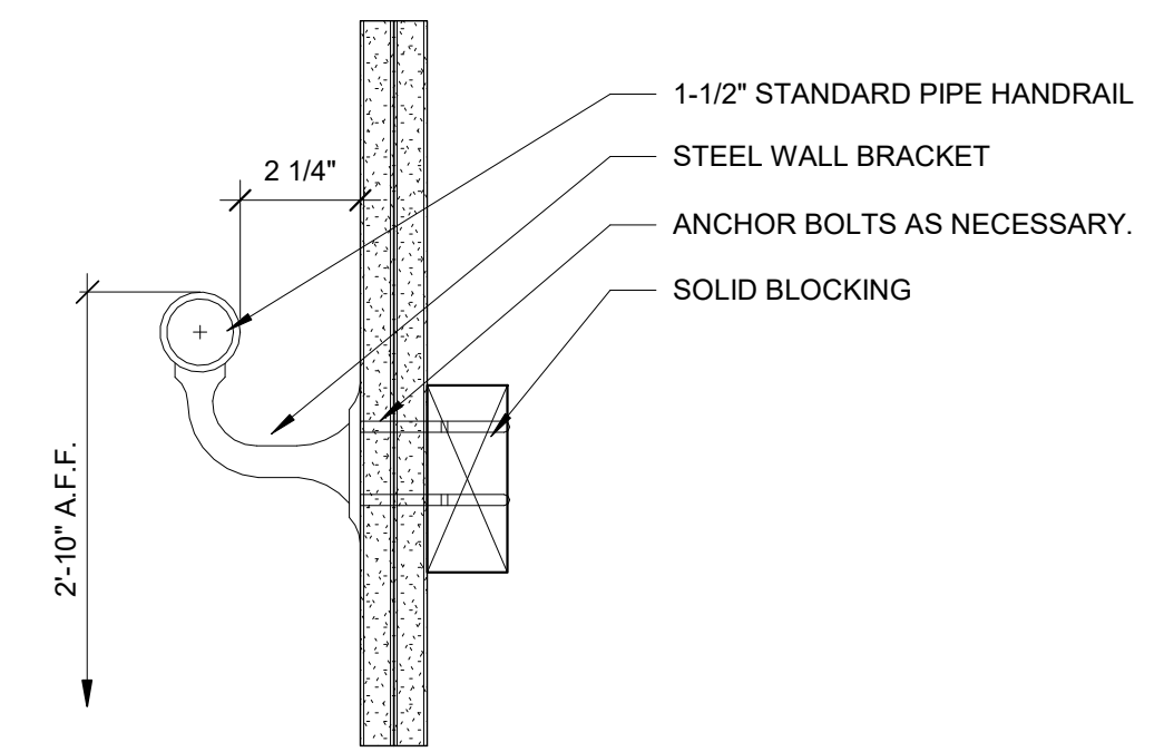
3 STAIR - METAL HANDRAIL DETAIL - SECTION 3" = 1'-0"
