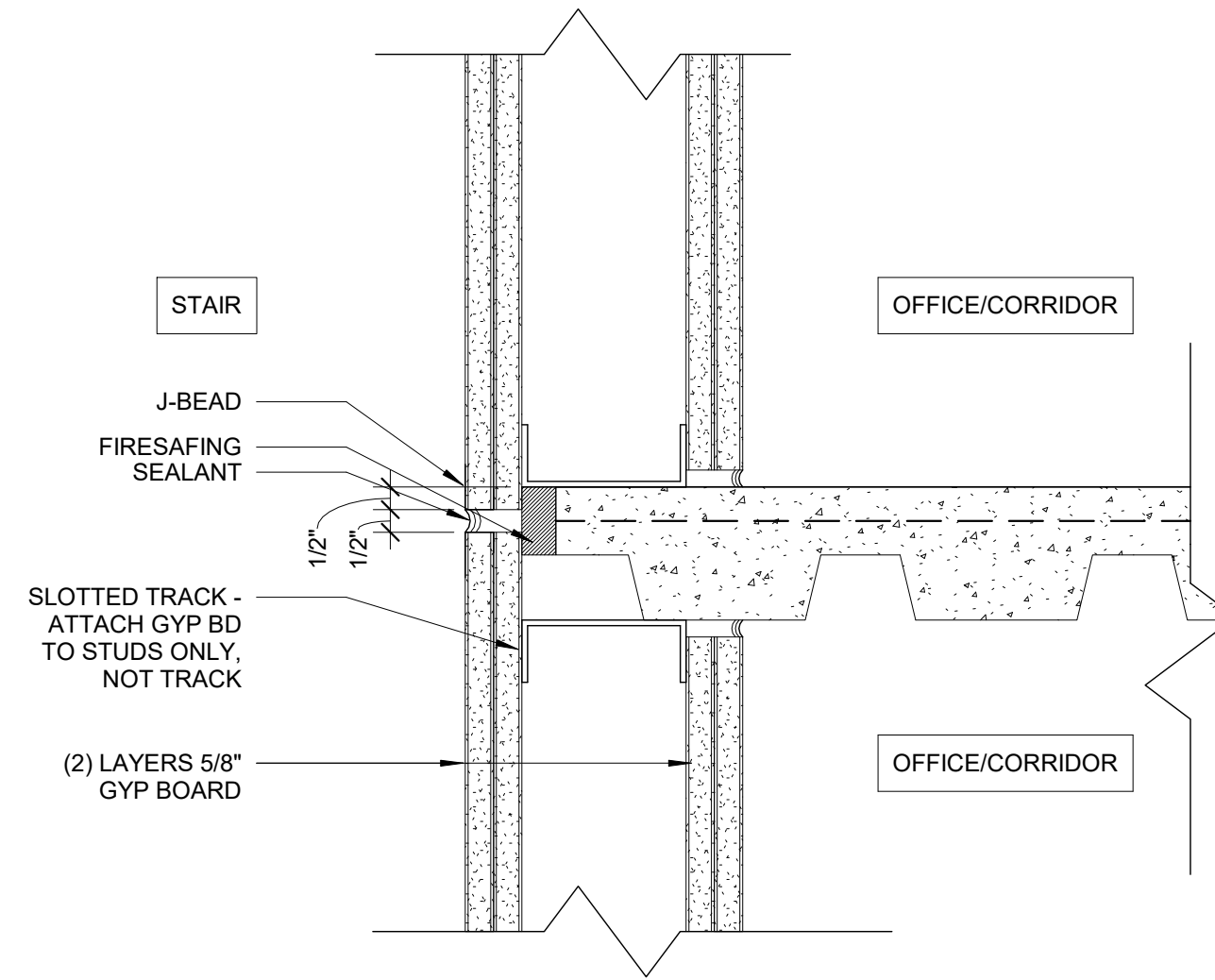
12 EDGE OF SLAB AT STAIR DETAIL 3" = 1'-0"
