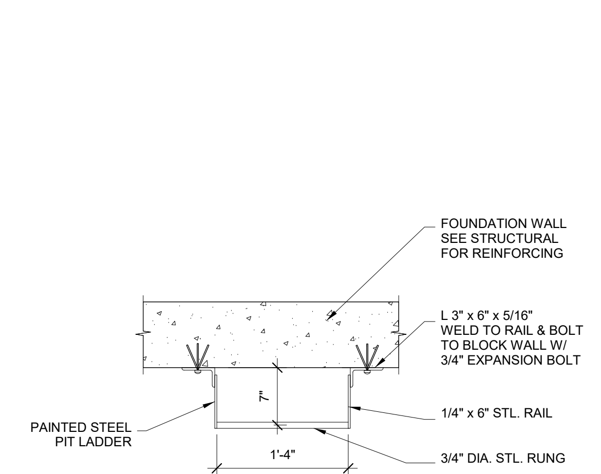
1 ELEVATOR PIT LADDER PLAN 1" = 1'-0"
