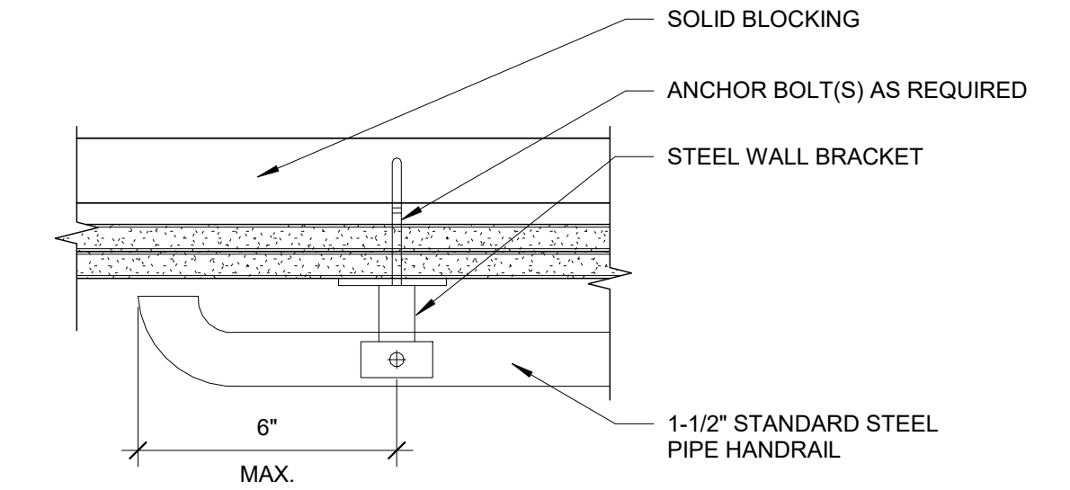
4 STAIR - METAL HANDRAIL DETAIL - PLAN 3" = 1'-0"
