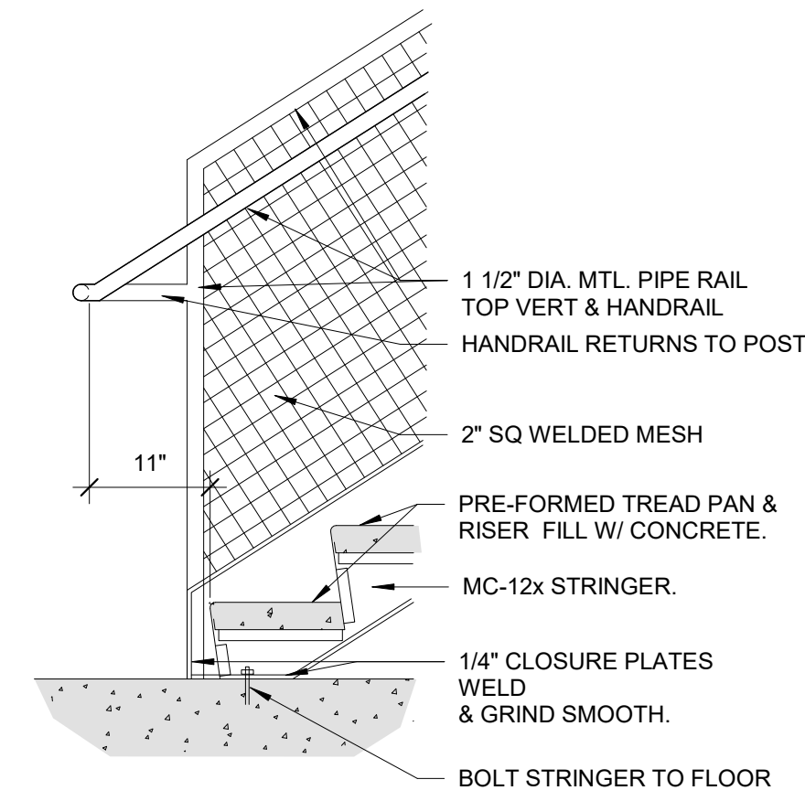
9 STAIR DETAIL - B/O RUN TO DECK 3/4" = 1'-0"
