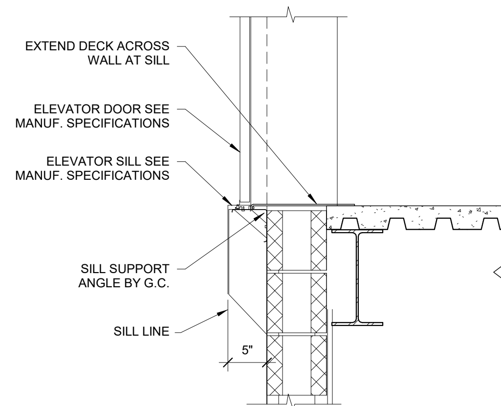
11 ELEVATOR DOOR THRESHOLD 1" = 1'-0"
