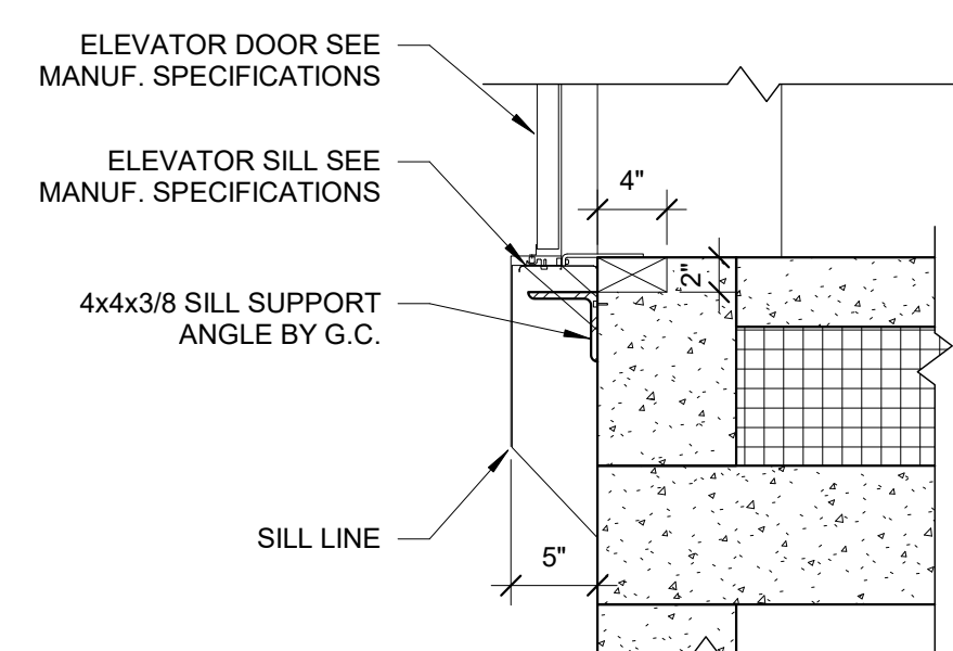
10 ELEVATOR DOOR AT CONCRETE 1" = 1'-0"
