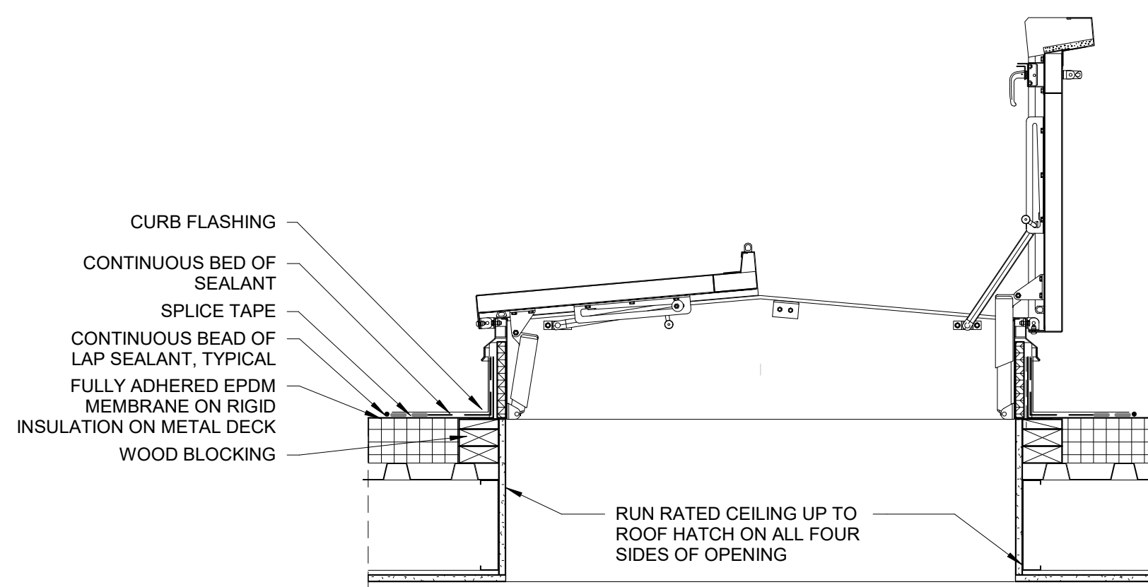
13 ROOF DETAIL - ROOF HATCH 1" = 1'-0"
