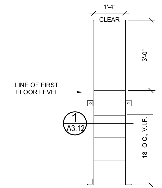
2 ELEVATOR PIT LADDER ELEVATION 1/2" = 1'-0"
