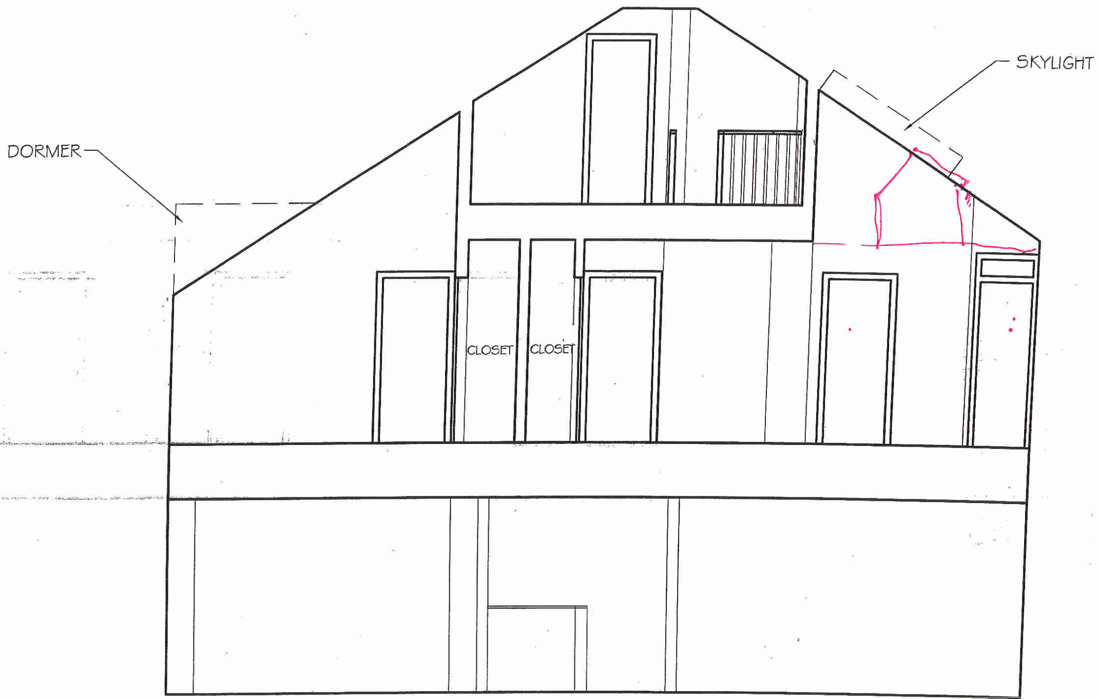
SECTION
