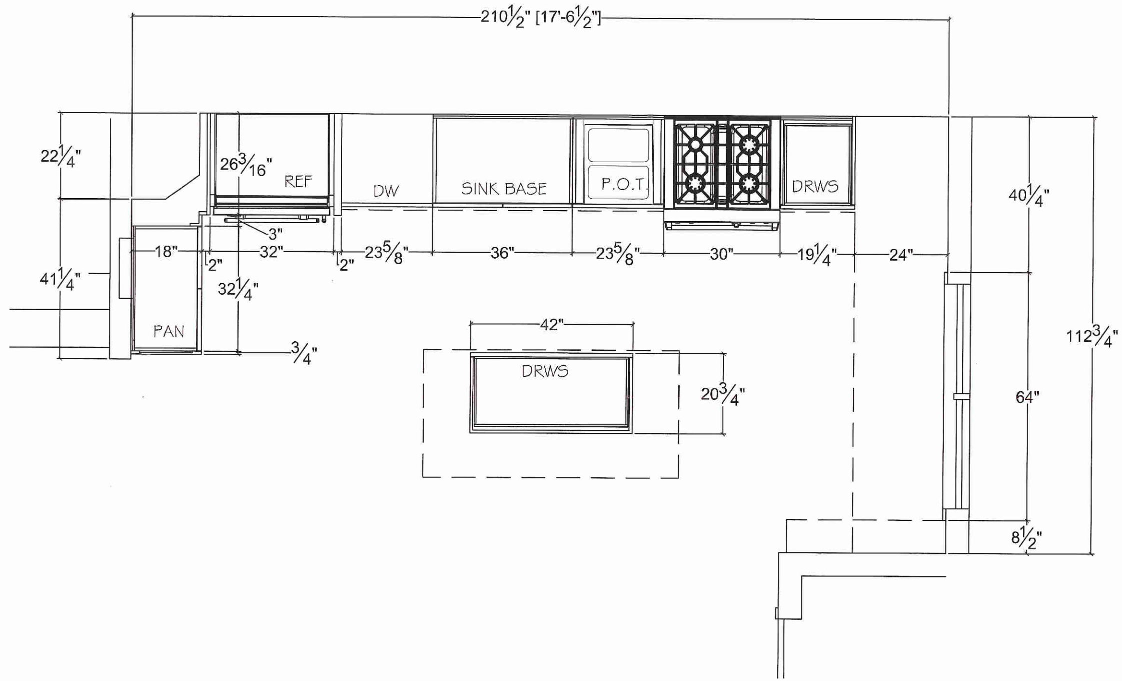
LOWER PLAN SECTION
