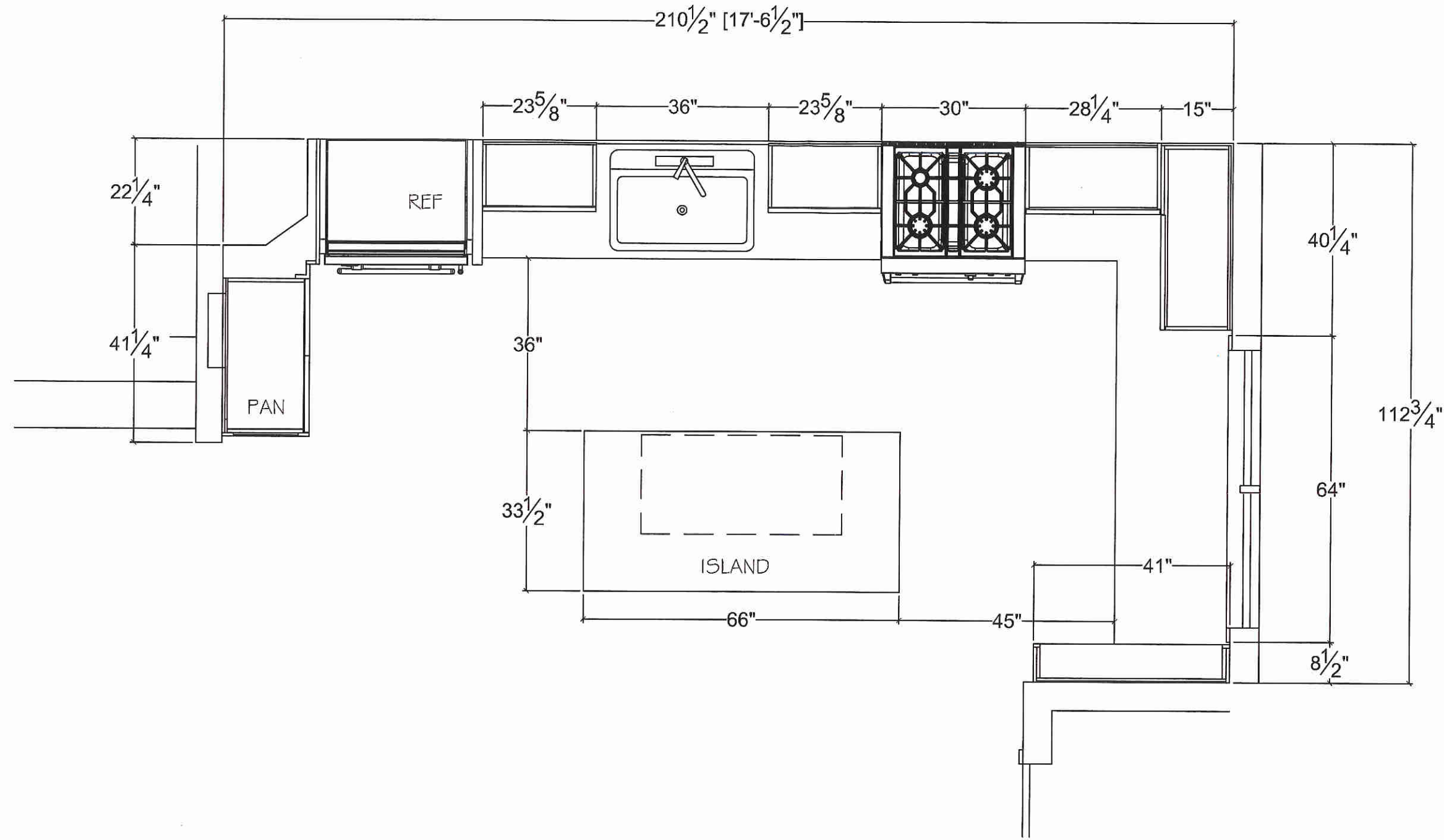
UPPER PLAN SECTION
