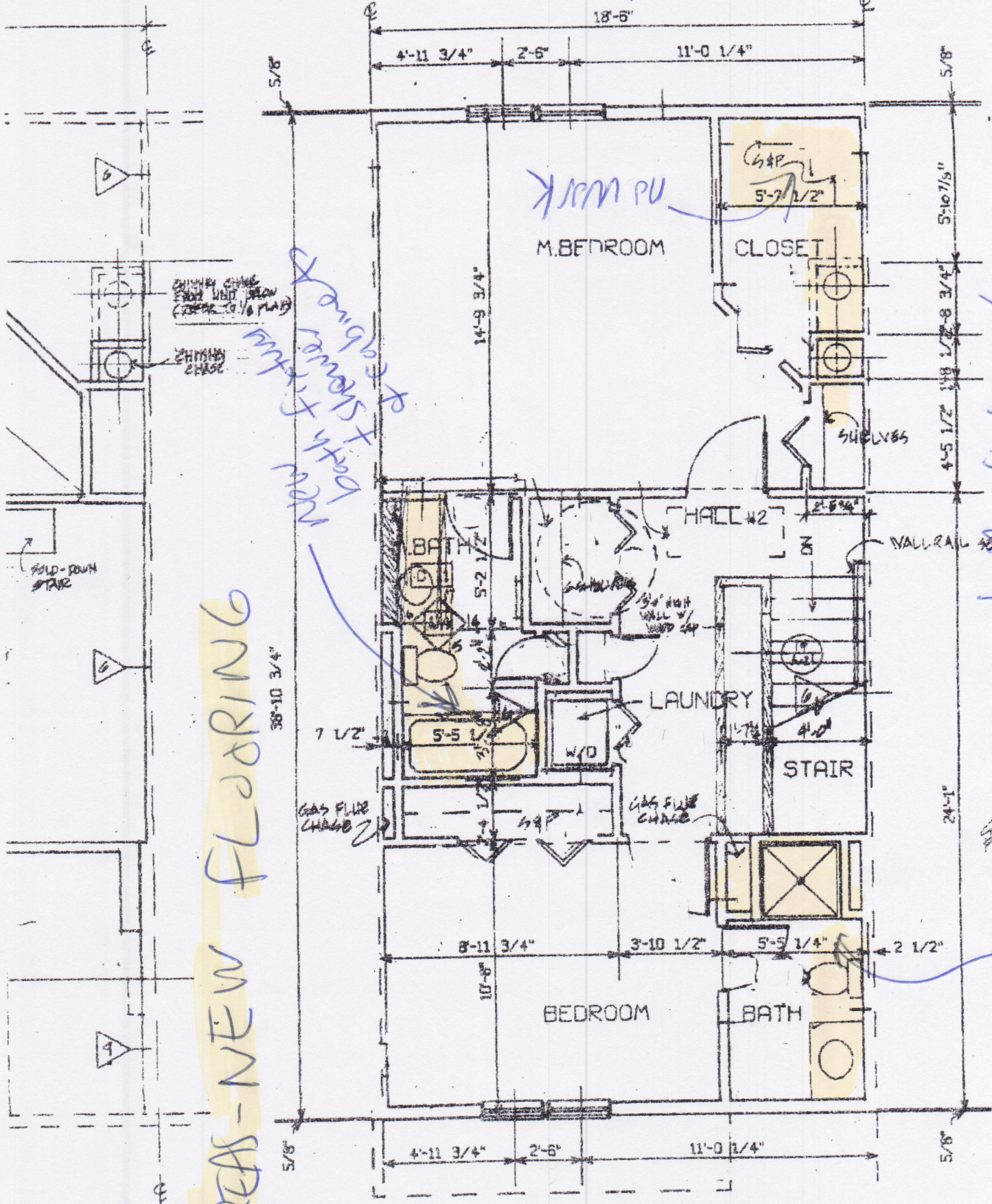
D UNIT PLAN Second Floor
