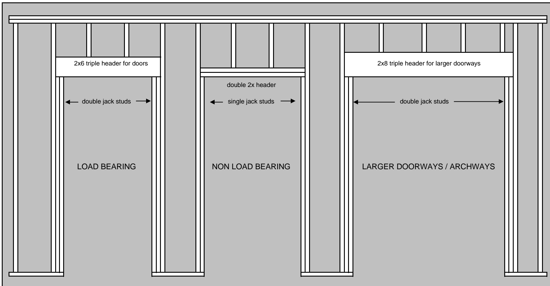
EXAMPLE OF FRAMING OF INTERIOR WALLS. NONE OF THE WALLS THAT WILL BE CONSTRUCTED OR REMOVED ARE LOAD BEARING. WALLS CONTAINING PLUMBING WILL BE 2 X 6. ALL OTHERS WILL BE 2 X 4
