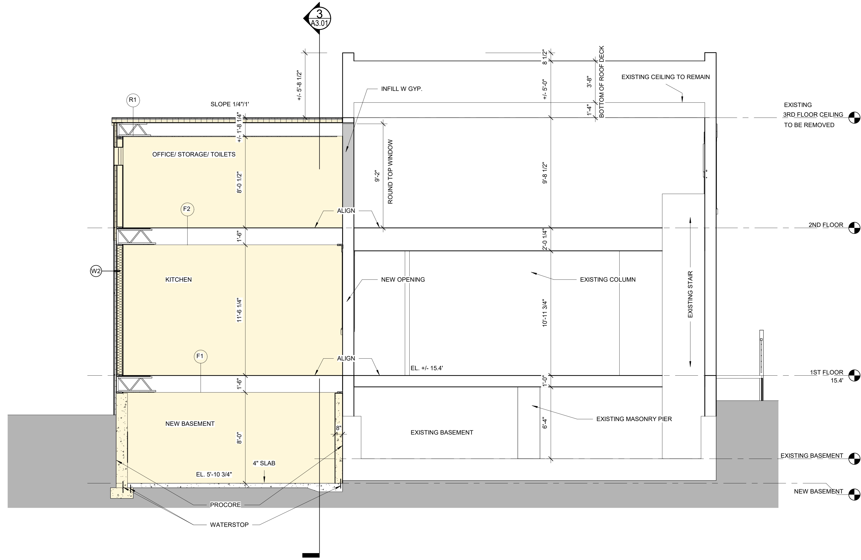
1 BUILDING SECTION 1/4" = 1'-0"
