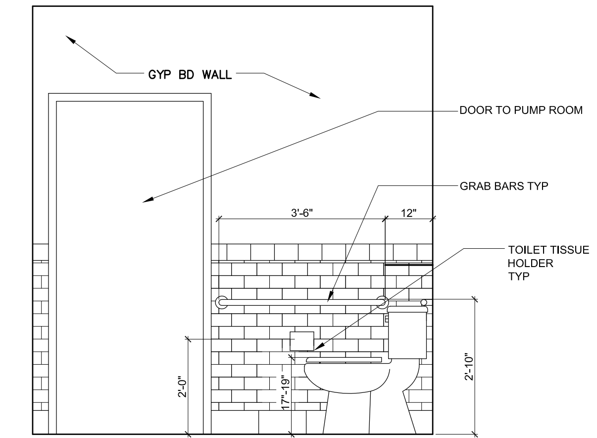
5 INTERIOR ELEVATION AT MEN'S RESTROOM 1/2"=1'-0"
