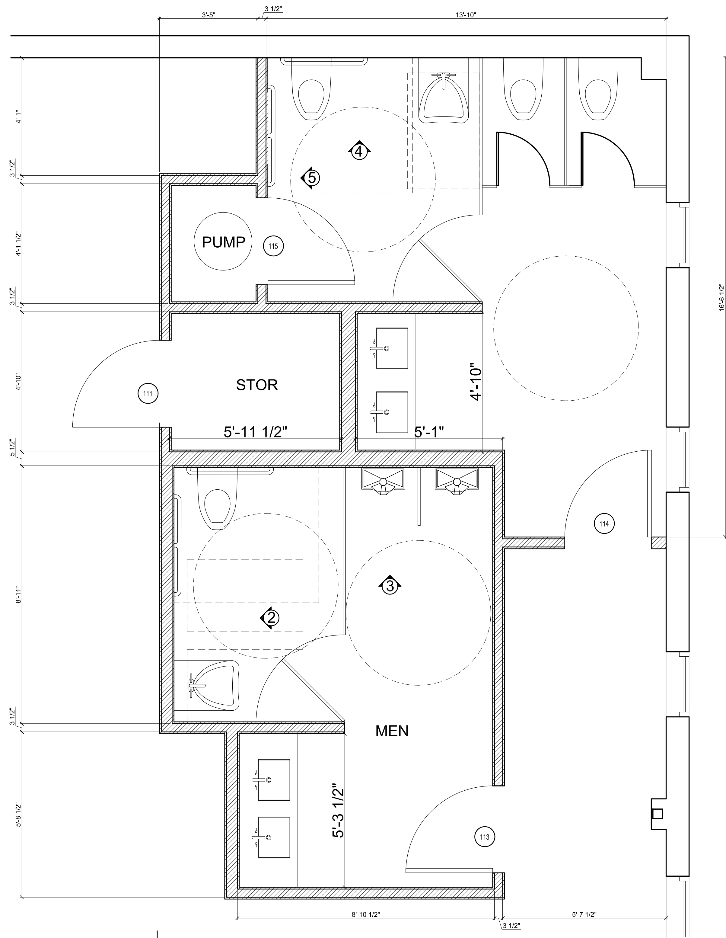
1 ENLARGED RESTROOM PLAN 1/2"=1'-0"
