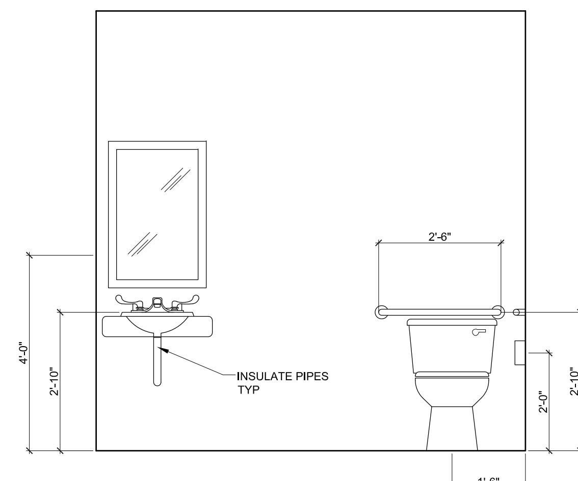
7 INTERIOR ELEVATION AT EMPLOYEE REST. 1/2"=1'-0"
