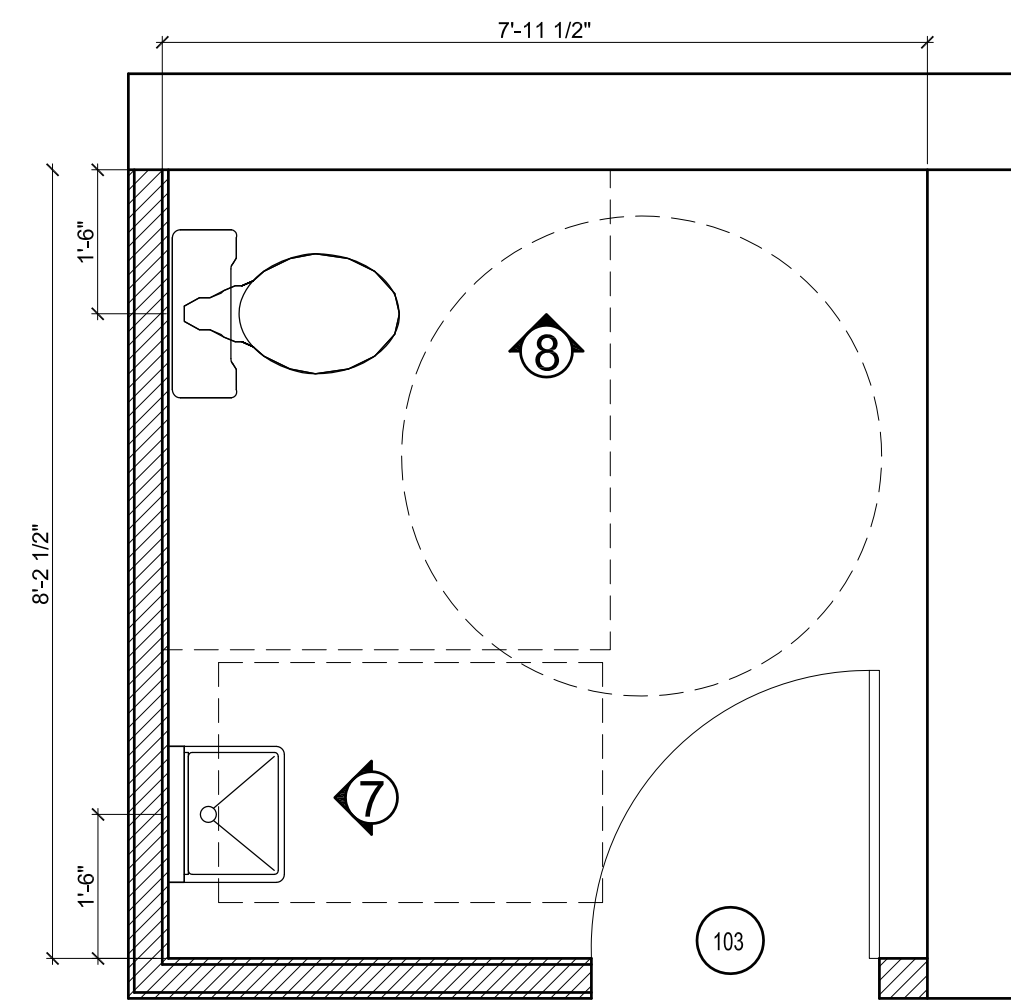
6 ENLARGED EMPLOYEE RESTROOM PLAN 1/2"=1'-0"
