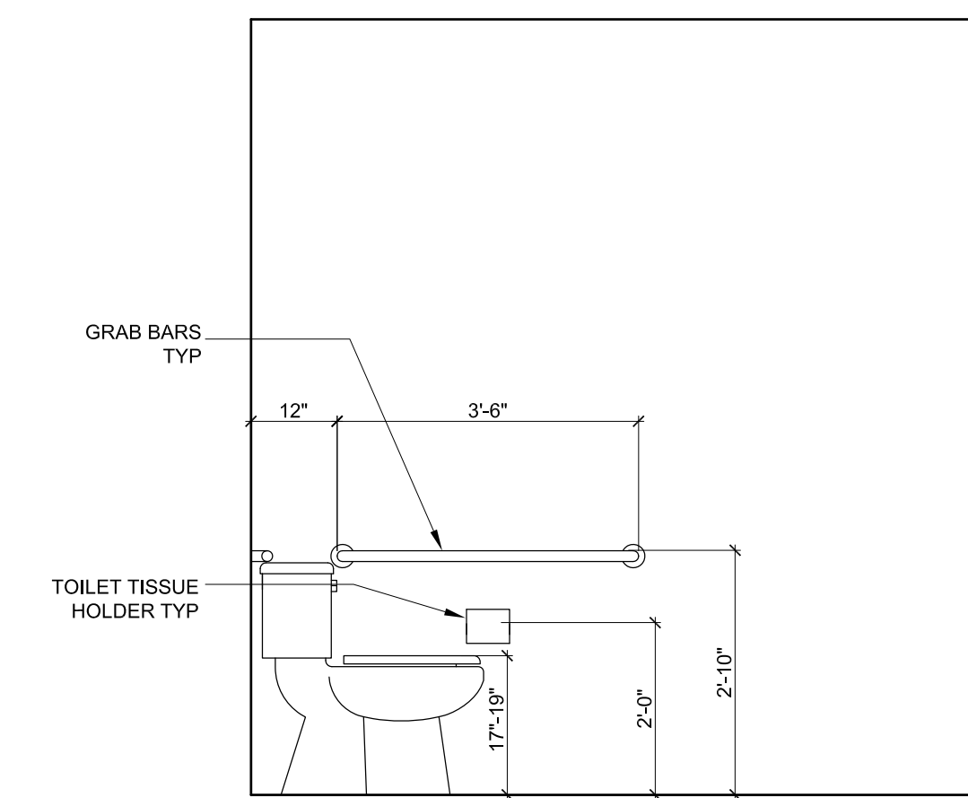
8 INTERIOR ELEVATION AT EMPLOYEE REST. 1/2"=1'-0"
