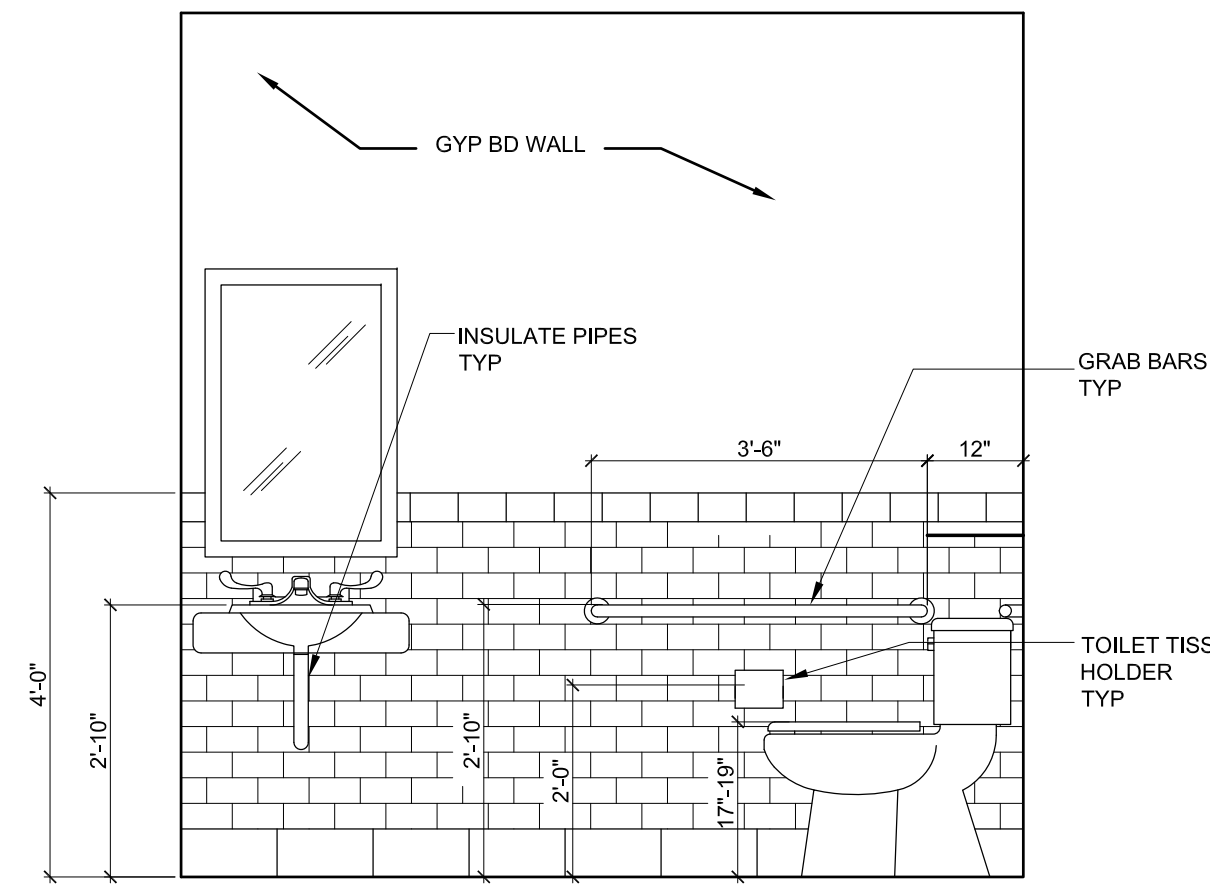
2 INTERIOR ELEVATION AT MEN'S RESTROOM 1/2"=1'-0"
