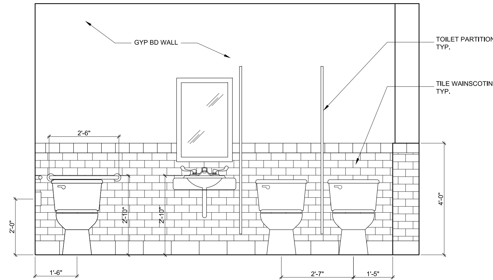
4 INTERIOR ELEVATION AT WOMEN'S RESTROOM 1/2"=1'-0"
