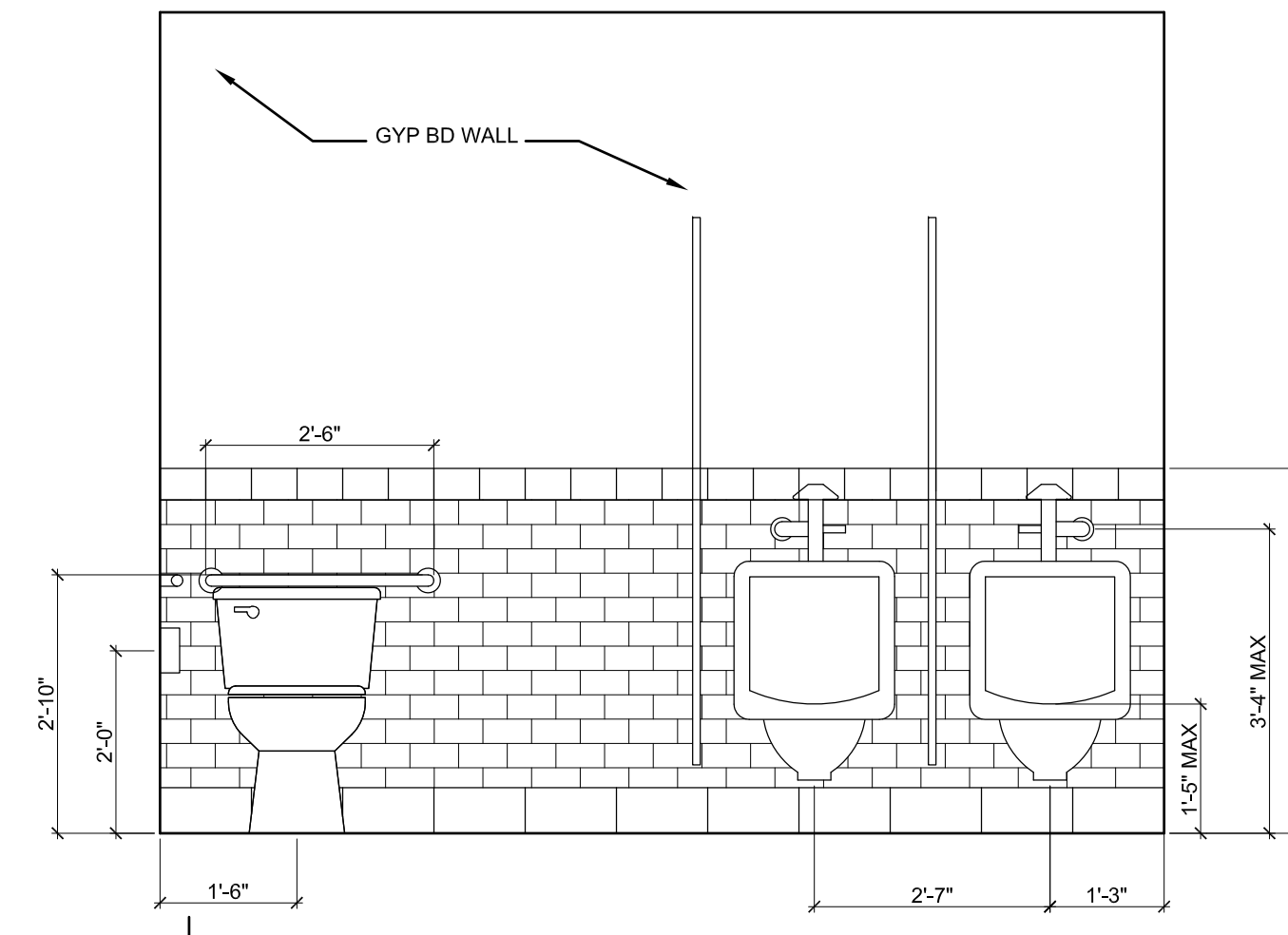
3 INTERIOR ELEVATION AT MEN'S RESTROOM 1/2"=1'-0"
