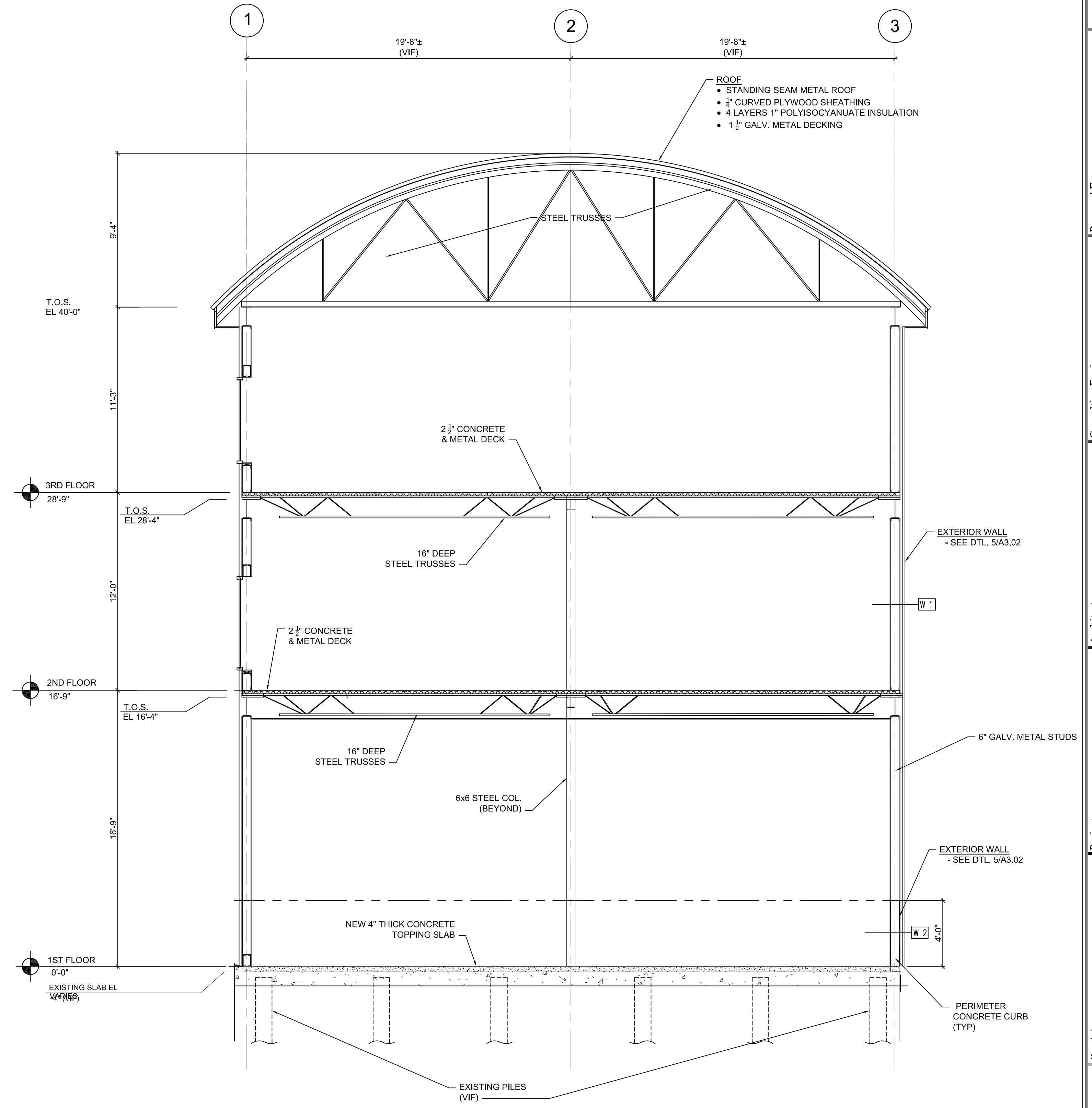
2 BUILDING SECTION 1/4" = 1'-0" 5' 4' 3' 2' 1' 0 5' 10'
