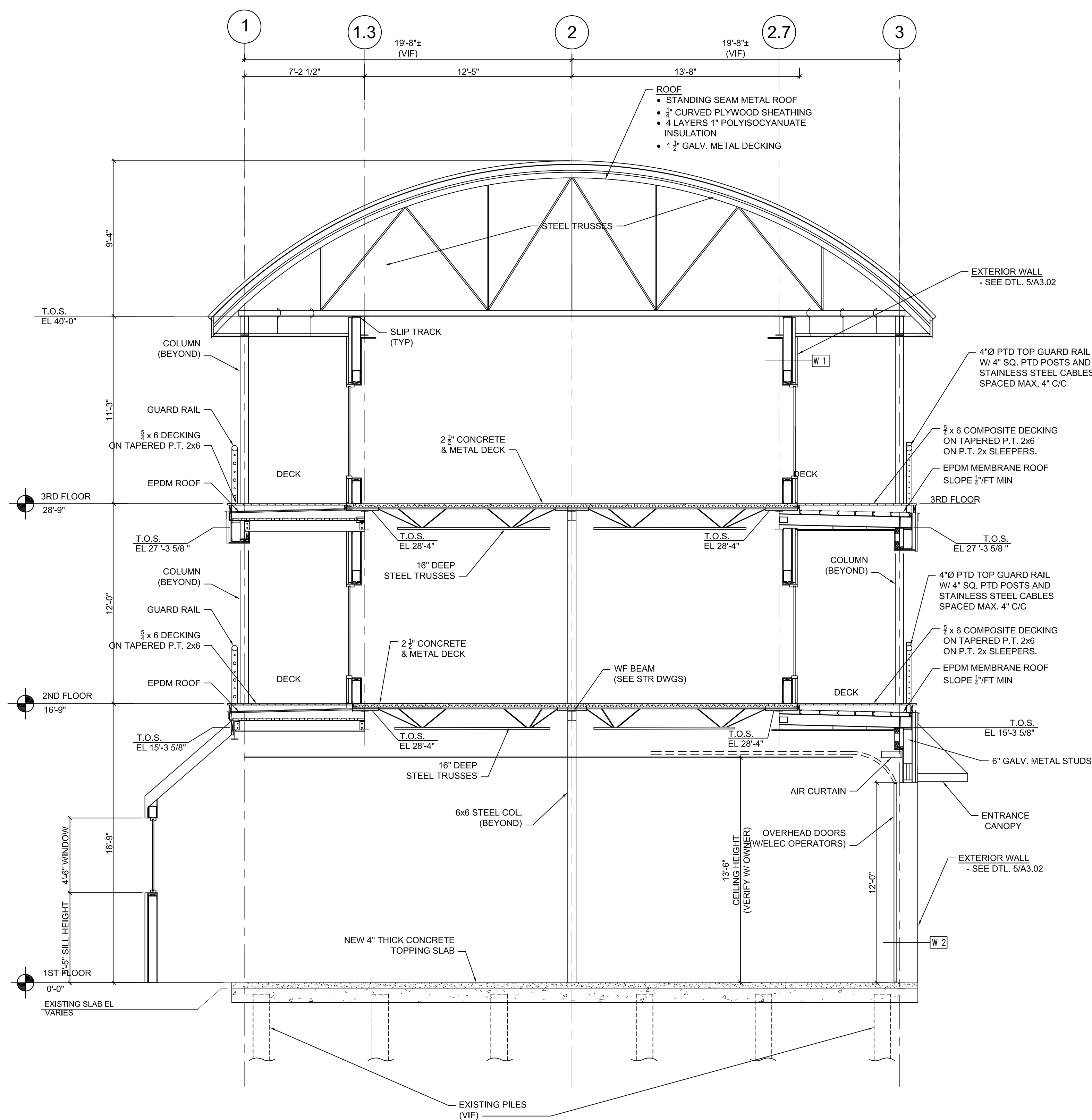
1 BUILDING SECTION 1/4" = 1'-0" 5' 4' 3' 2' 1' 0 5' 10'
