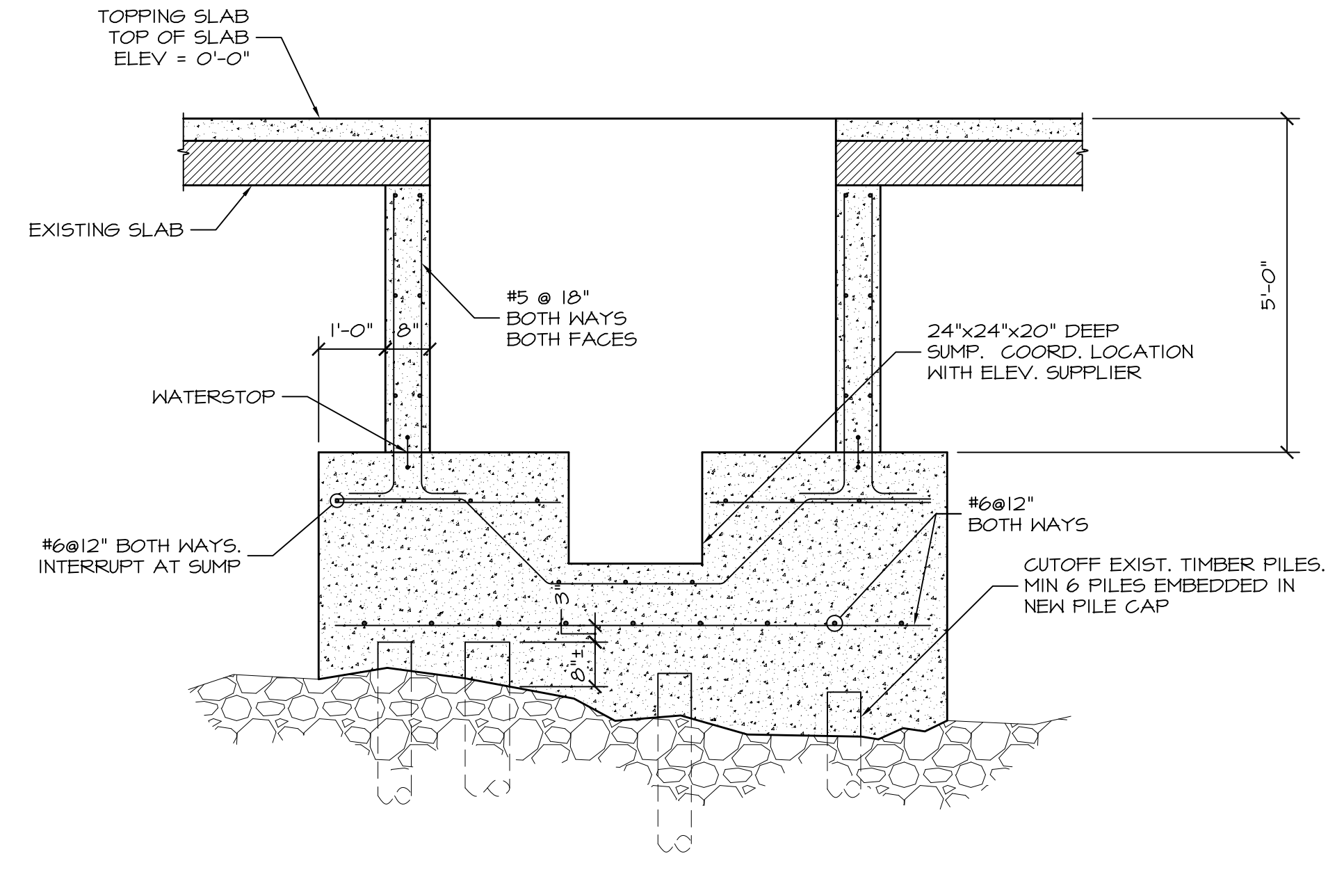
SECTION 1 1/2"=1'-0" S2.01 COORDINATE ALL ELEVATOR PIT DIMENSIONS WITH ELEVATOR SUPPLIER.
