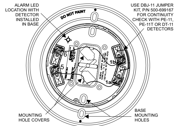
Figure 4 Mounting The DB-11 Base
