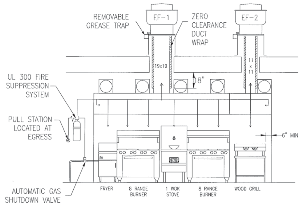
ELEVATION HOOD #1&2
