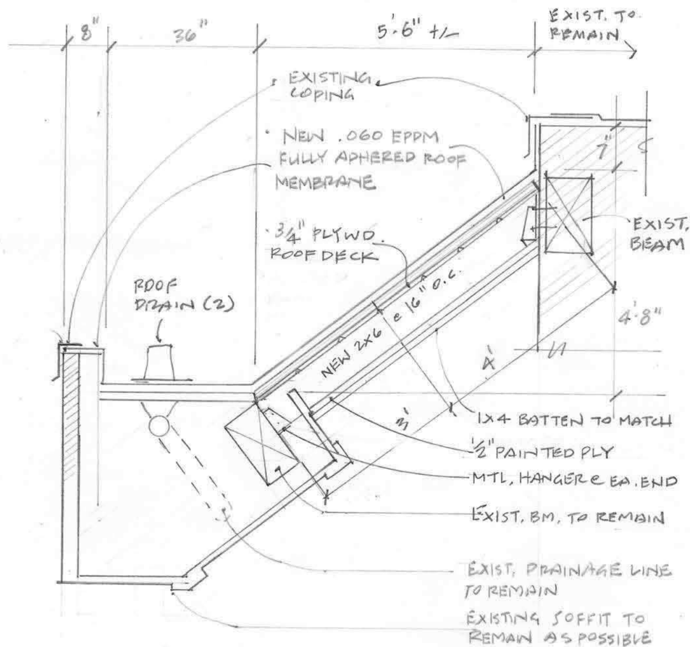
ROOF DETAIL NEW 1/2" = 1'
