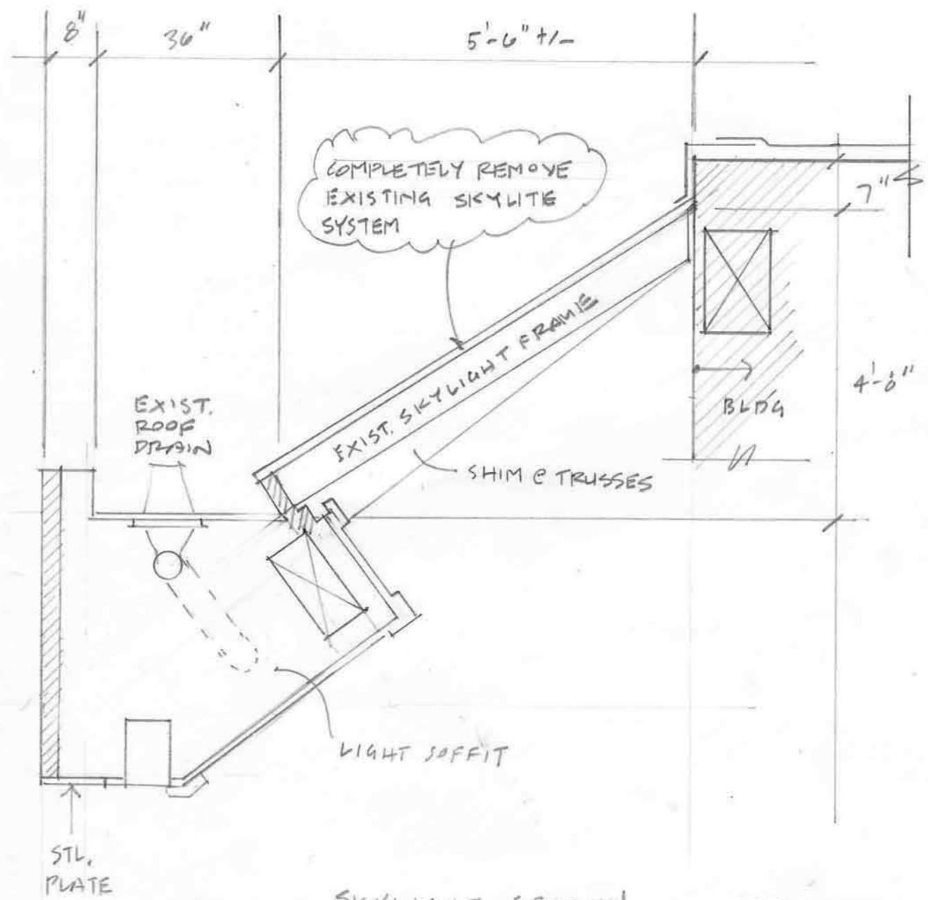
SKYLIGHT SECTION EXISTING 1/2" = 1'
