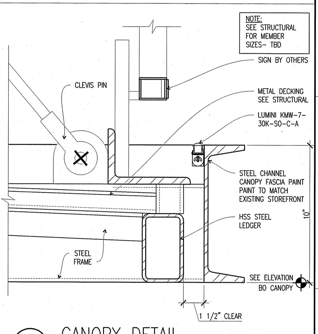
C9 CANOPY DETAIL 3'-1'-0"
