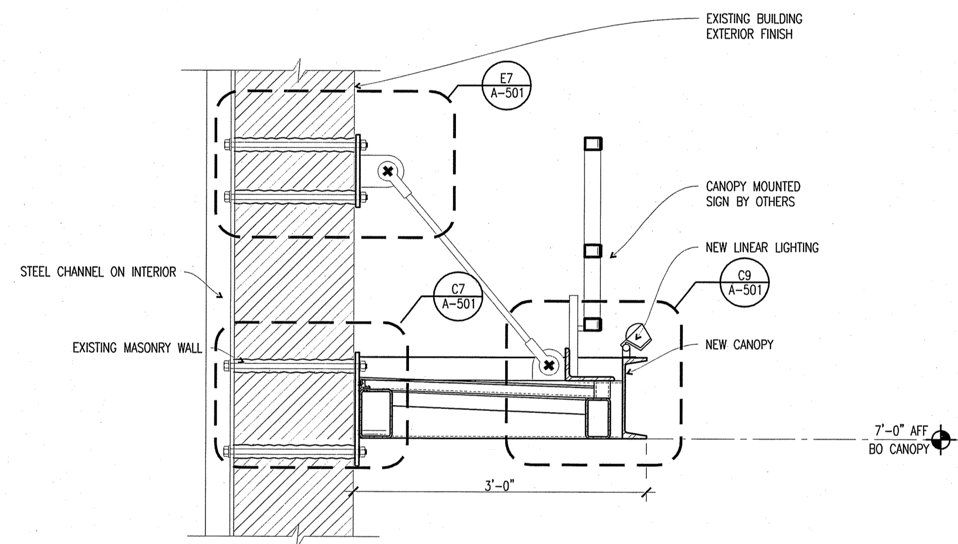
C1 CANOPY SECTION 1'-1'-0"
