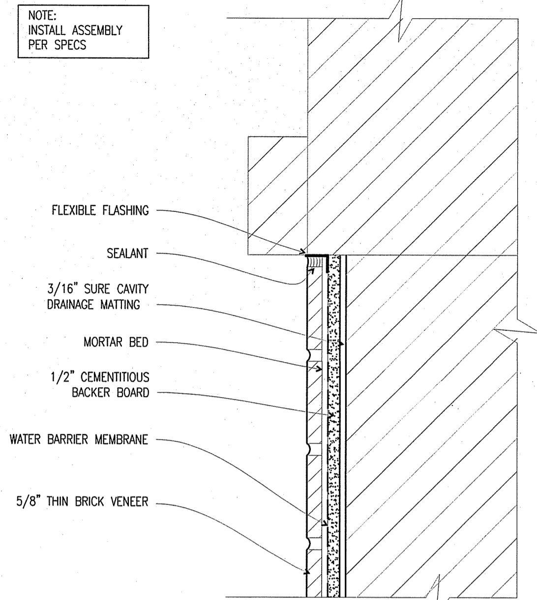
C CURVED HEAD / JAMB
