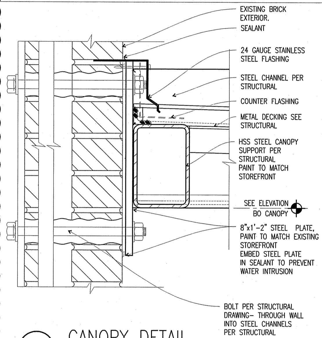
C7 CANOPY DETAIL 3'-1'-0"
