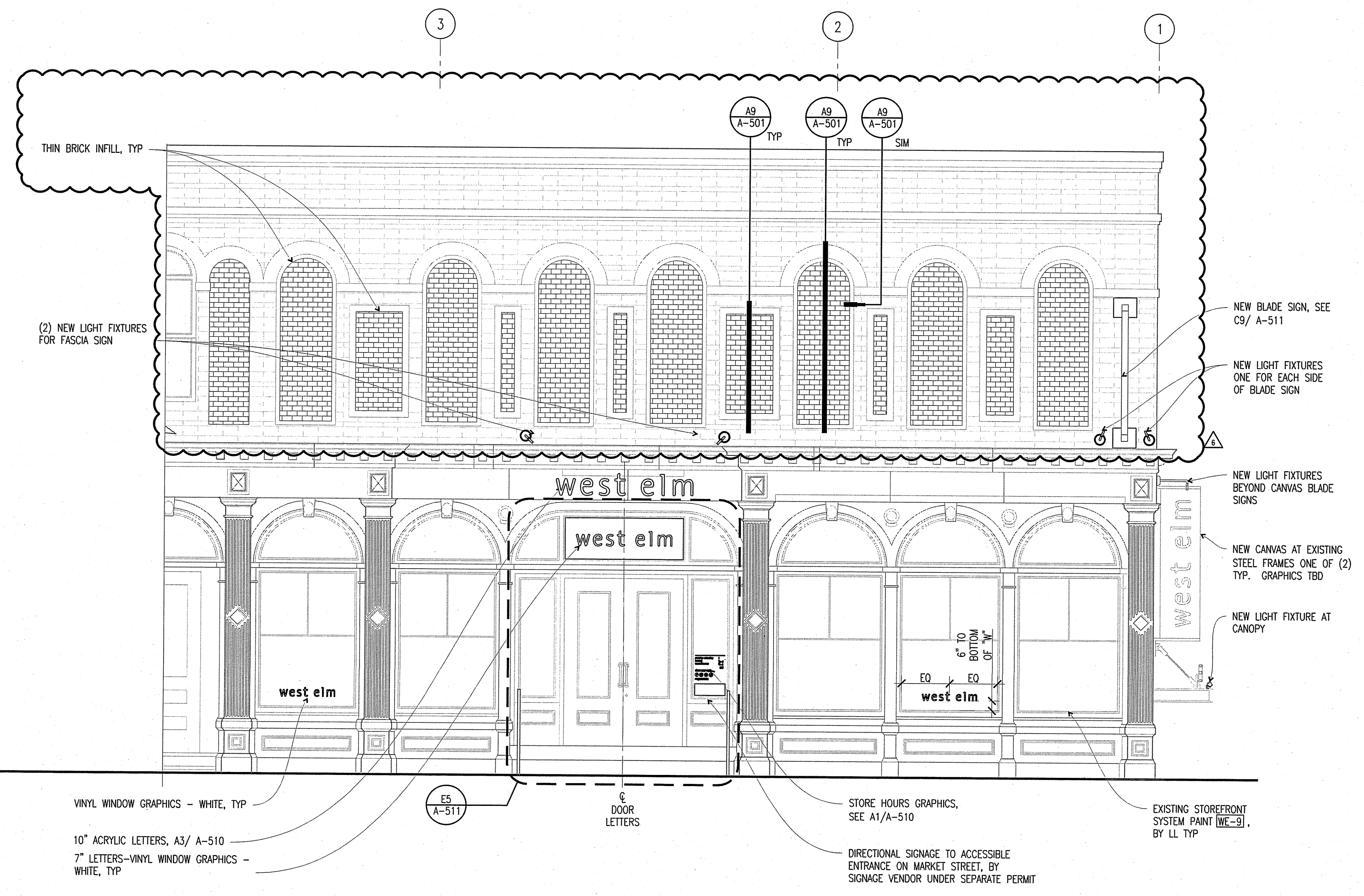
A1 ENLARGED EXTERIOR ELEVATION - ENTRY NO 1 1/4"=1'-0"
