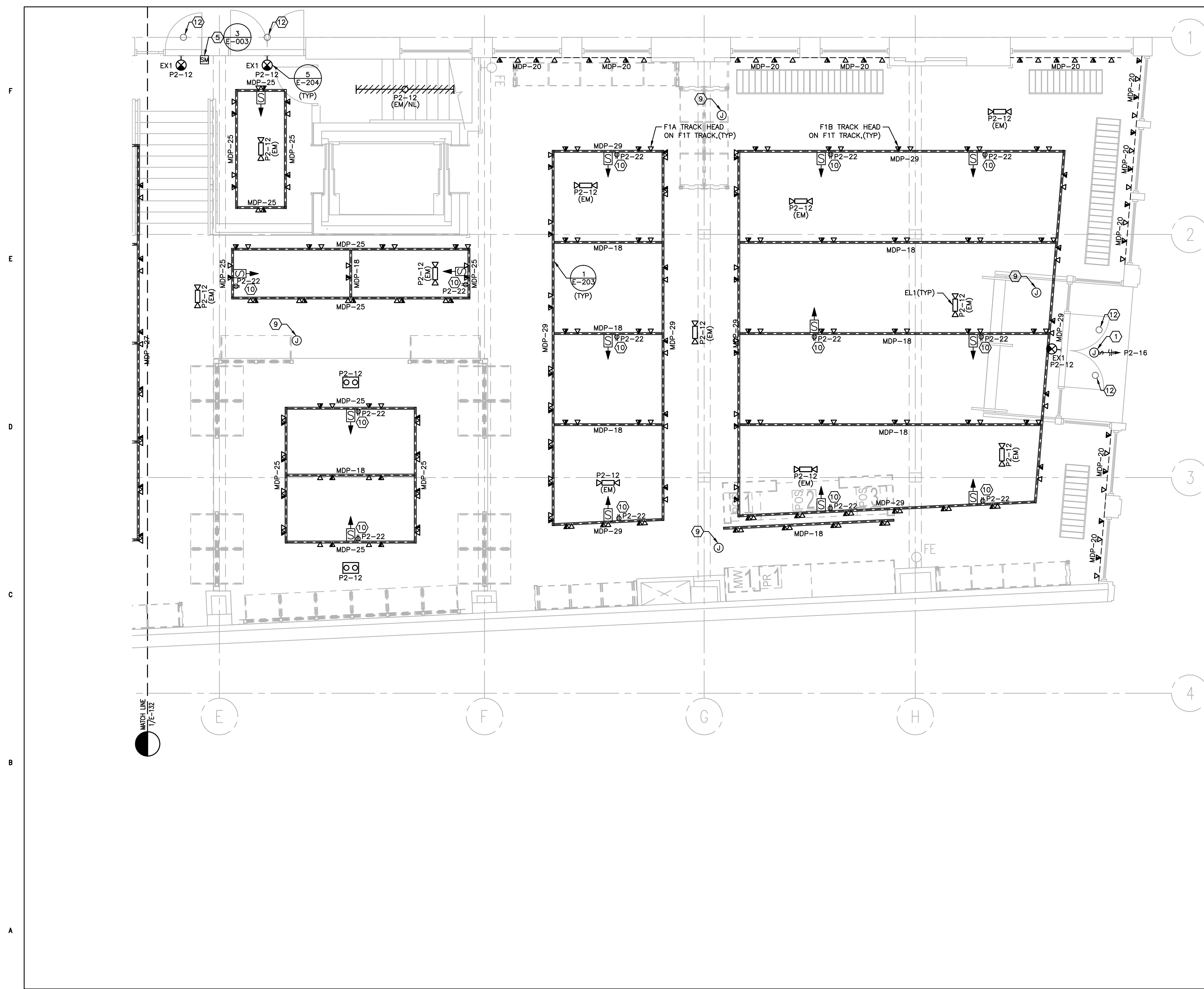
PARTIAL FIRST FLOOR LIGHTING PLAN
