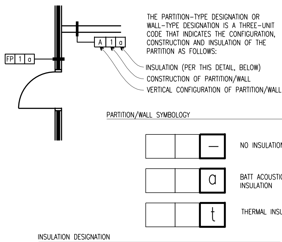
C1 PARTITION-TYPE LEGEND NO SCALE
