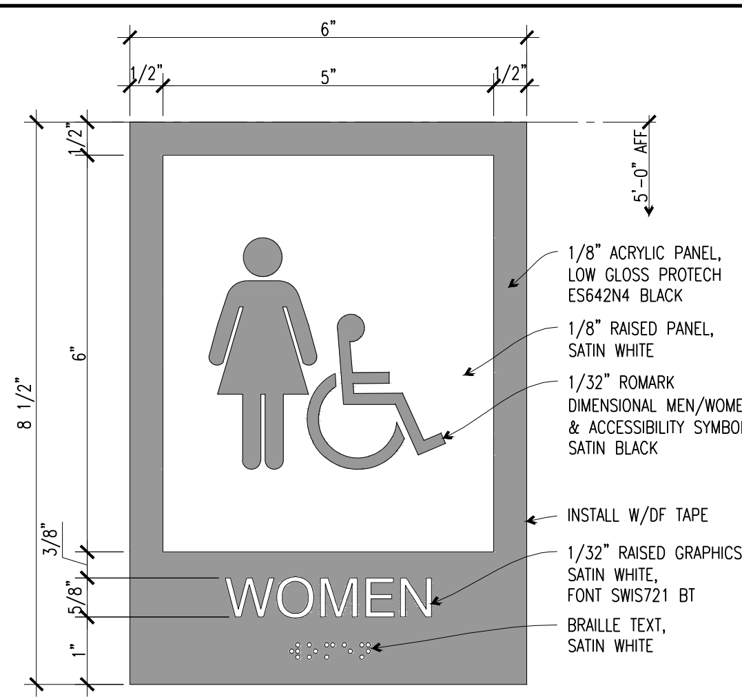
E5 PUBLIC RESTROOM SIGNAGE 6"=1'-0" SIGNAGE FOIO
