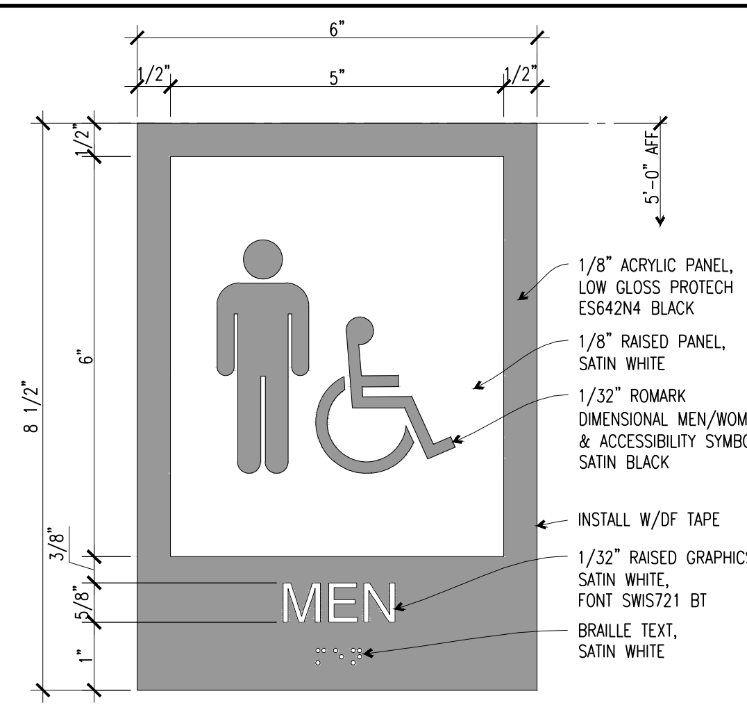
E7 PUBLIC RESTROOM SIGNAGE 6"=1'-0" SIGNAGE FOIO
