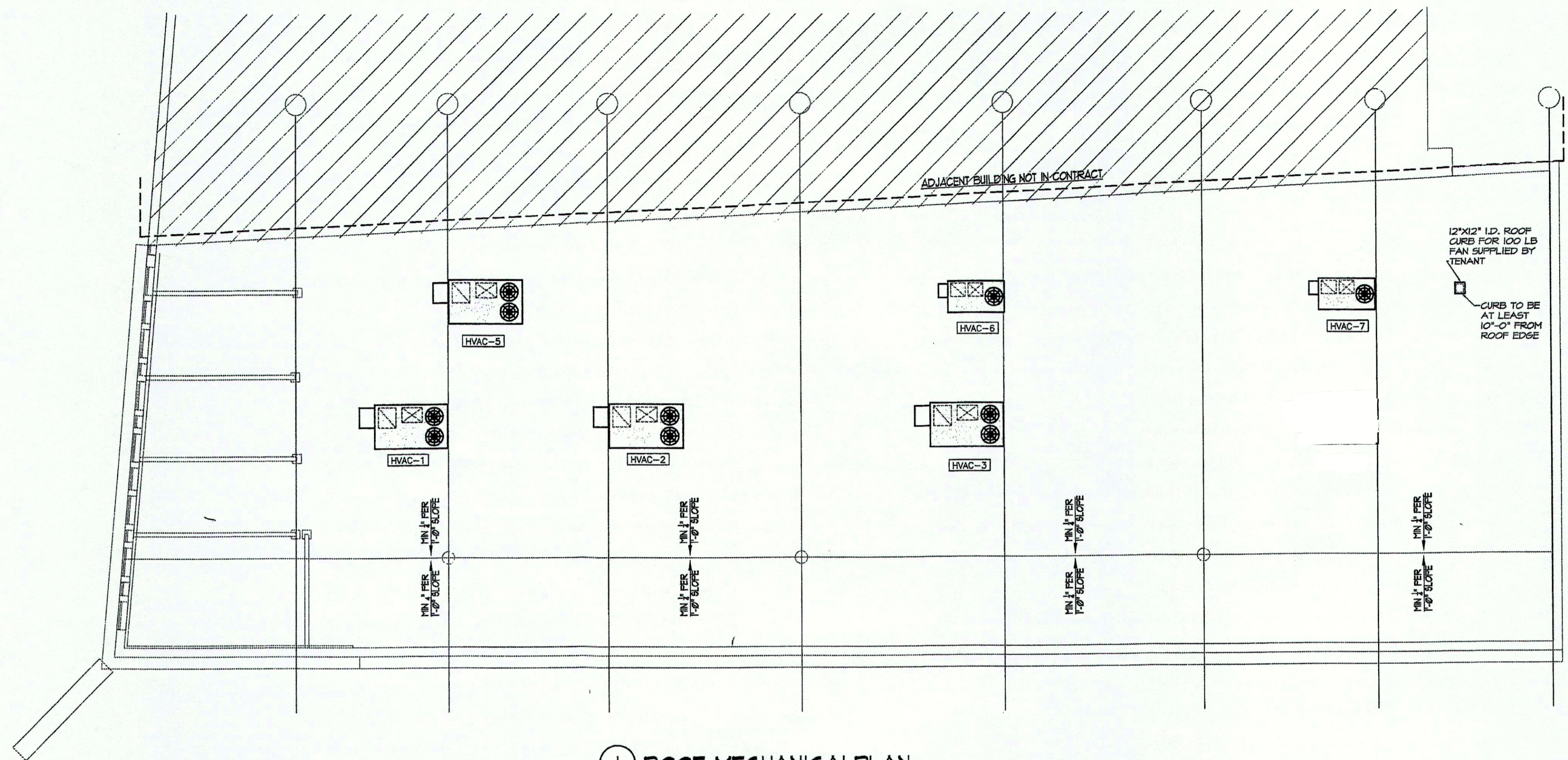
1 ROOF MECHANICAL PLAN SCALE: 1/8" = 1'-0"
