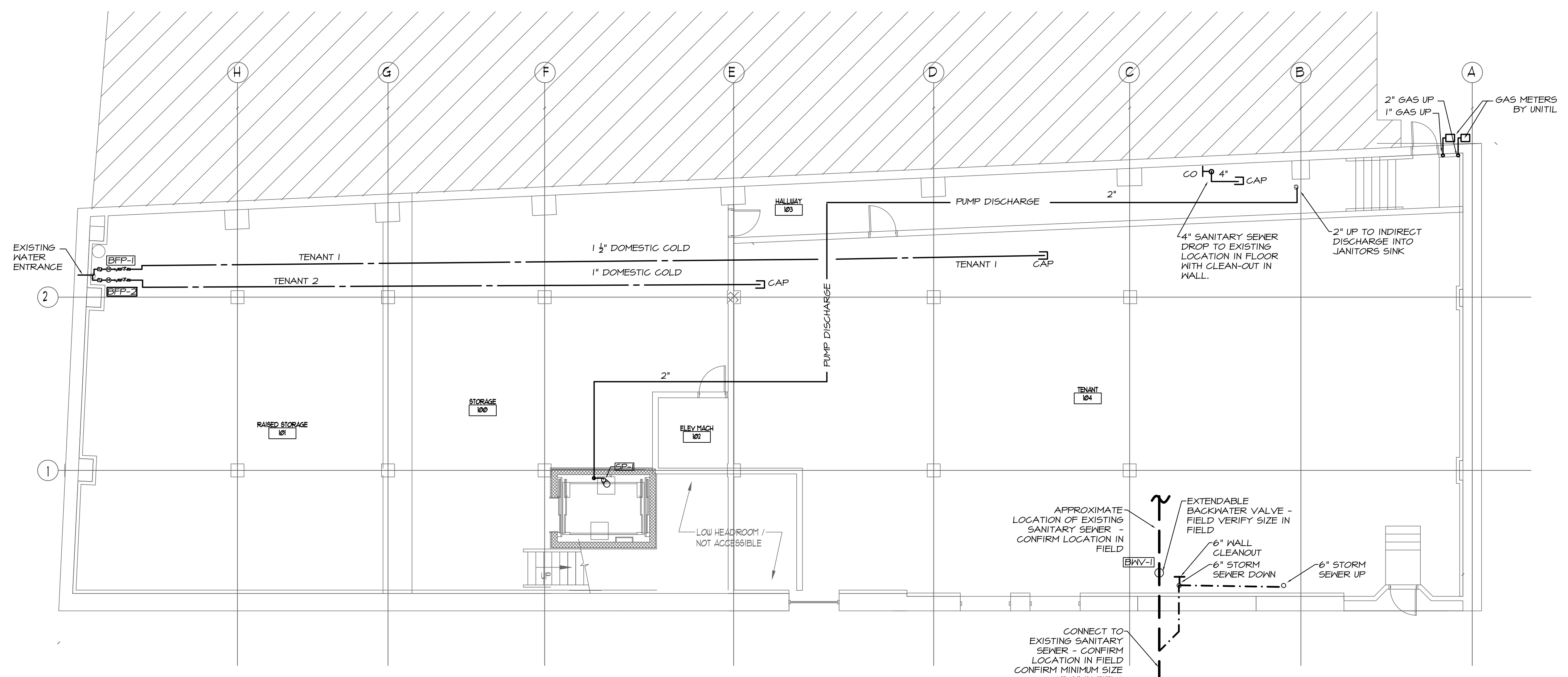
2 LOWER LEVEL PLUMBING PLAN SCALE: 1/8" = 1'-0"
