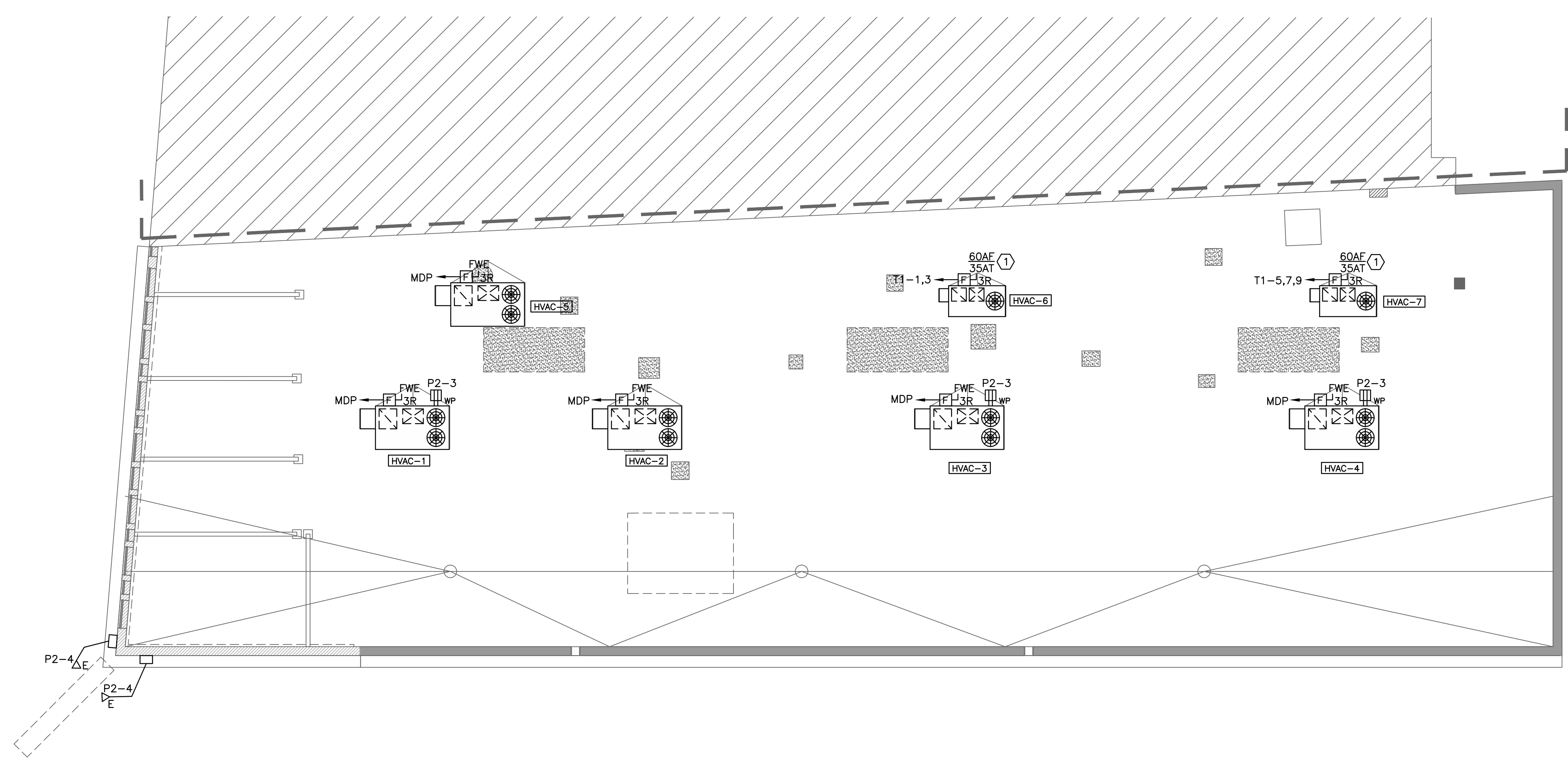
1 ELECTRICAL ROOF PLAN SCALE: 1/8"=1'-0"
