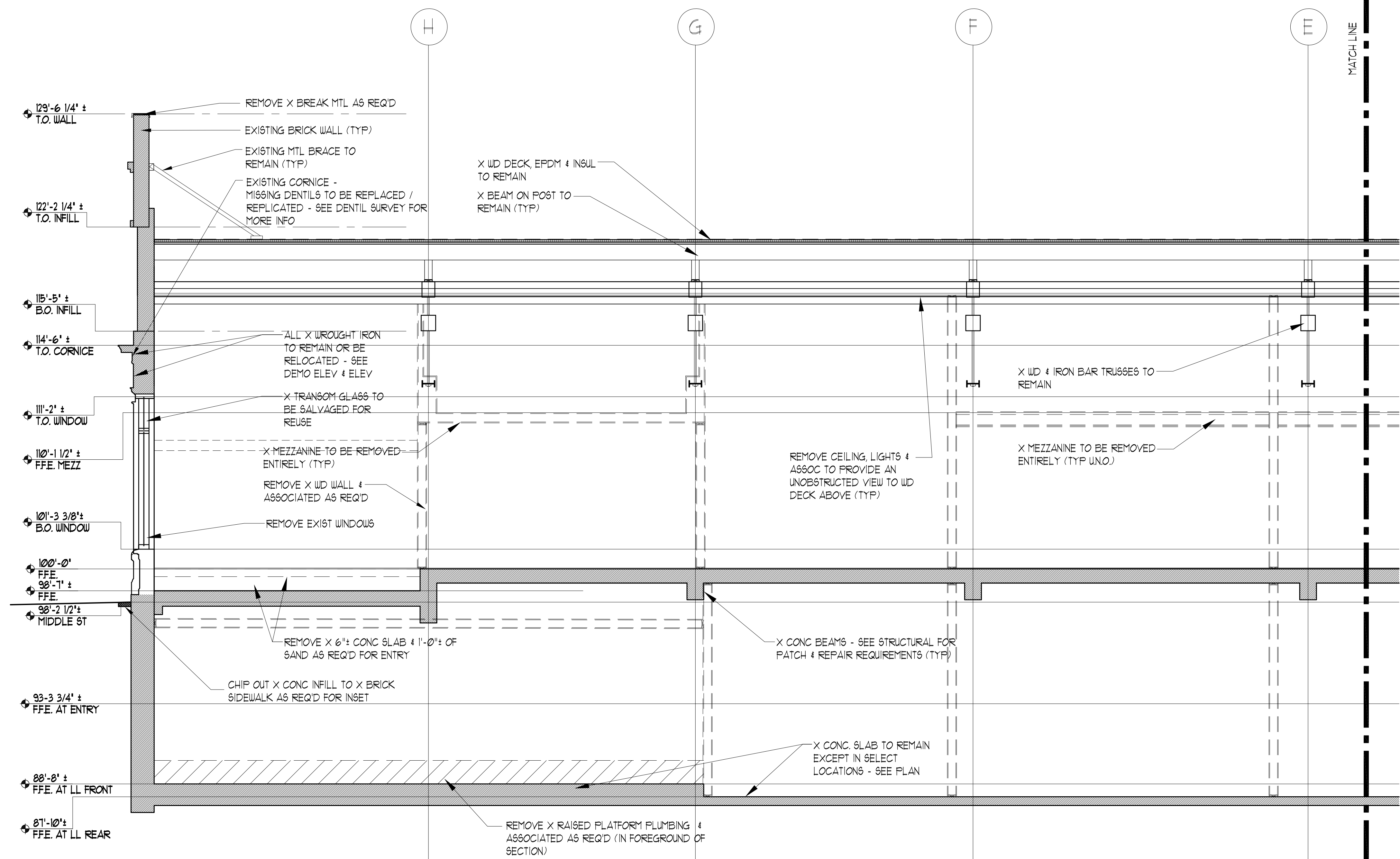
1 DEMO BUILDING SECTION D11P3.3 0 4'-0" SCALE: 1/4" = 1'-0"
