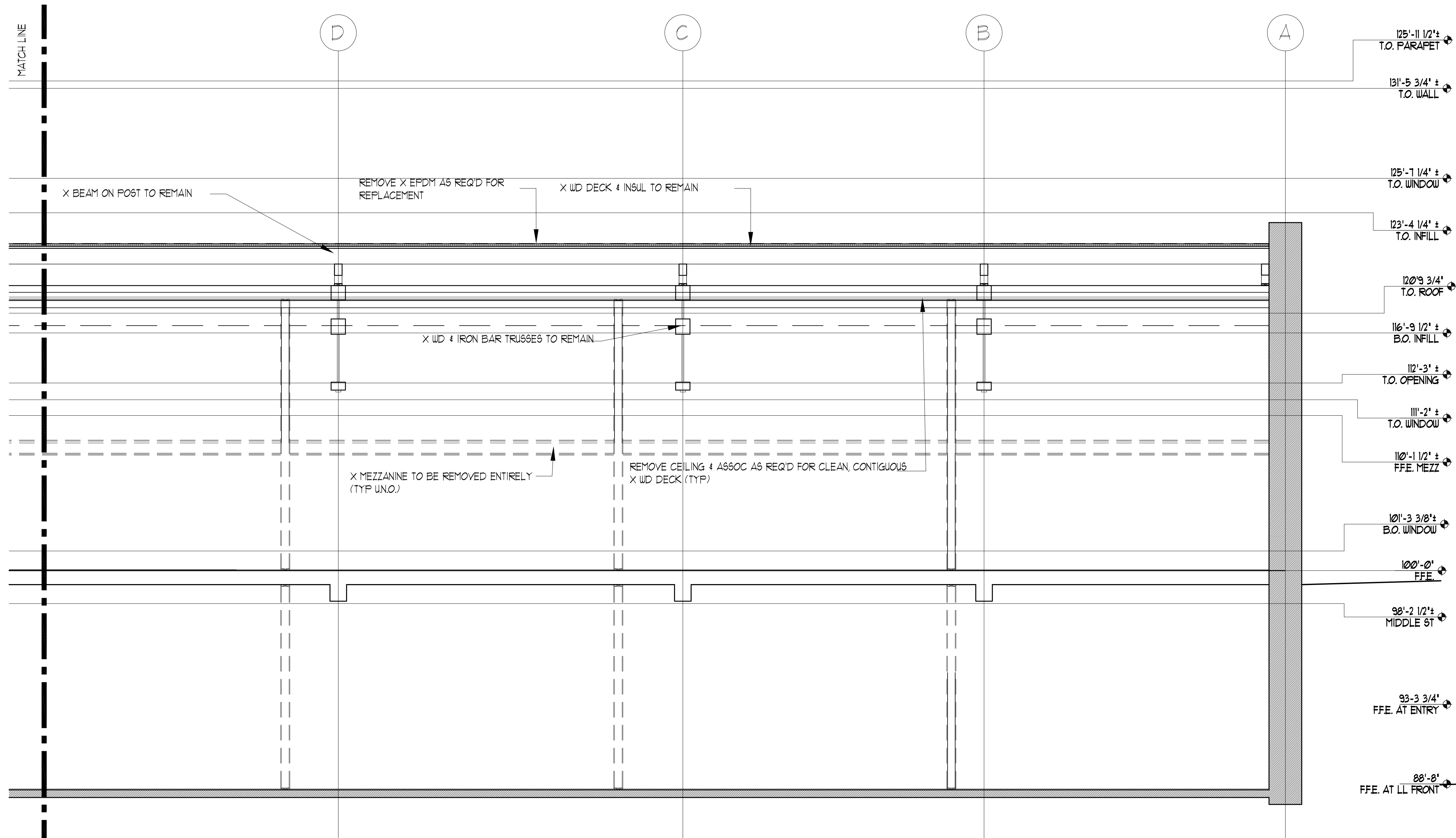
DEMO BUILDING SECTION SCALE: 1/8" = 1'-0"
