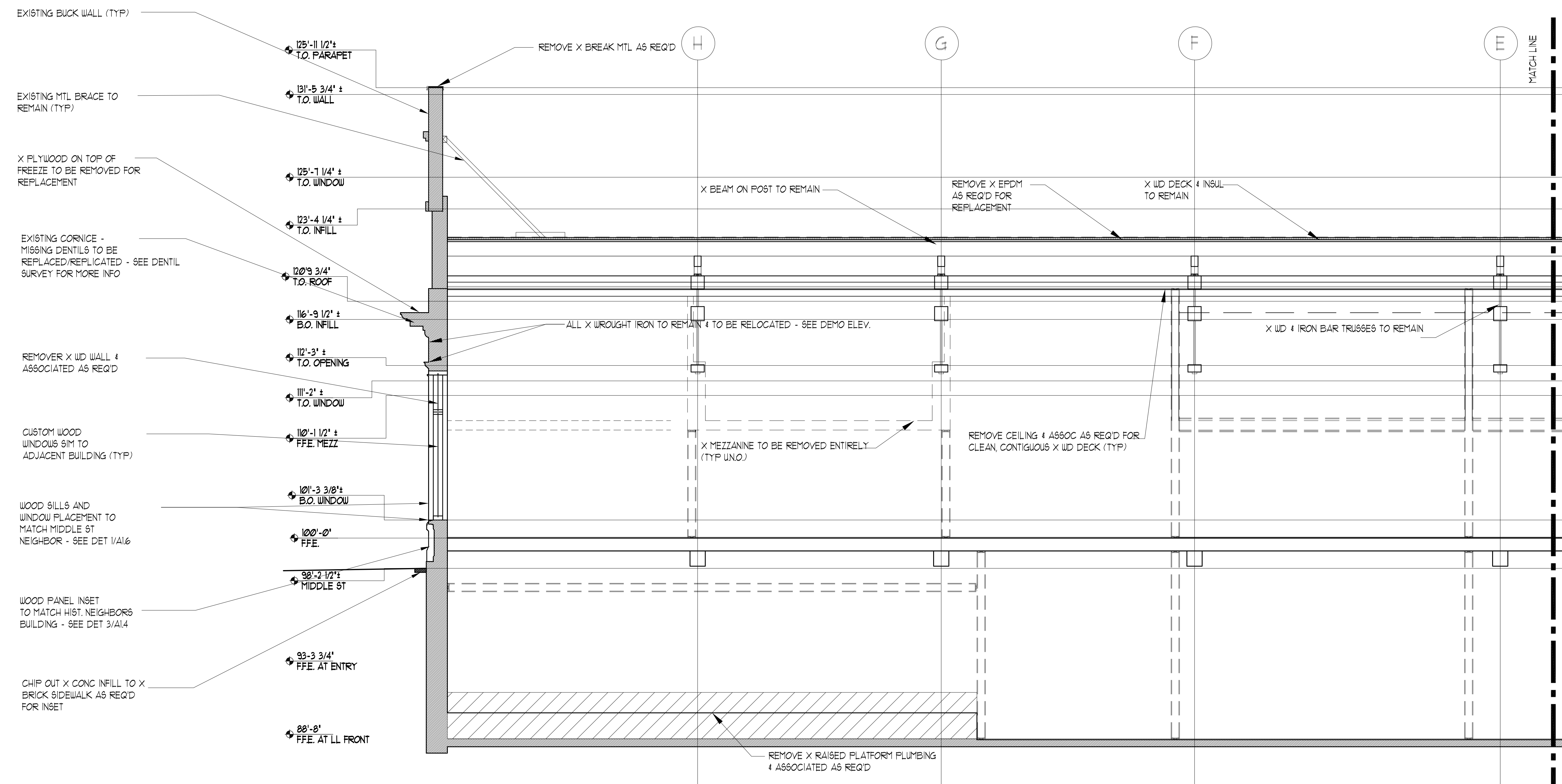
DEMO BUILDING SECTION SCALE: 1/4" = 1'-0"
