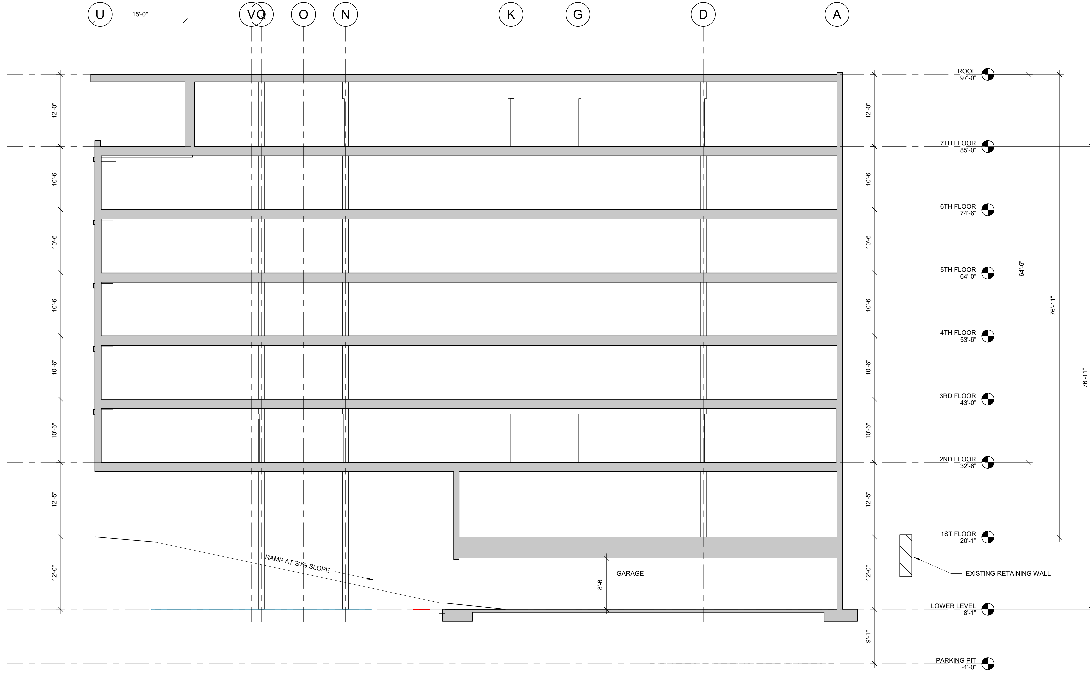
1 SECTION WITH GARAGE 1/8" = 1'-0"
