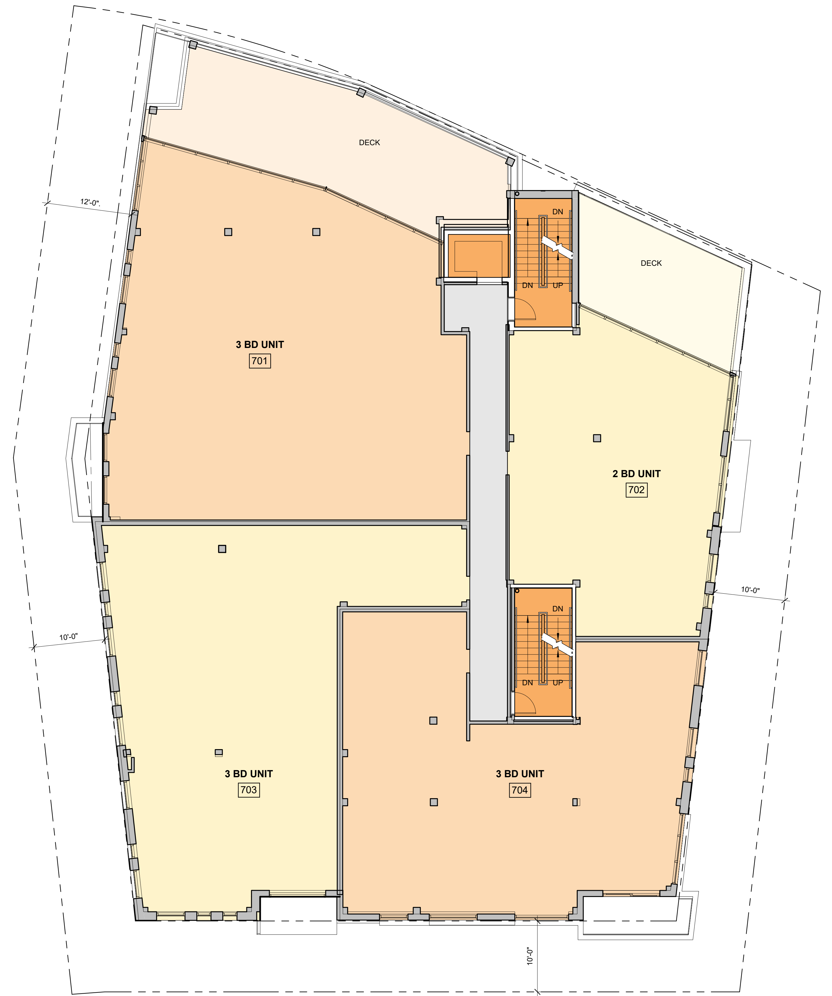
2 | 7TH FLOOR PLAN 1/8" = 1'-0"
