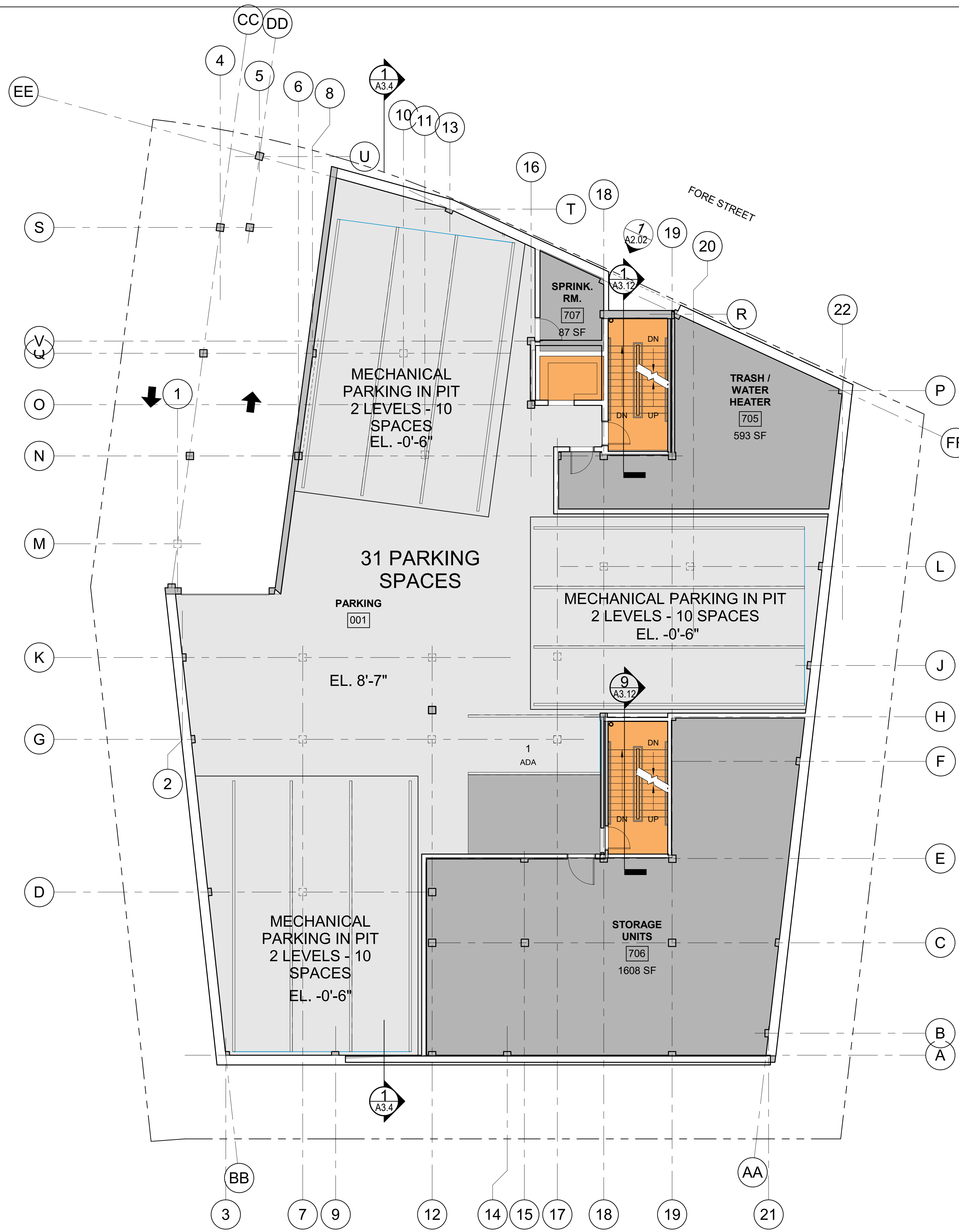
1 LOWER LEVEL 1/8" = 1'-0"
