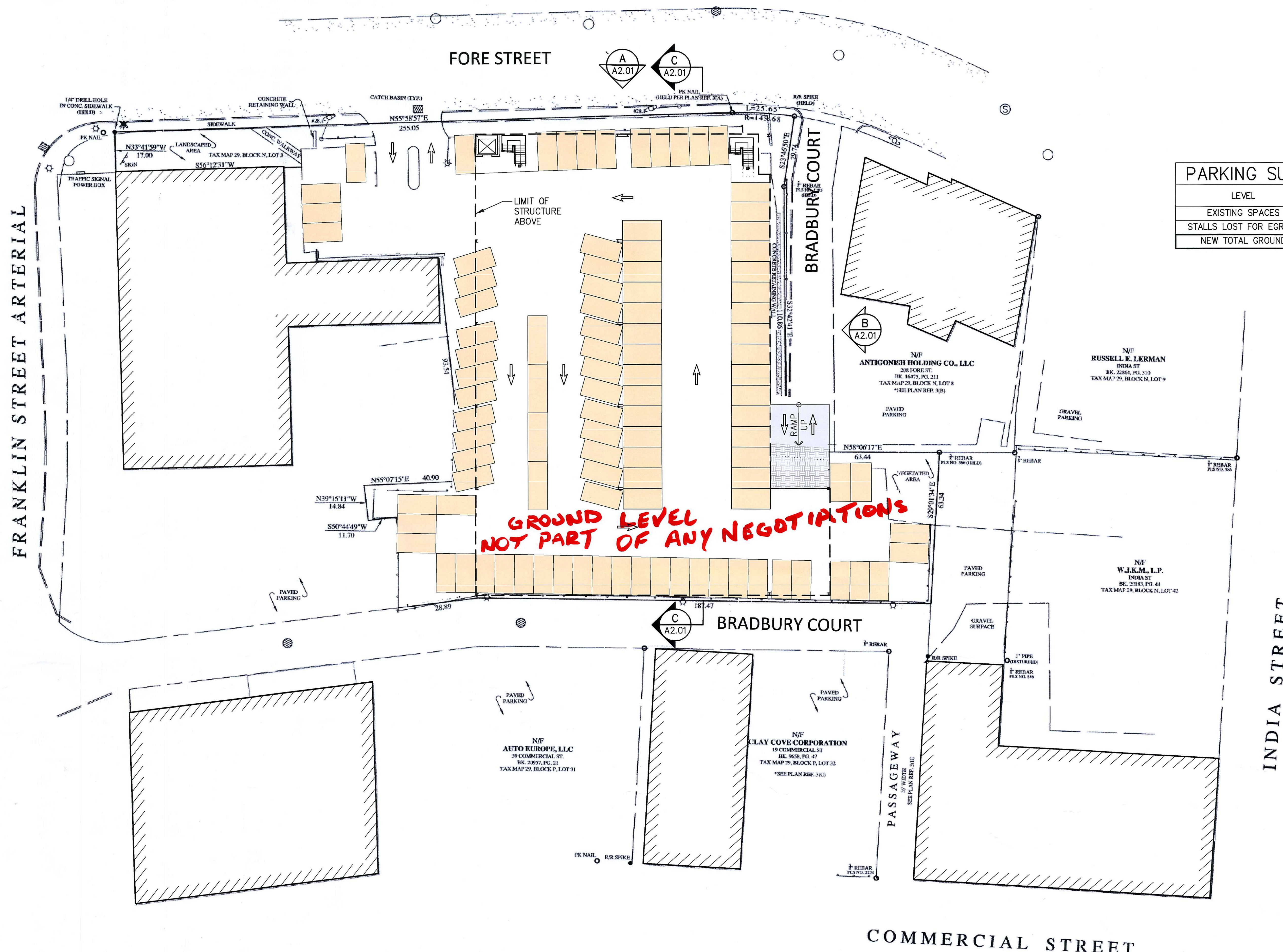
GROUND LEVEL PARKING PLAN 1"=20'-0"
