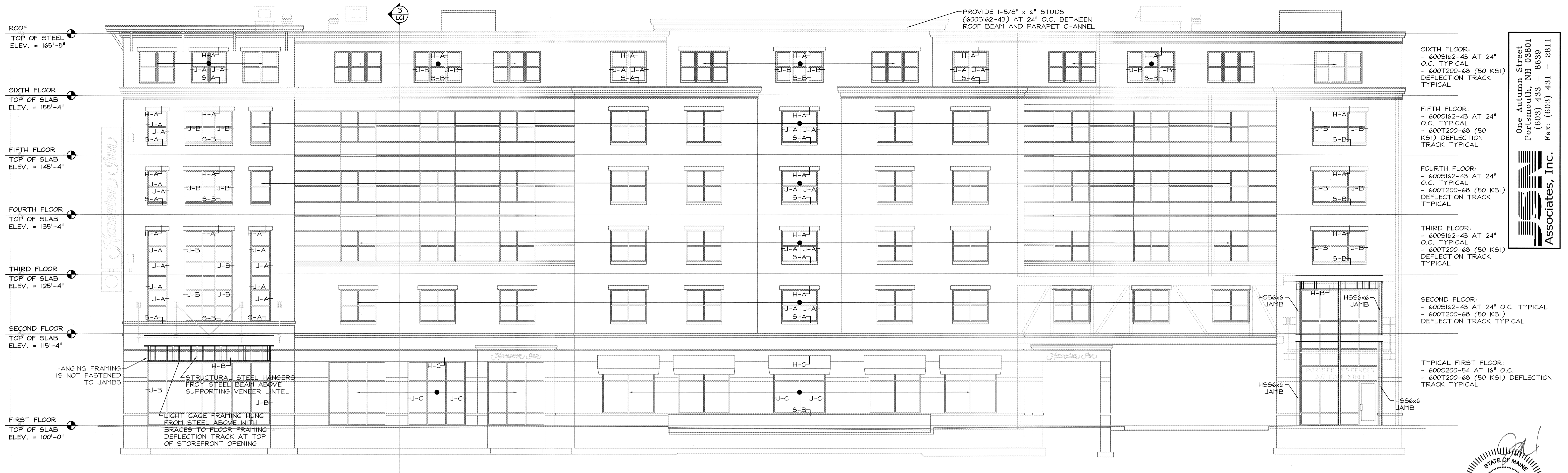
1 SOUTH (FRONT) ELEVATION Scale: 1/8" = 1'
