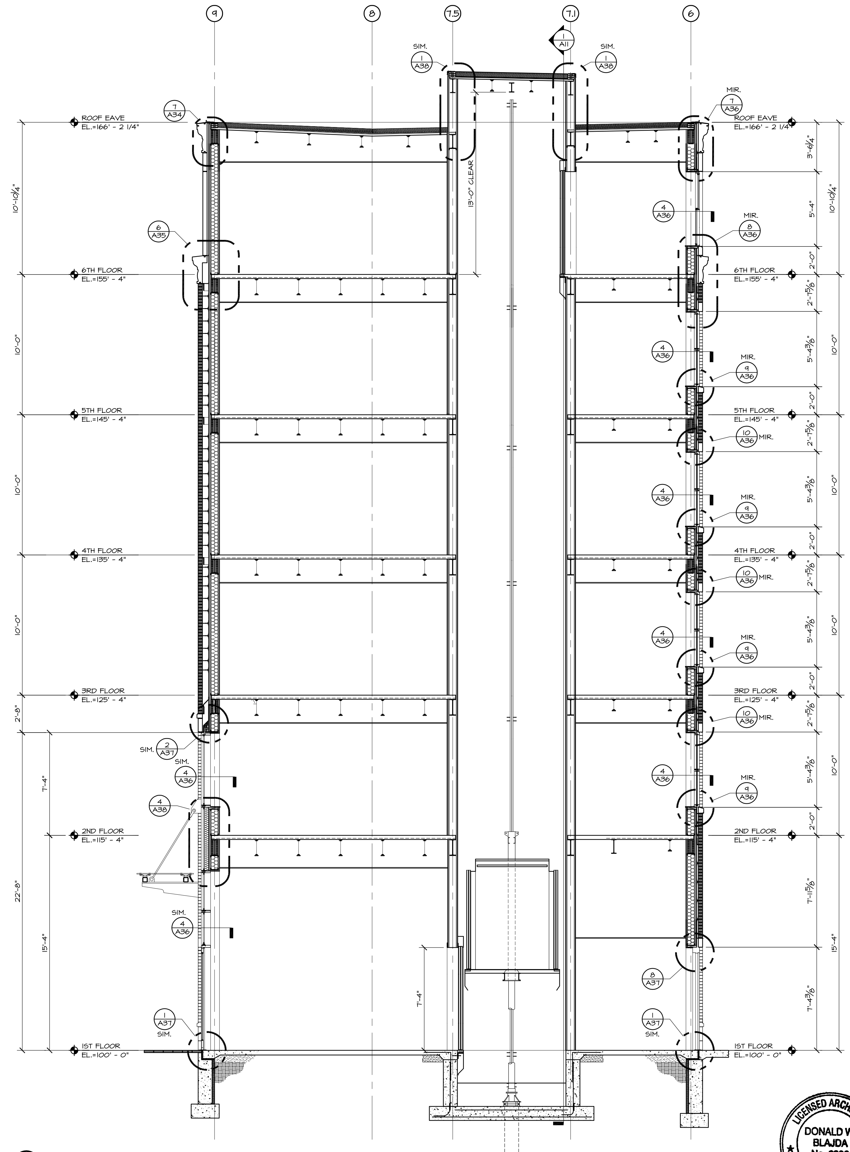
1 ELEVATOR & LOBBY SECTION 1/4" = 1'-0"
