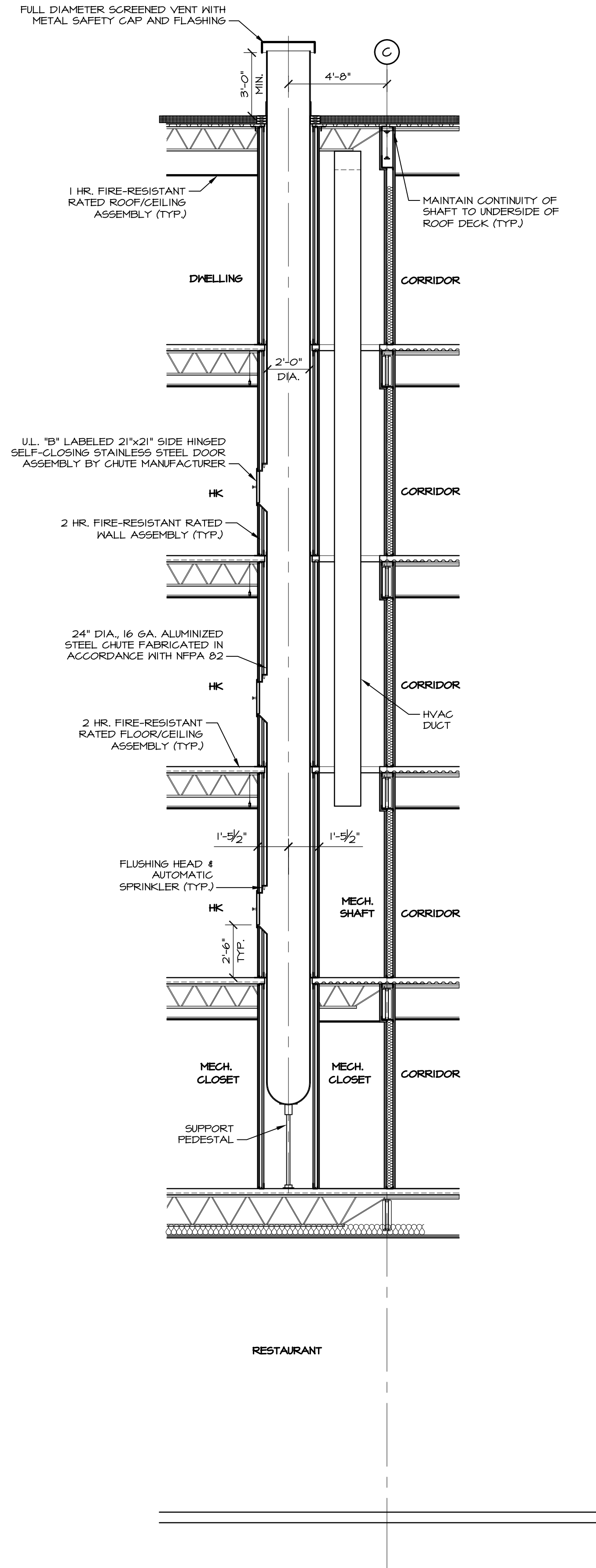
2 LINEN CHUTE SECTION 1/4" = 1'-0"
