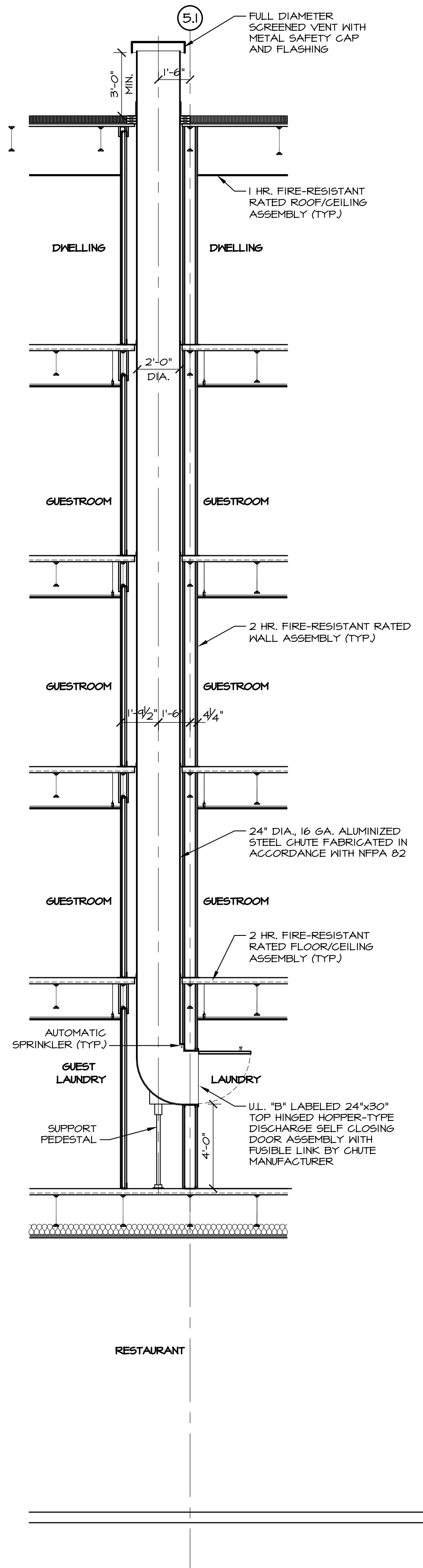
3 LINEN CHUTE SECTION 1/4" = 1'-0"
