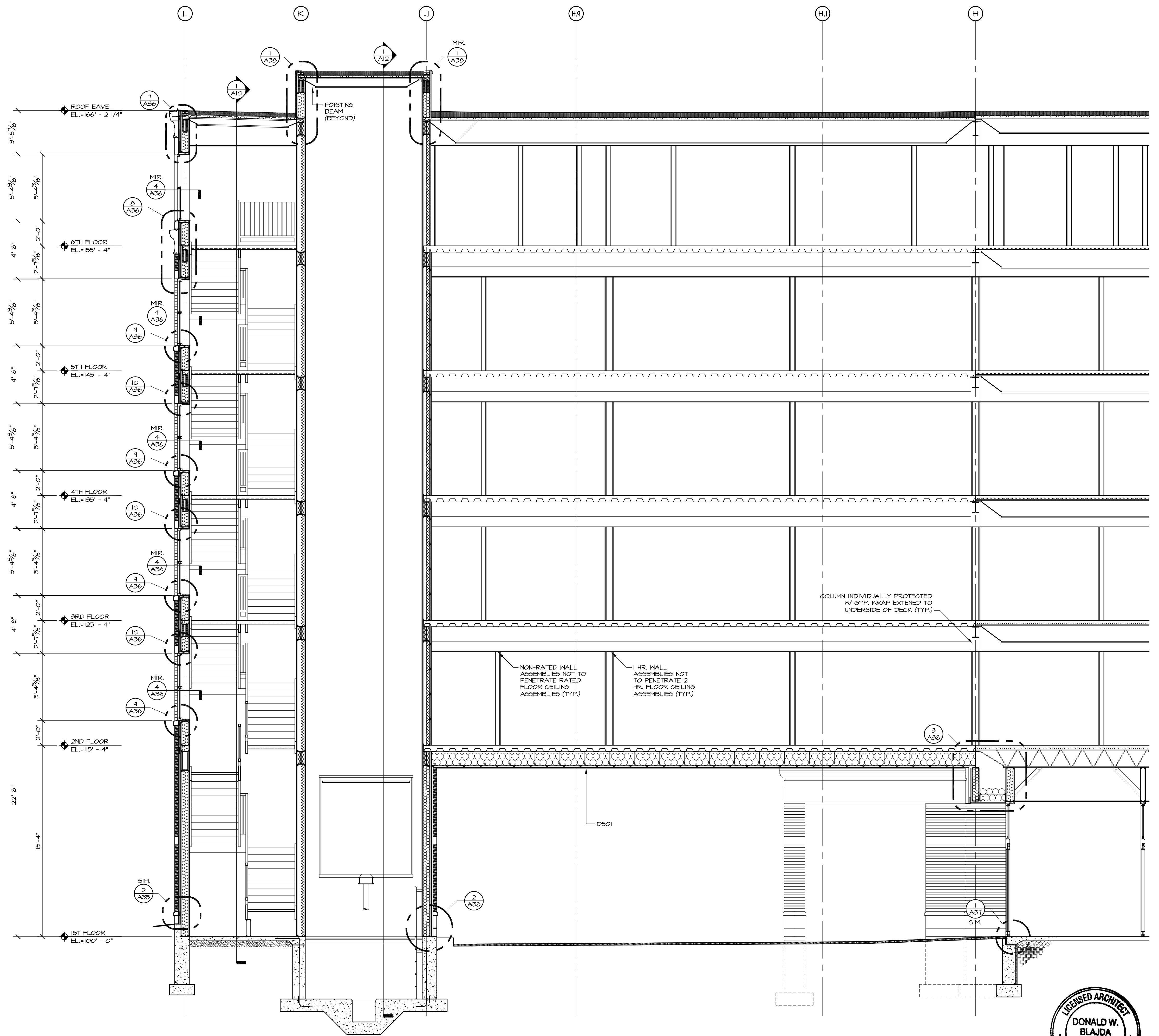
1 STAIR 1 & ELEVATOR SECTION 1/4" = 1'-0"
