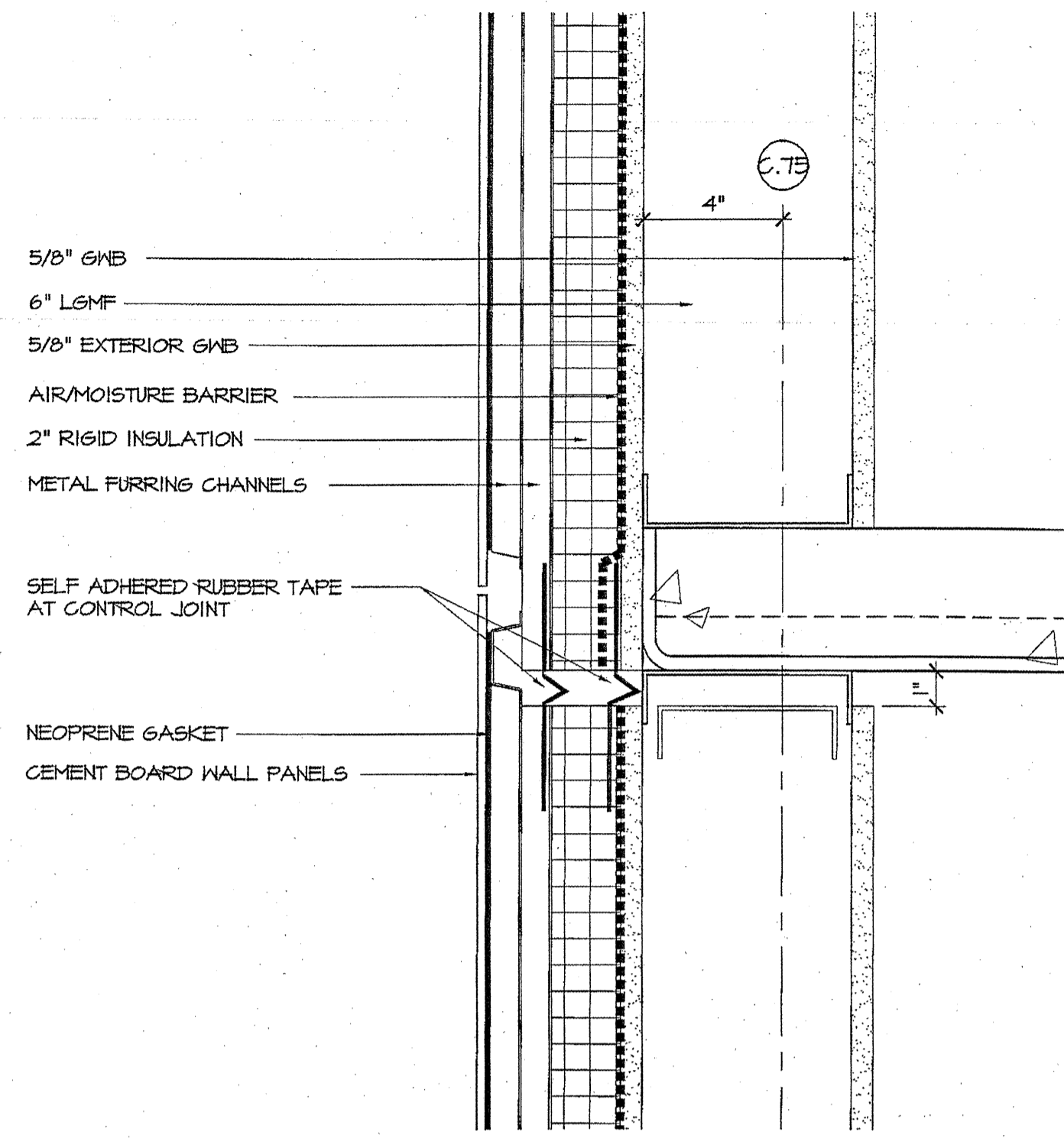
1 SECTION DETAIL - FIFTH FLOOR SCALE: 3" = 1'-0"
