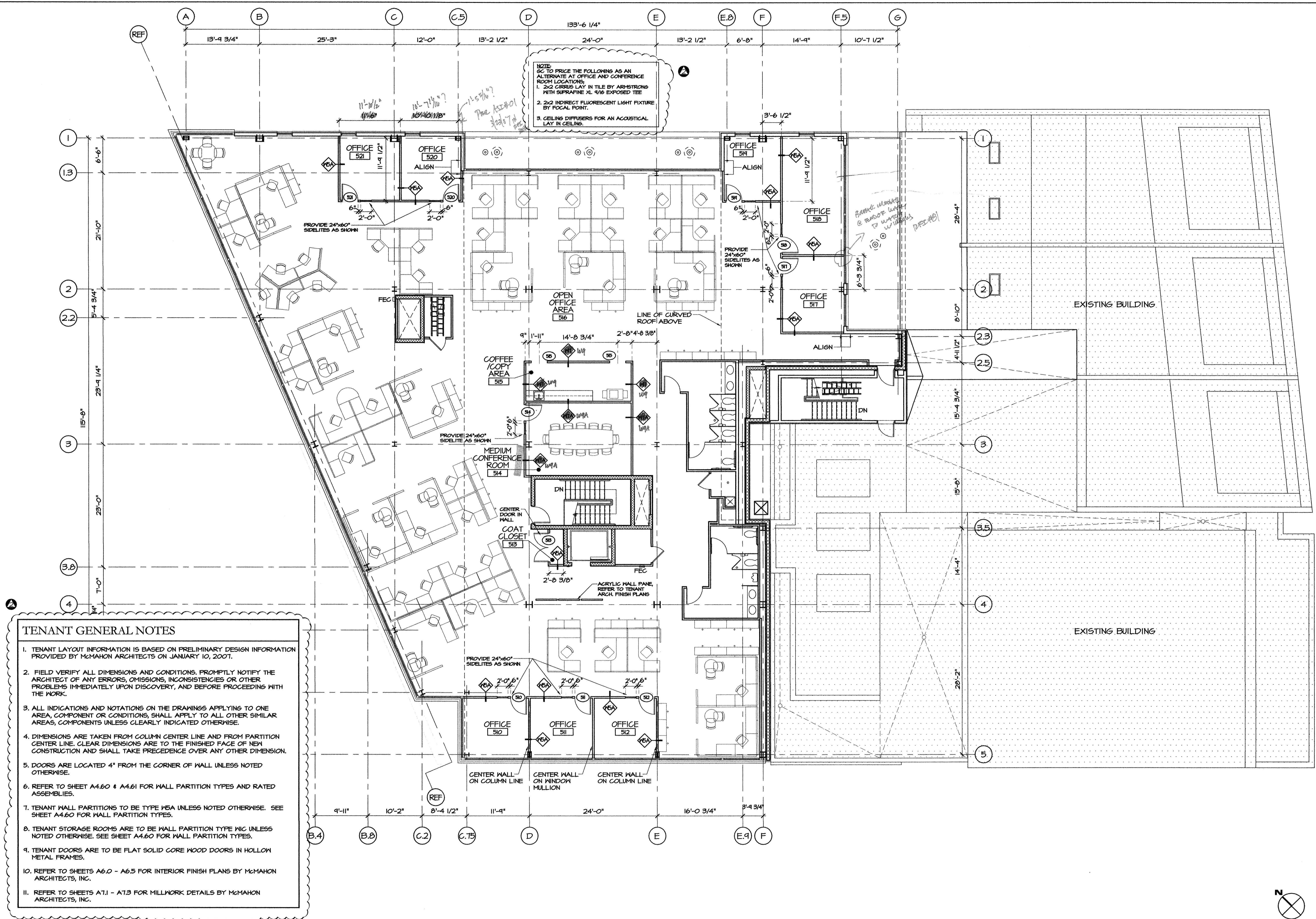
FIFTH FLOOR TENANT FIT-UP PLAN SCALE: 1/8" = 1'-0"
