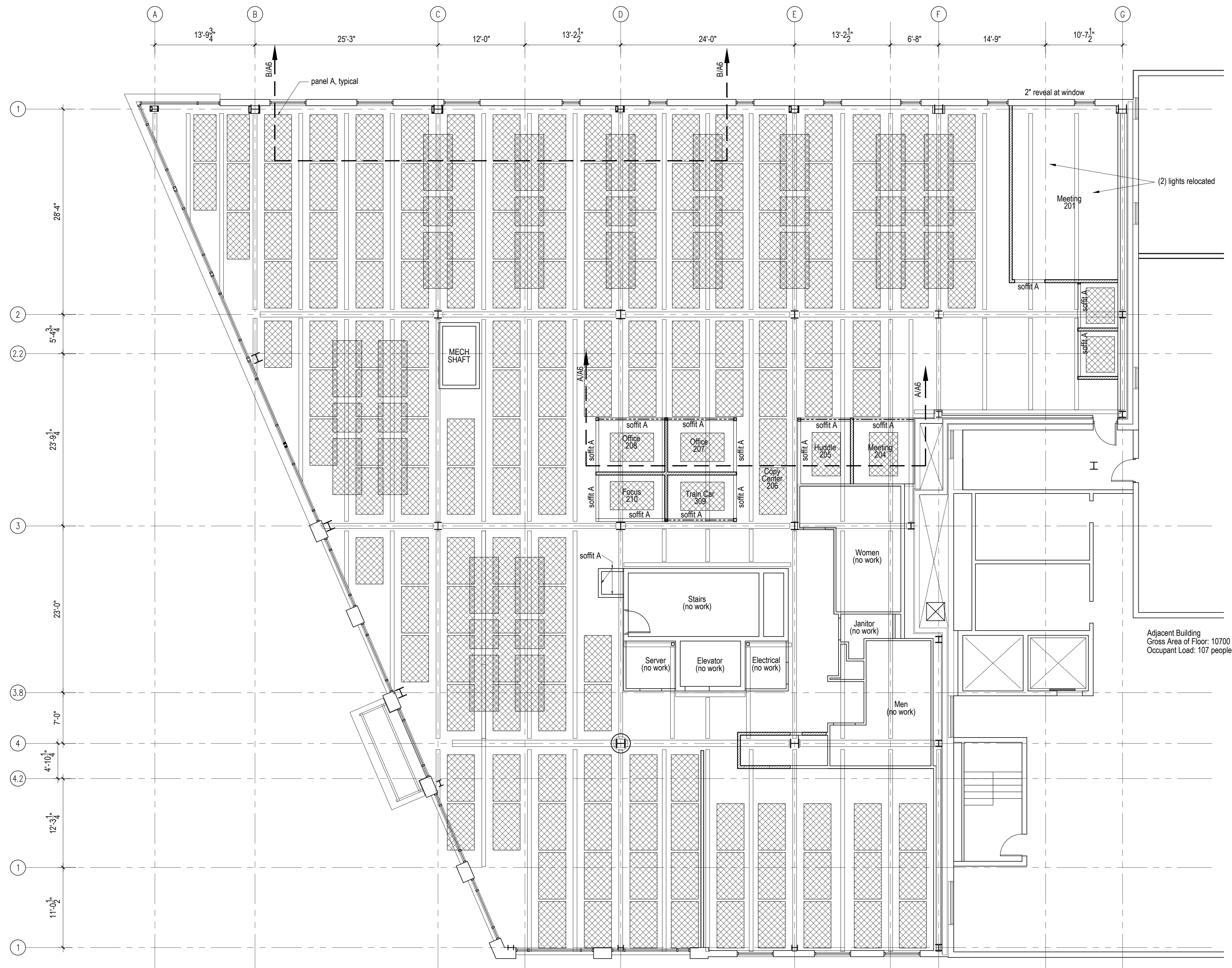
2nd Floor Acoustic Panel Ceiling Plan
